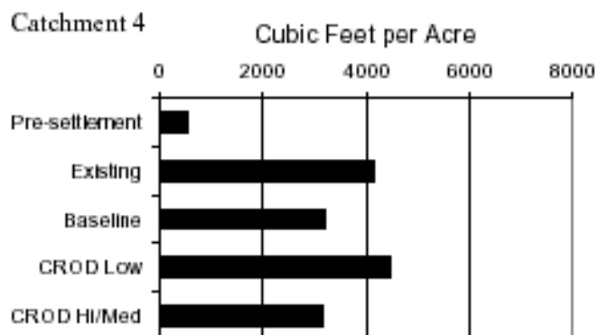
Graph 12.5 Cottage Grove Hydrology Comparison: Cubic Feet of Runoff per Acre for a 10-Year Storm Event
