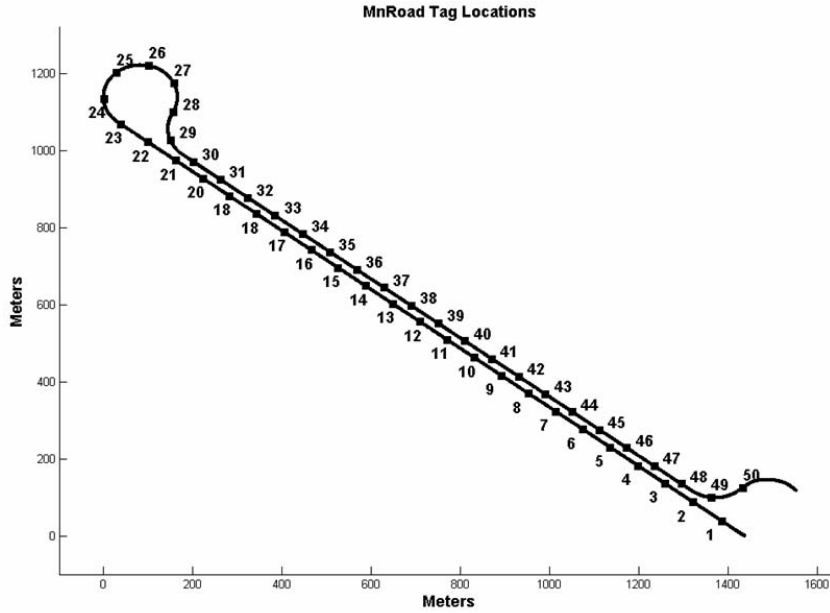
Figure 3.4: RFID tag locations at Mn/ROAD.
