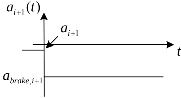
Figure 5.3: Acceleration of lead vehicle (vehicle i+1).
