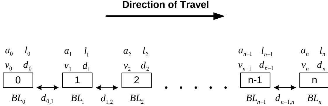
Figure 5.1: A platoon of vehicles showing the data that will be available for risk metric computation.
