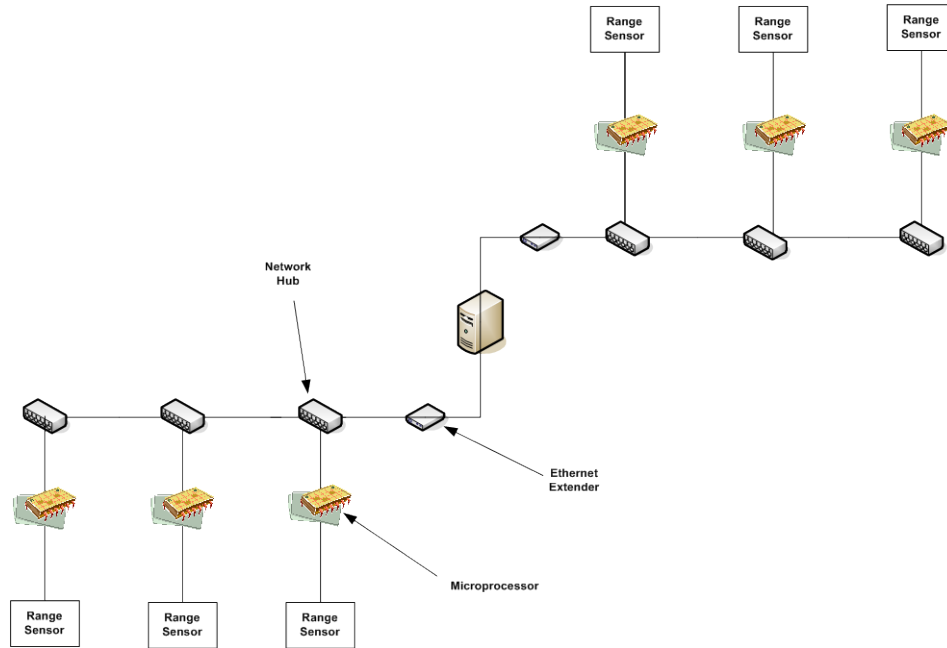
Figure 7: Minimal sensor surveillance system network topology. Daisy chained to reduce construction costs. Ethernet extenders (long distance) and Ethernet hubs (short distance) are employed for network connectivity to the central server. Microprocessors are used to interface with range sensor hardware.
