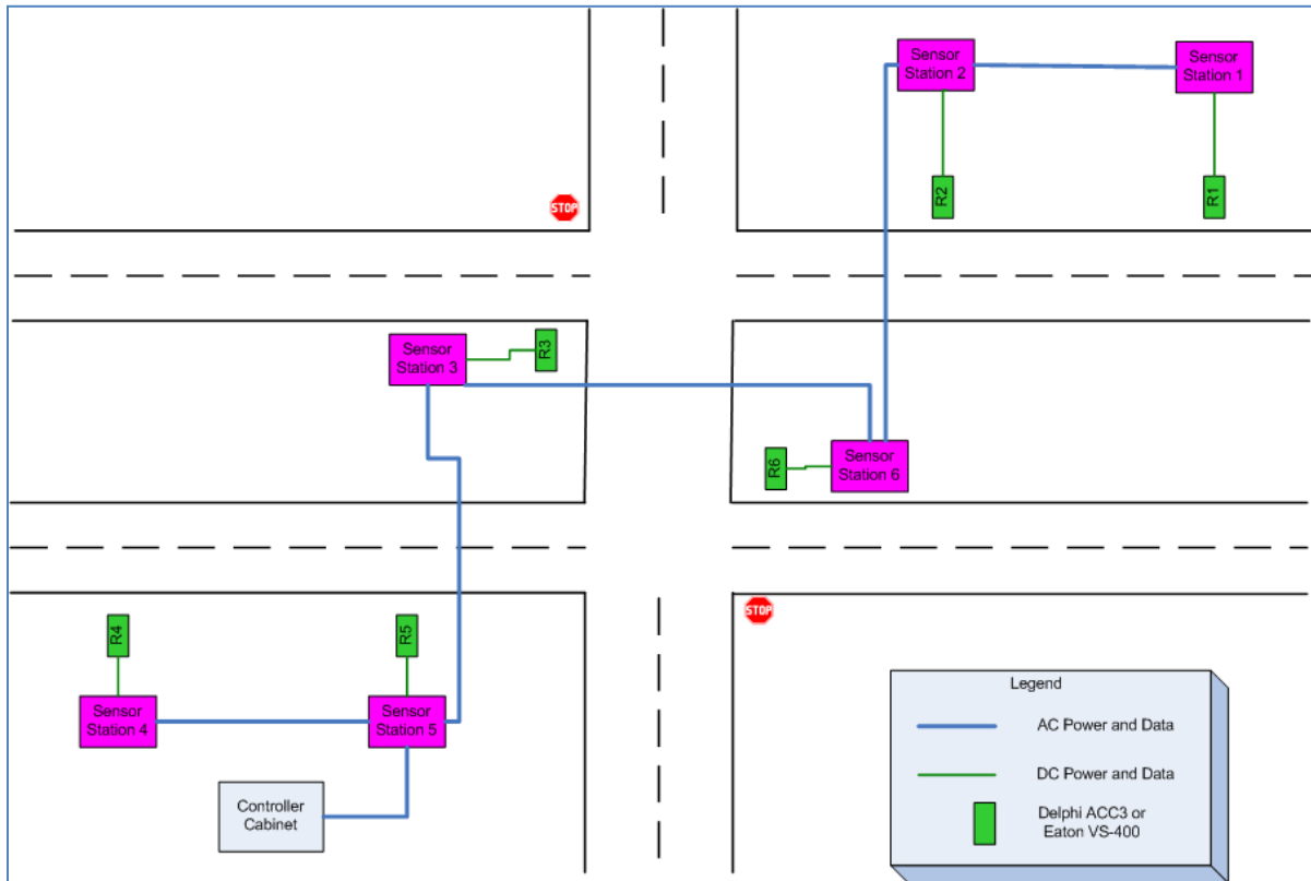
Figure 9: Proposed minimal sensor surveillance system hardware layout for rural four lane expressway thru-stop intersections with Delphi ACC3/Eaton VS-400 radar
