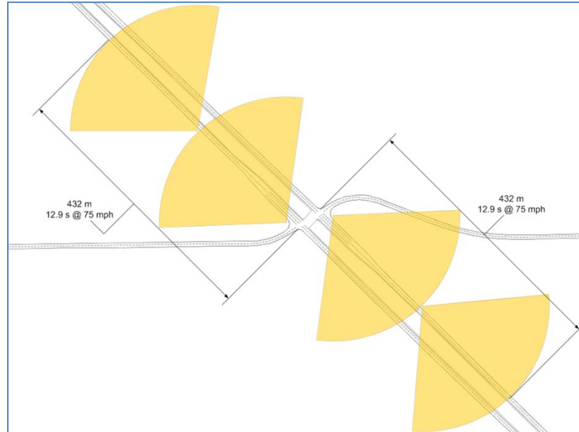
Figure 12: Minimal sensor suite layout required for mainline surveillance system on rural four lane expressway thru-stop intersections using specifications for Ibeo Lux sensor
