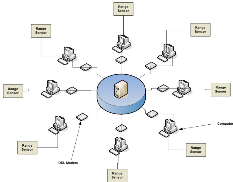
Figure 6: Network topology of Hwy 52 intersection. A star topology was chosen for robustness. DSL modems facilitated long range network connection between central server and computer stations.
