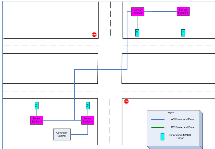
Figure 17: Proposed minimal sensor surveillance system hardware layout using Smartmicro UMRR radar
