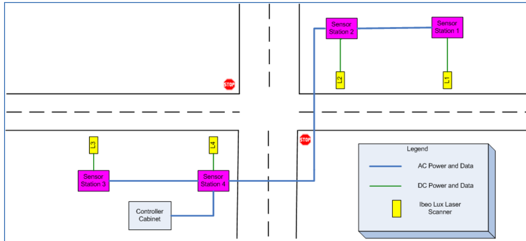
Figure 15: Proposed minimal sensor surveillance system hardware layout for rural two lane highway thru-stop intersections with Ibeo Lux Sensor
