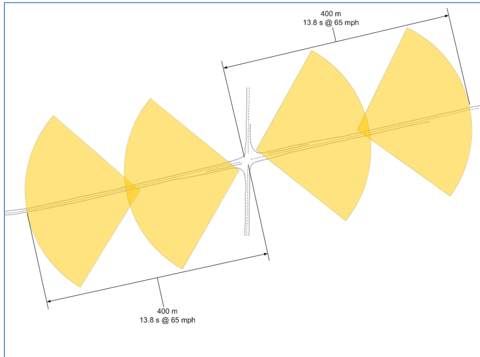
Figure 14: Minimal sensor suite layout required for mainline surveillance system on rural two lane highway thru-stop intersection using specifications for Ibeo Lux Sensor
