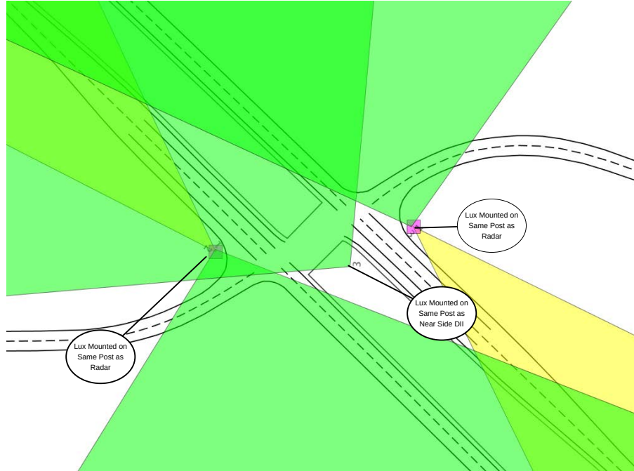
Figure 24: Proposed minor road vehicle presence detection sensor layout using Ibeo Lux, mounted on already existing posts, at rural four lane expressway thru-stop intersection. The field of view of the Lux is shown in green.
