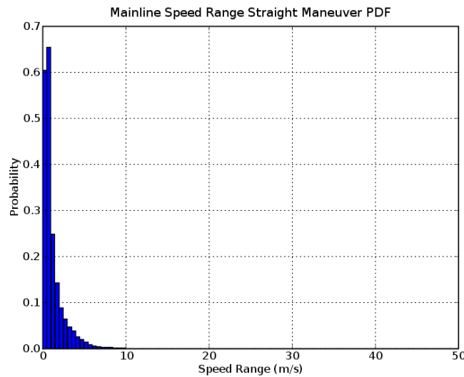
Figure 5: Probability Density Function of the range of speed of vehicles traveling on the mainline (US 52) that went straight through the intersection
