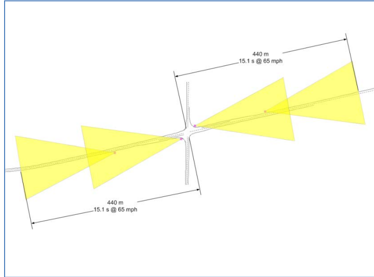
Figure 18: Minimal sensor suite layout required for mainline surveillance system on rural two lane highway thru-stop intersection using specifications for Smartmicro UMRR radar
