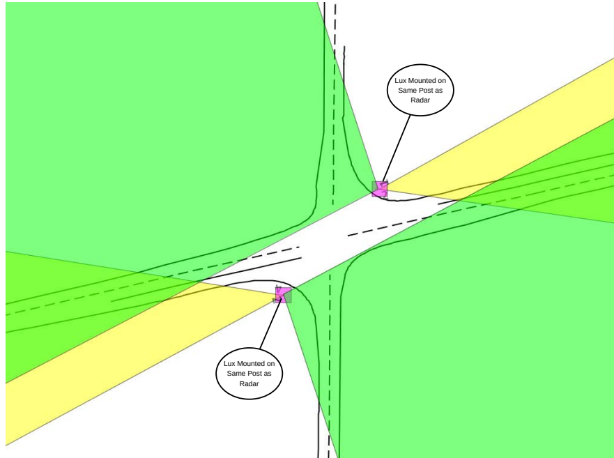
Figure 25: Proposed minor road vehicle presence detection sensor layout using Ibeo Lux, mounted on already existing poles, on a rural two lane highway thru-stop intersection. The field of view of the Lux is shown in green.
