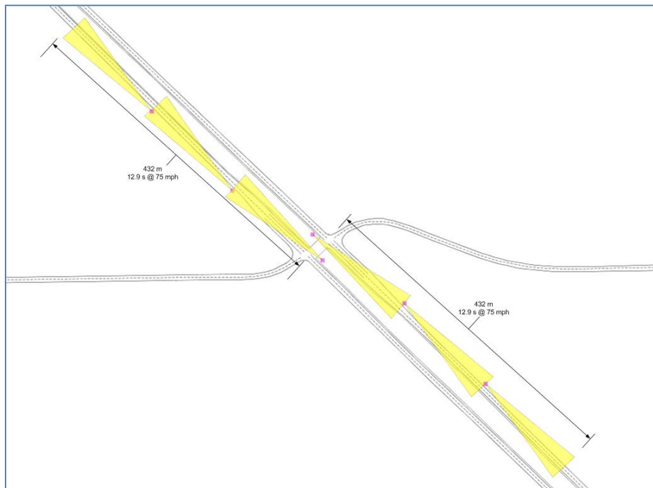
Figure 8: Minimal sensor suite layout required for mainline surveillance system on rural four lane expressway thru-stop intersections using specifications for Delphi ACC3/Eaton VS-400 radar
