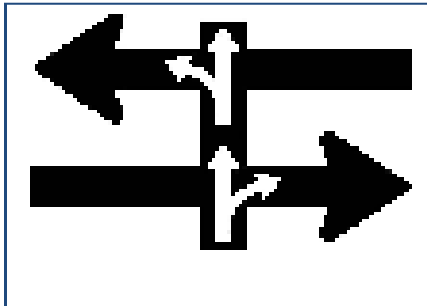
Figure 20: Bitmap representing the default DII state (no vehicles on mainline)
