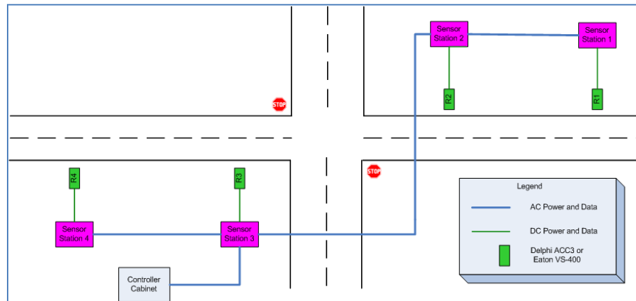
Figure 11: Proposed minimal sensor surveillance system hardware layout for two lane roads with Delphi ACC3/Eaton VS-400 radar
