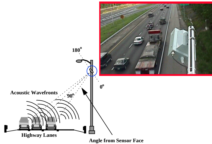
Figure 3: The SAS-1 sensor mounted in a side fire configuration can detect multiple lanes
