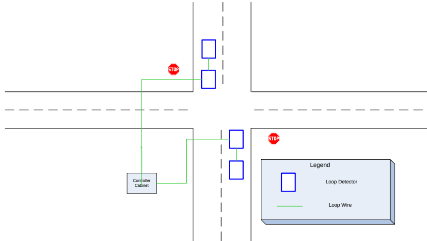
Figure 23: Hardware layout of proposed inductive loop installation on rural two lane highway thru-stop intersection
