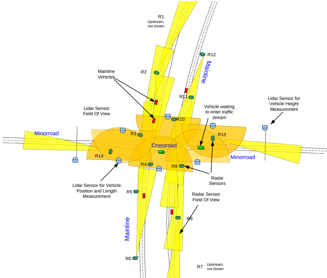
Figure 1: Plan view of a typical instrumented rural four lane expressway intersection. Sensors are radar (yellow triangles indicate field of view and) scanning lidar (orange semicircles); all data is sent from sensor processors to the main central processor.
