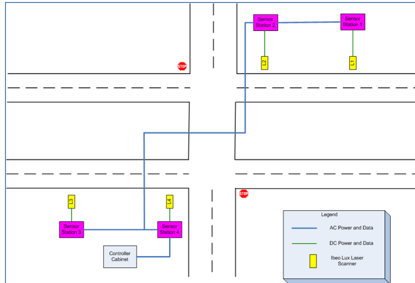
Figure 13: Proposed minimal sensor surveillance system hardware layout for rural four lane expressway thru-stop intersections using Ibeo Lux laser scanners
