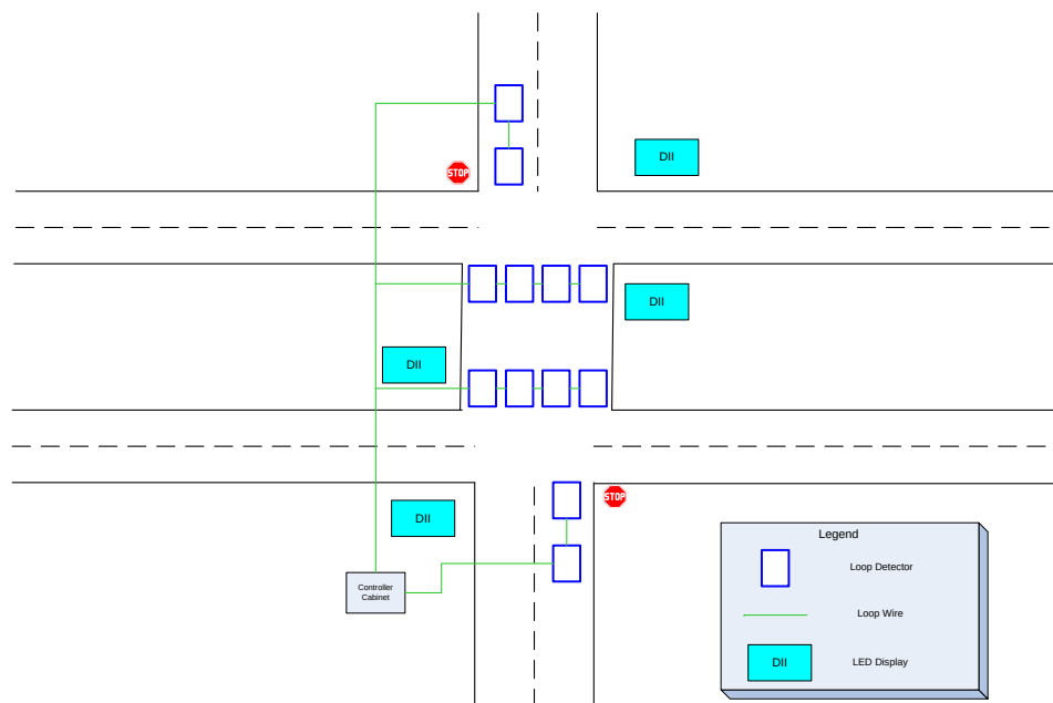
Figure 22: Hardware layout of proposed inductive loop installation of a rural four lane expressway thru-stop intersection
