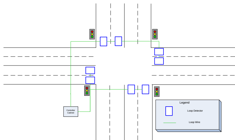
Figure 21: Hardware layout of inductive loop installation of a four leg intersection, two lanes per approach
