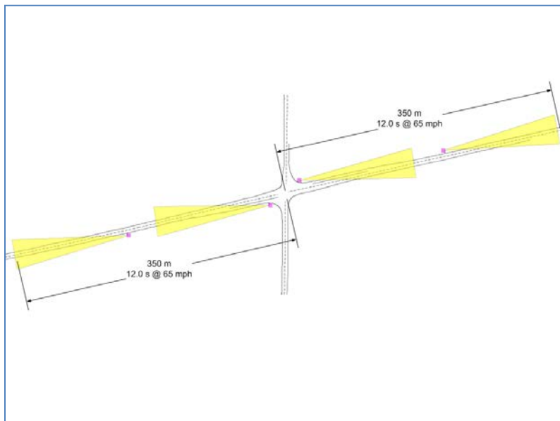
Figure 10: Minimal sensor suite layout required for mainline surveillance system on rural 2 lane highway thru-stop intersection using specifications for Delphi ACC3/Eaton VS-400 radar
