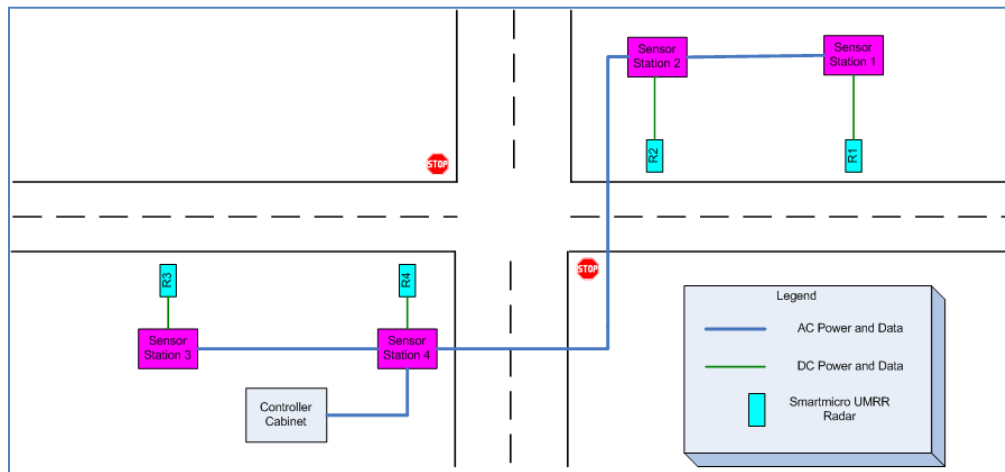
Figure 19: Proposed minimal sensor surveillance system hardware layout for rural two lane highway thru-stop intersection with Smartmicro UMRR radar
