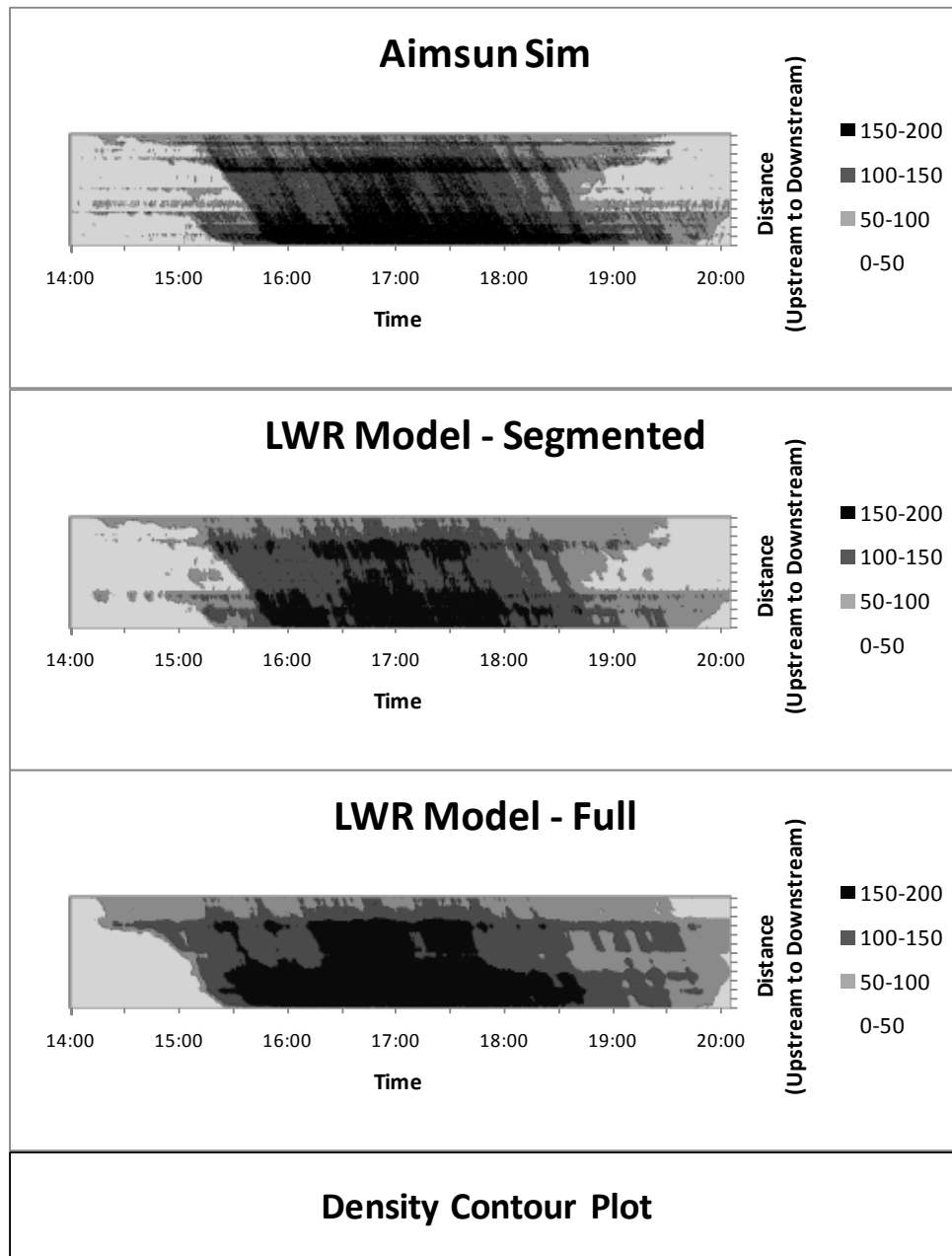
Figure 3-9: Density contour plots comparing AIMSUN vs. traditional LWR vs. segmented LWR
