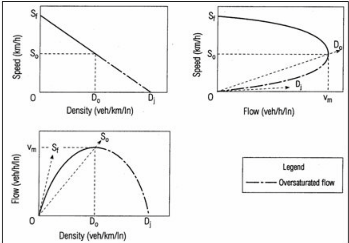
Figure 2-1: Graphs showing relationships between traffic state parameters
