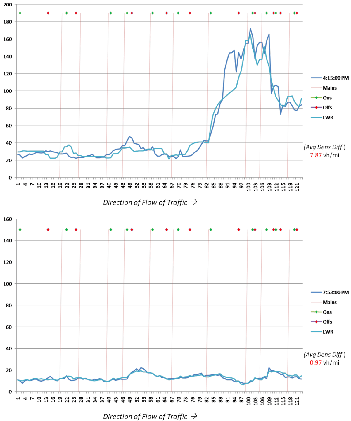
Figure 3-8: Sample density profile plots against space comparing the segmented LWR to AIMSUN
