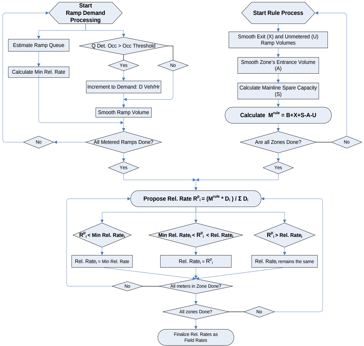
Figure 4-2: Structure of the Stratified Zone Metering algorithm (source: [27])
