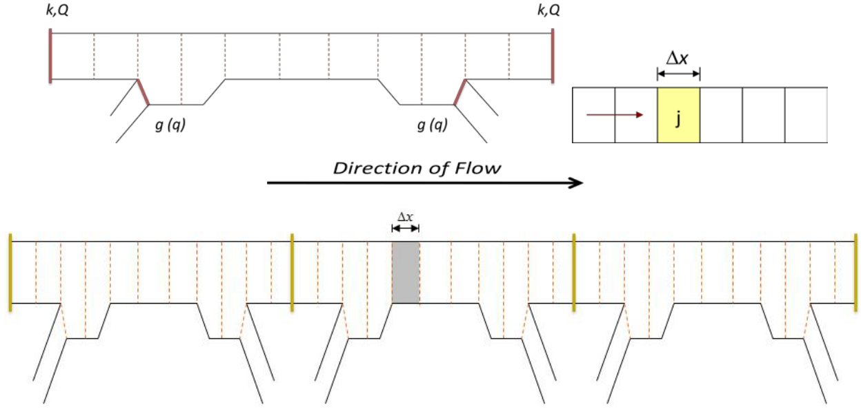
Figure 3-2: Application of the LWR model to a section of the freeway
