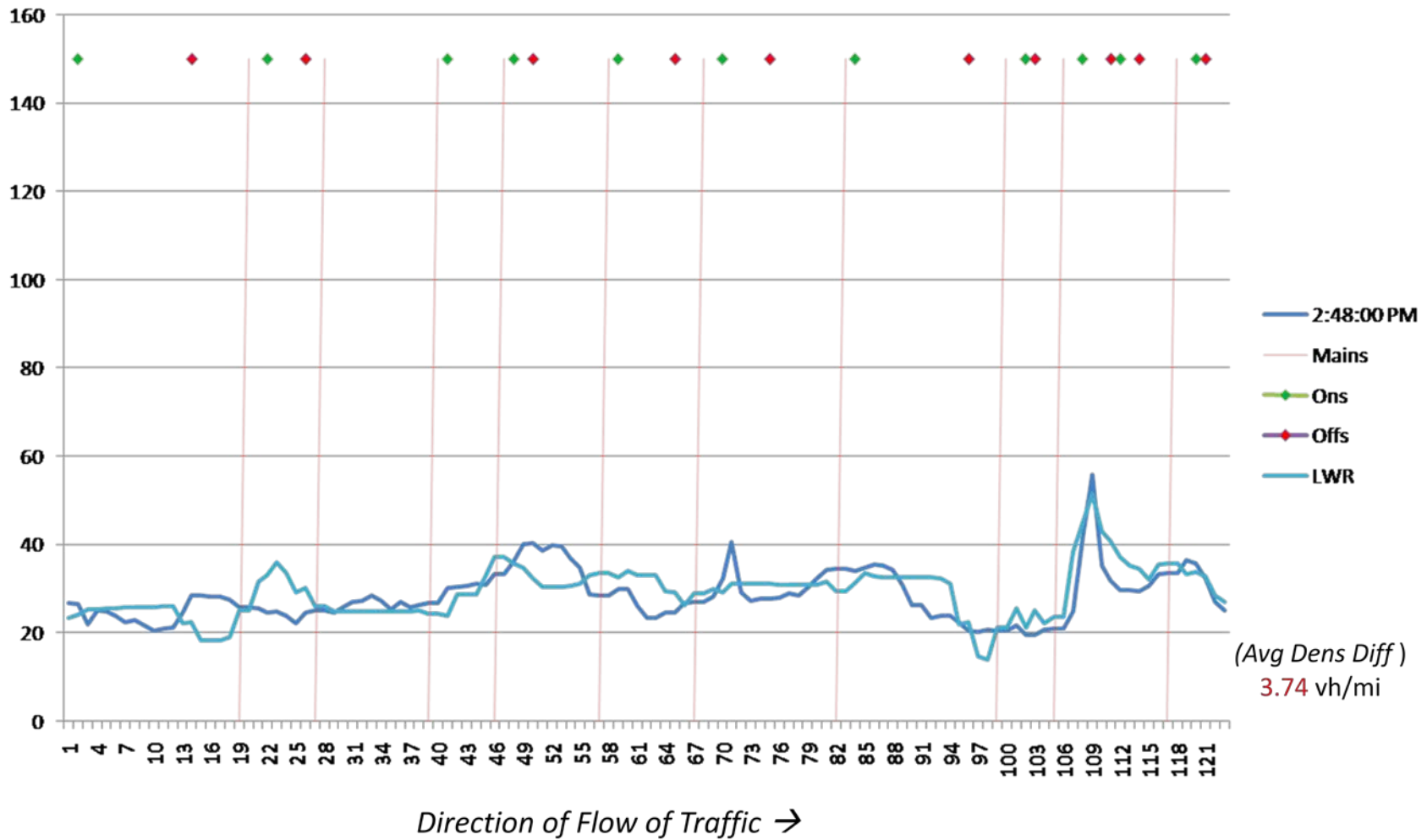
Figure 3-5: Density profile showing AIMSUN reported density vs. LWR predicted density against distance during an off-peak instance of time
