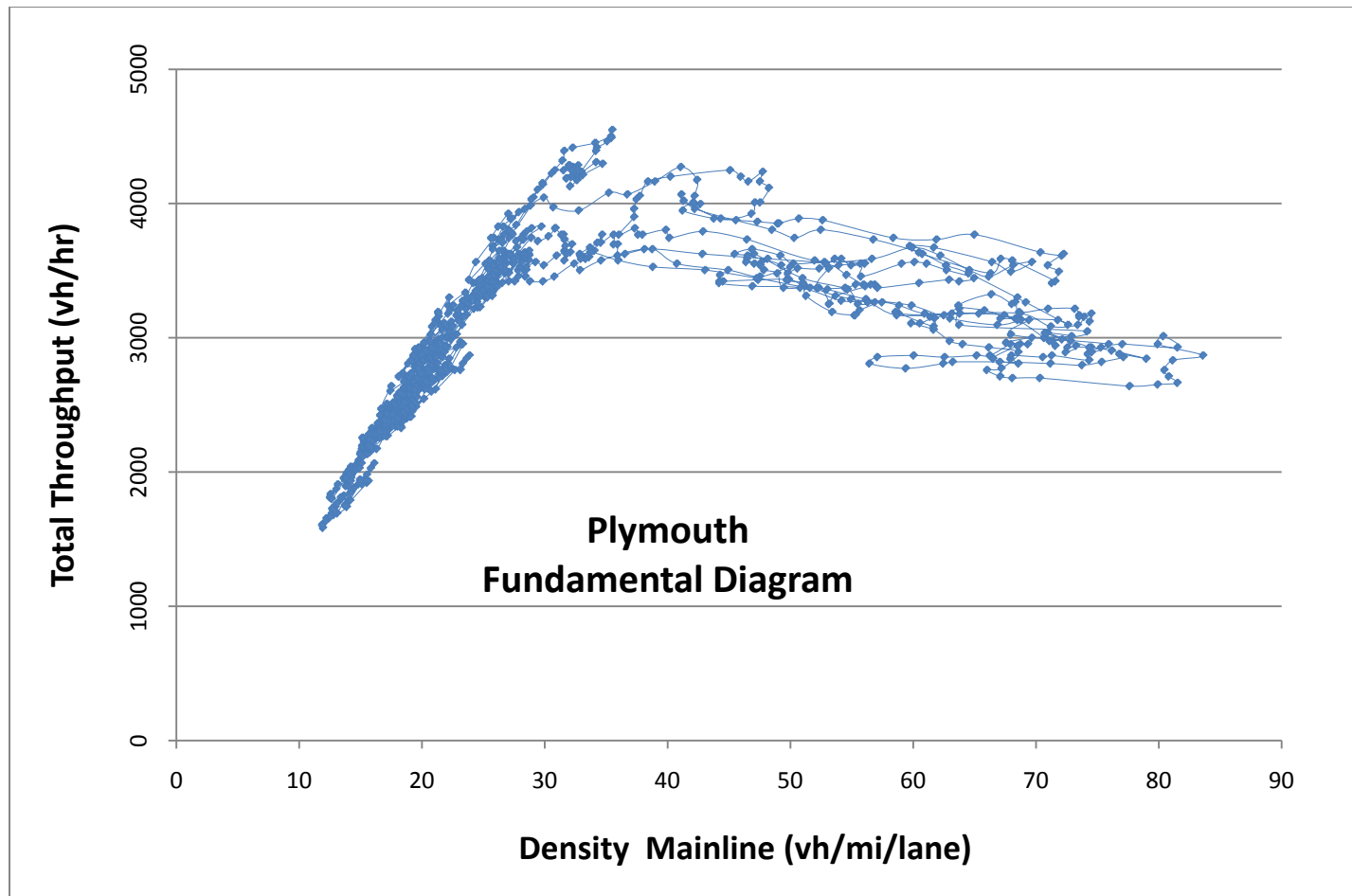
Figure 2-5: Fundamental diagram plot between flow and density at bottleneck
