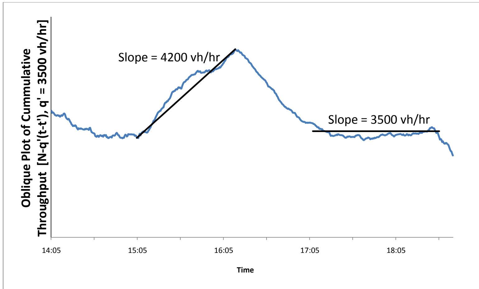
Figure 2-4: Oblique plot of cumulative throughput at bottleneck
