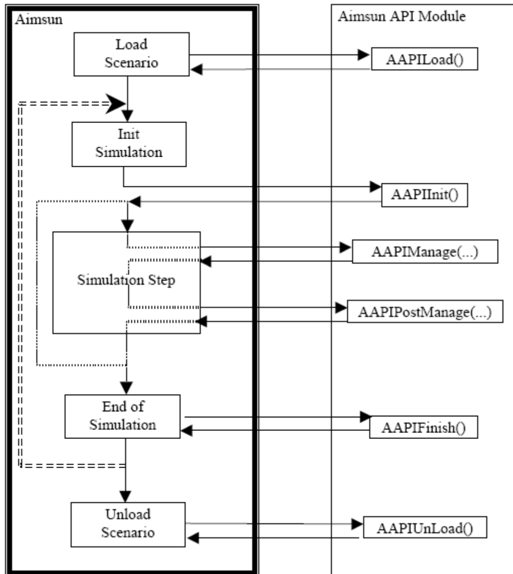
Figure 5-5: AIMSUN and AIMSUN API module interaction scheme (Source: AIMSUN API v6 documentation)
