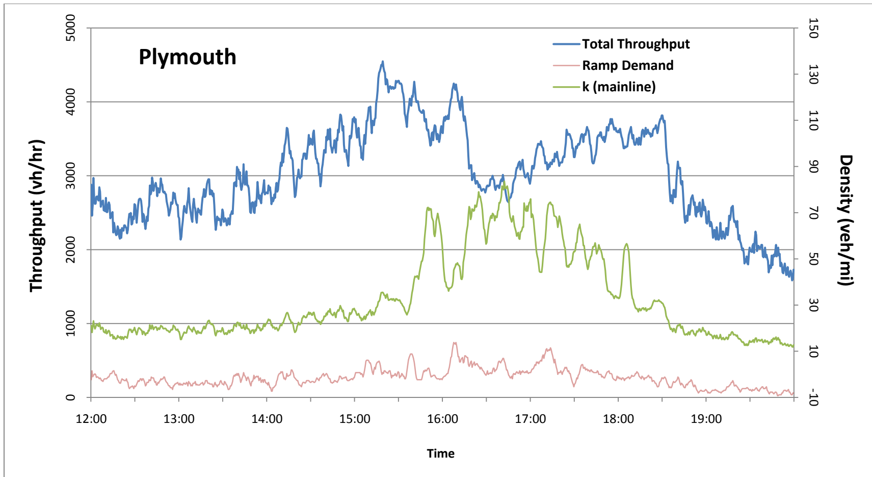
Figure 2-3: Time series plot of throughput at bottleneck (5 min averages)
