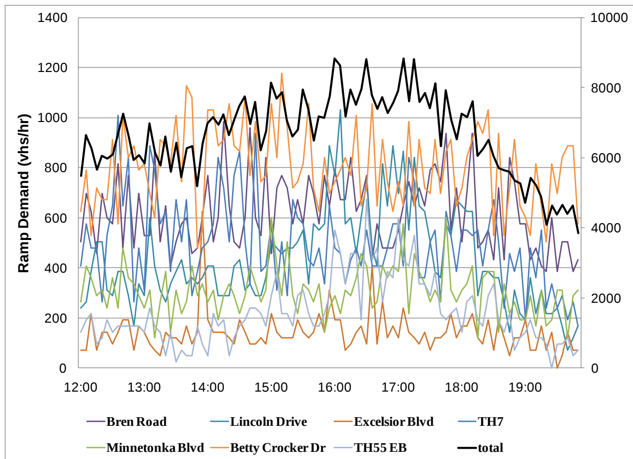
Figure 5-3: On ramp demands for the study site
