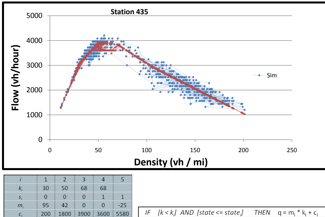
Figure 3-3: Model “5-step” stepwise linear flow - density relation
