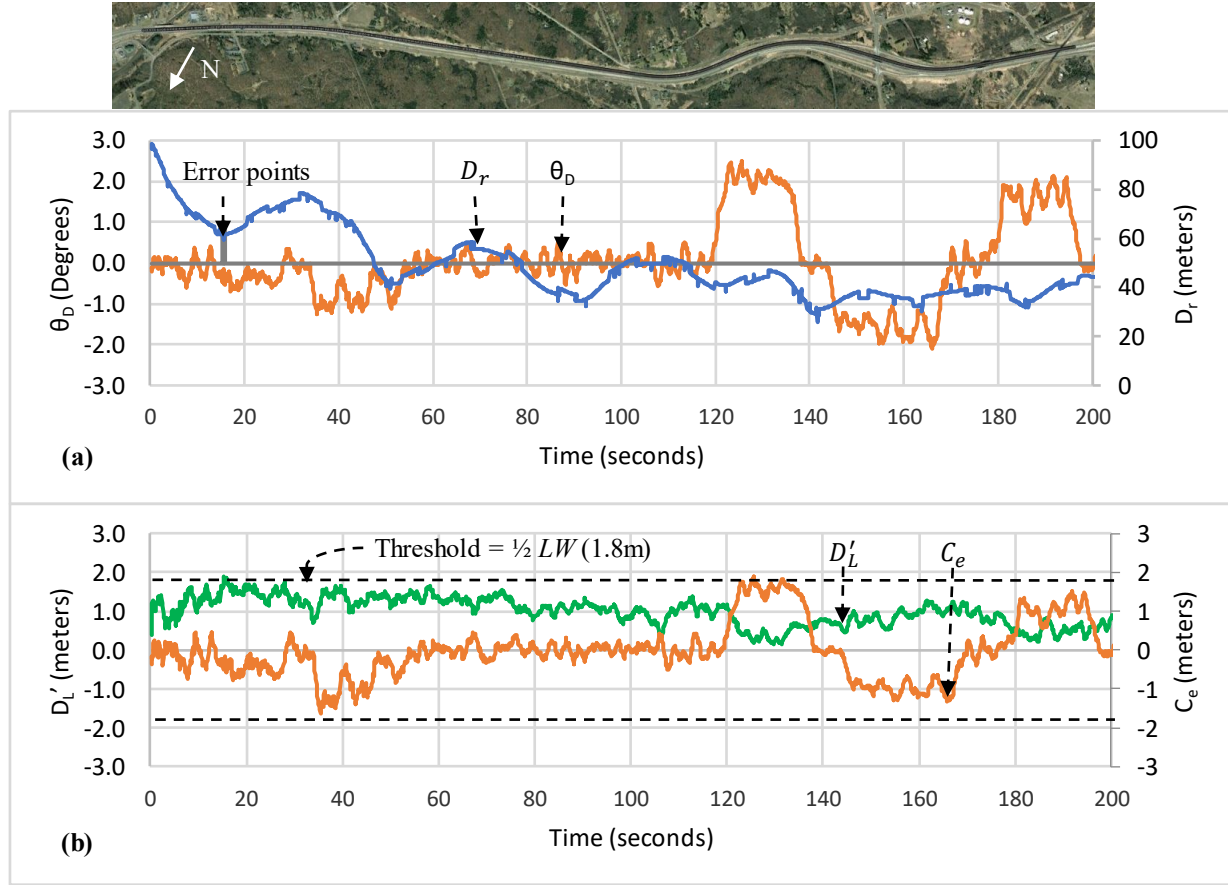
Figure 3.5 (a) \theta_D and D_r vs time and (b) C_e and D'_L vs. time, for field test run #1 where many erroneous lane decisions were observed. The erroneous decisions are shown with grey mask in (a). The corresponding road map of the field test is shown on the top of the figure.
