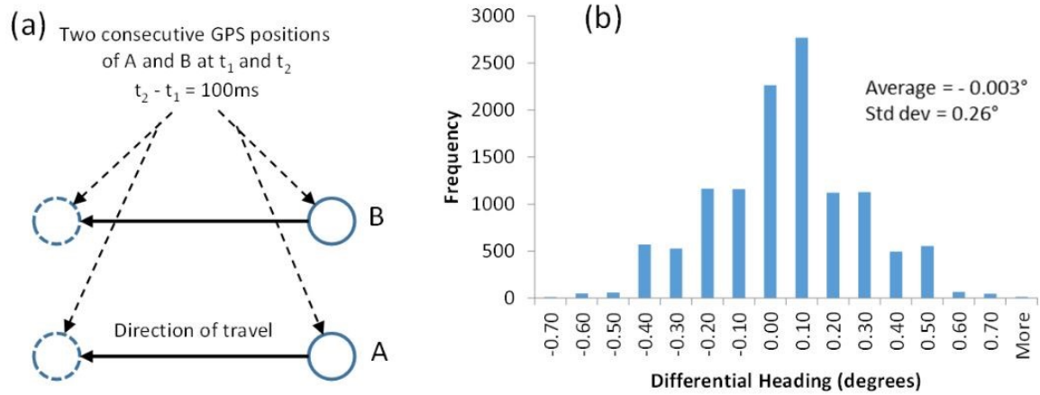
Figure 2.14 (a) The schematic diagram of calculated headings of the two GPS receivers at locations A and B, and (b) the histogram of the differential heading.
