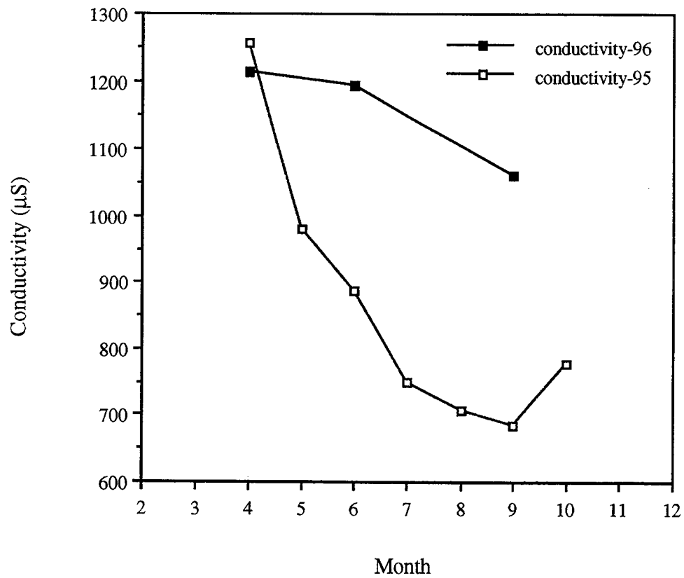
Figure 13. Soil conductivity during the 1995 and 1996 seasons at the Cambridge-Fall field site. Soil samples were collected within 4 m from the pavement edge, to a depth of 10 cm. Each data point represents the mean value from 16 soil samples.
