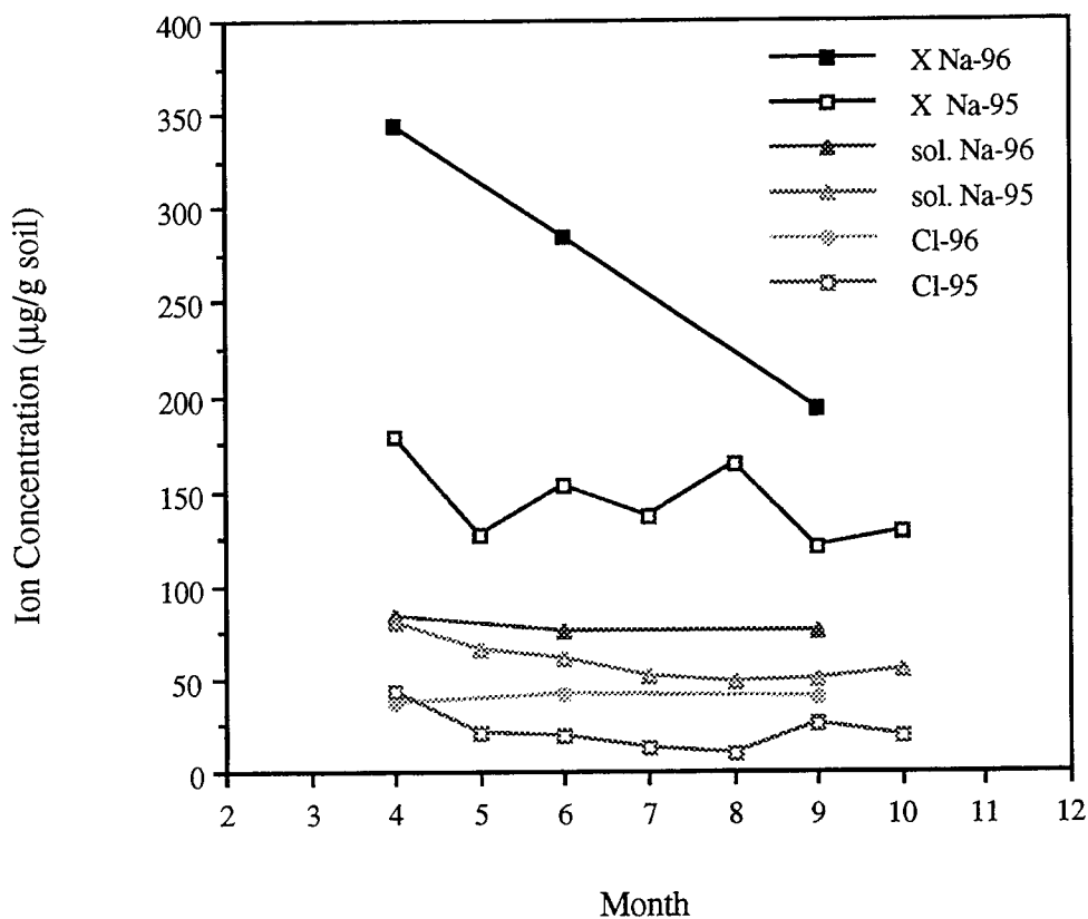
Figure 12. Sodium and chloride concentrations in soil during the 1995 and 1996 seasons at the Cambridge-Fall field site. Soil samples were collected within 4 m from the pavement edge, to a depth of 10 cm. Each data point represents the mean value from 16 soil samples. "X Na", "sol. Na" refer to exchangeable sodium and soluble sodium, respectively.
