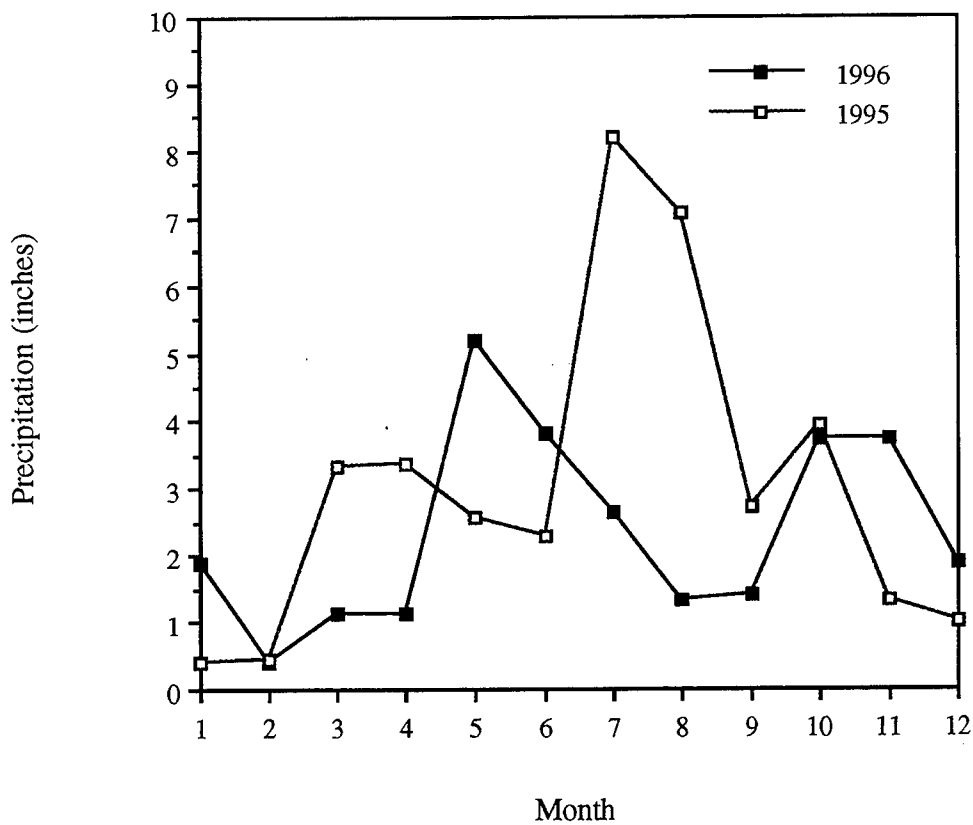
Figure 15. Precipitation totals for Cambridge, MN during the 1995 and 1996 seasons. The data was obtained from The State Climatology Office, Division of Waters, Minnesota Department of Natural Resources.
