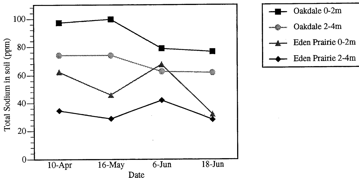
Figure 6. Total sodium in soils at each field site, 1996.
