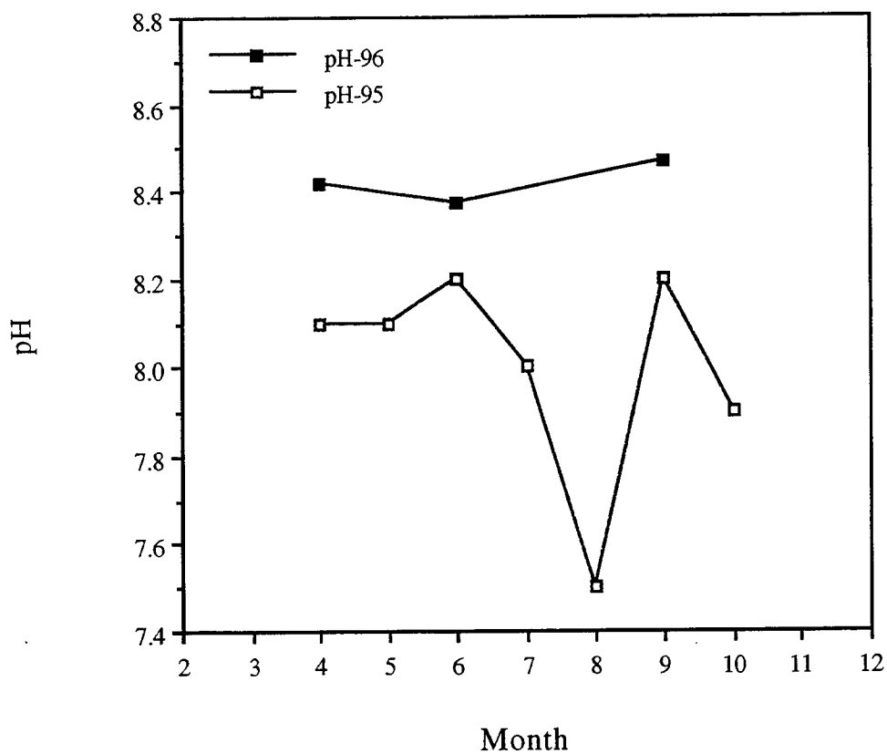
Figure 14. Soil pH during the 1995 and 1996 seasons at the Cambridge-Fall field site. Soil samples were collected within 4 m from the pavement edge, to a depth of 10 cm. Each data point represents the mean value from 16 soil samples.
