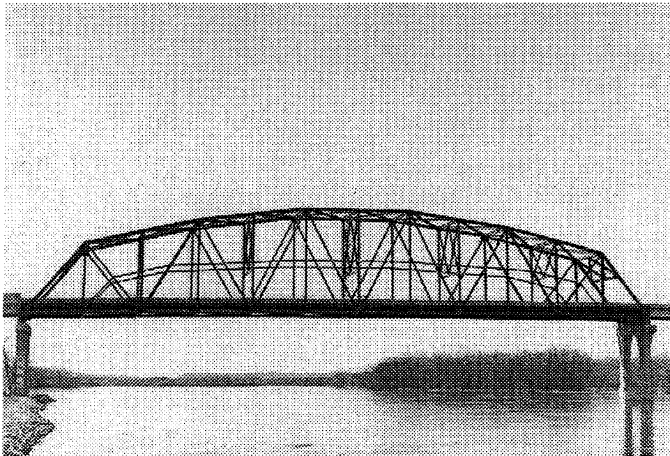
Figure 1.1 Wabasha County Bridge
