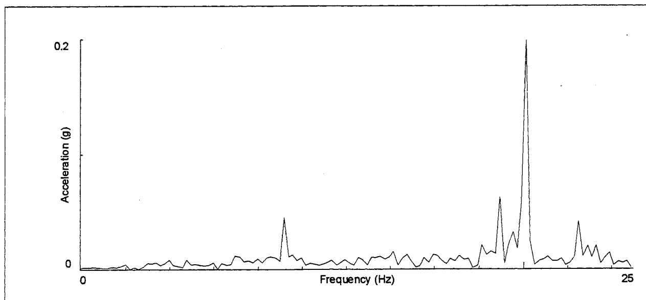
Figure 5.2 Typical Amplitude Spectrum
