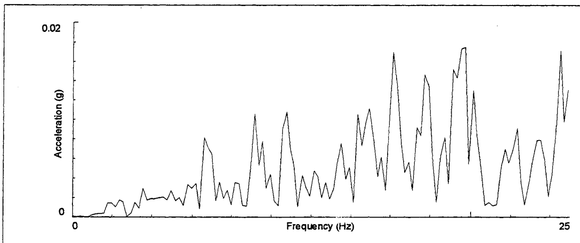
Figure 5.3 Wide Band Amplitude Spectrum
