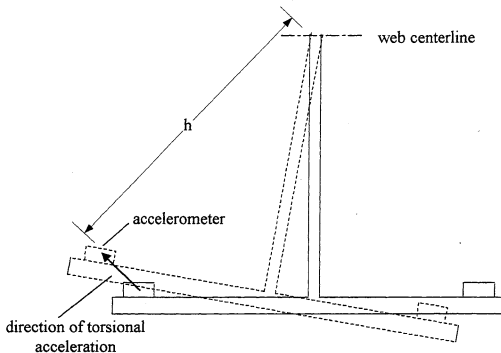
Figure 6.1 Torsional Acceleration Schematic
