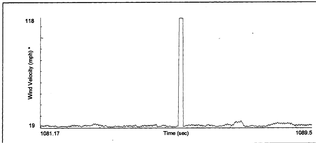
Figure 2.9 Typical Wind Speed Spike
