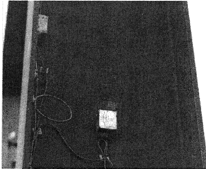
Figure 2.6 Installed Accelerometers
