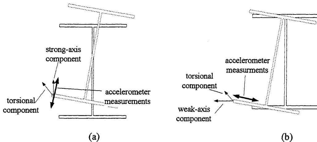
Figure 6.2 Acceleration Components
