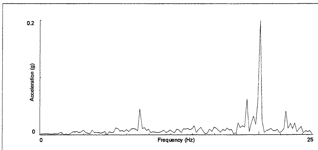
Figure 4.1 Fourier Amplitude Spectrum
