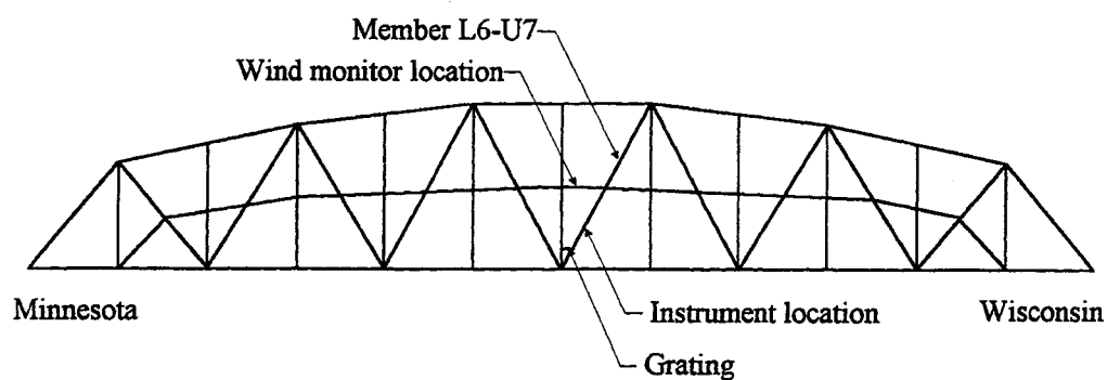
Figure 2.3 Upstream Truss, Wabasha County Bridge
