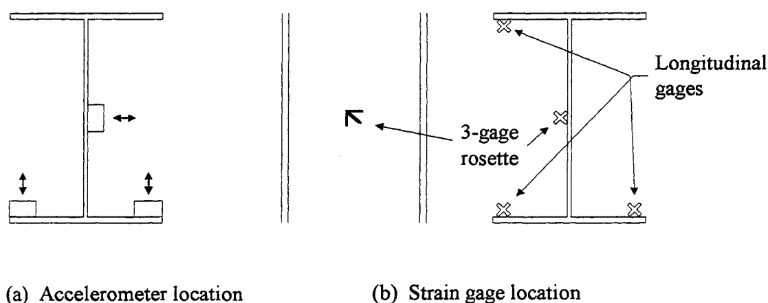
Figure 2.4 Instrument Location
