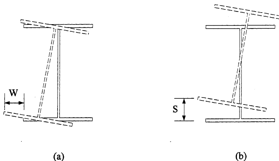
Figure 6.3 Combined Displacement Effects
