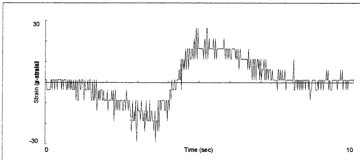
Figure 5.1 Typical Longitudinal Strain
