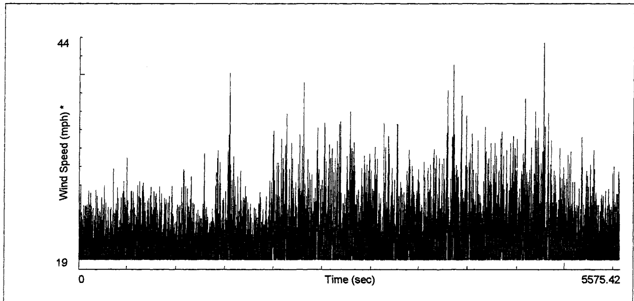
Figure 4.5 Continuous Record of Wind Speed Data
