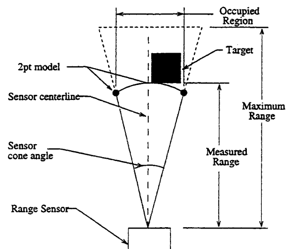
Figure 4.1: Two dimensional model of range sensor.
