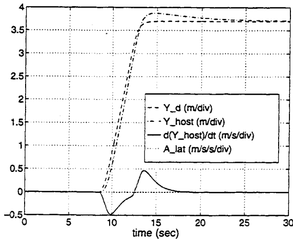
Figure B.7: Plot of lateral parameters for lane change maneuver with V_{long} = 3.0 \text{ m/s} .
