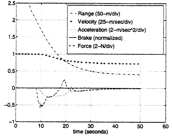
Figure 3.12: Time domain plot with dominant pole of .2 with \zeta = 1.7 .
