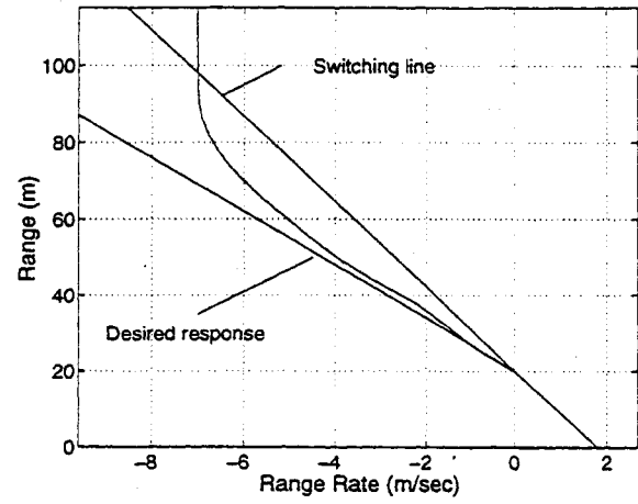
Figure 3.8: R, \dot{R} plot dominant pole of .2 with \zeta = 1.7 .
