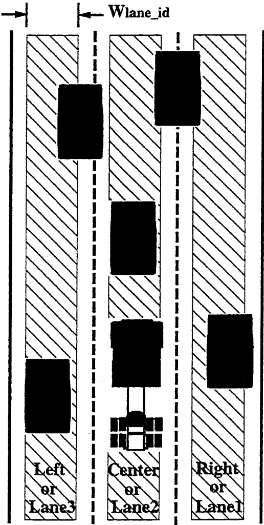
Figure 4.7: Various target positions and corresponding lane identification.
