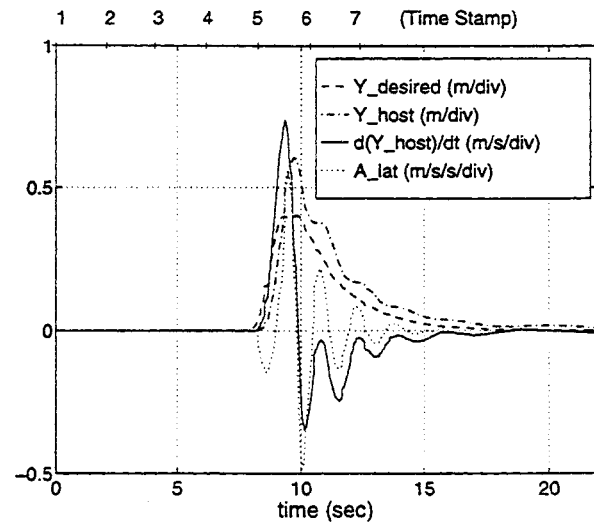
Figure 5.9: Time history of lateral parameters for "Passing parked car" scenario.
