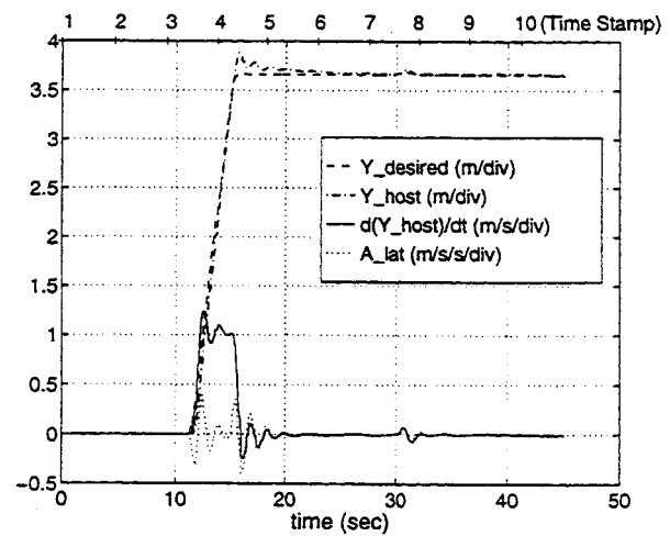
Figure 5.12: Time history of lateral parameters for "Overtaking" scenario.
