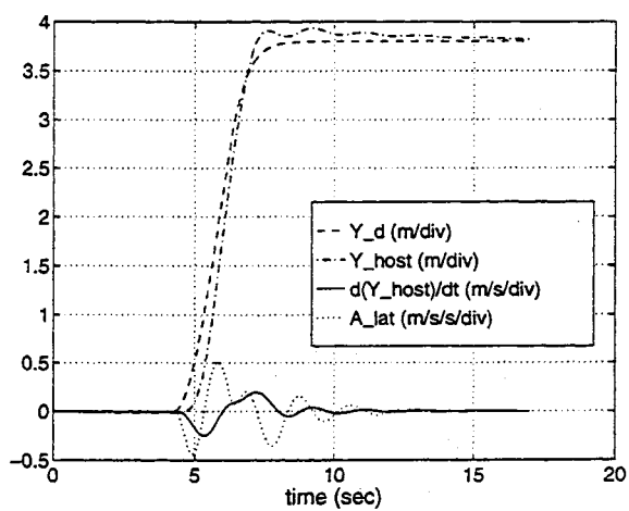
Figure B.13: Plot of lateral parameters for lane change maneuver with V_{long} = 20.0 \text{ m/s} .
