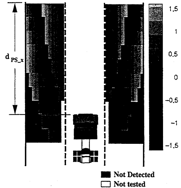
Figure 4.19: Y_{error} plot for configuration 3A using 1 pt.cntr target model.
