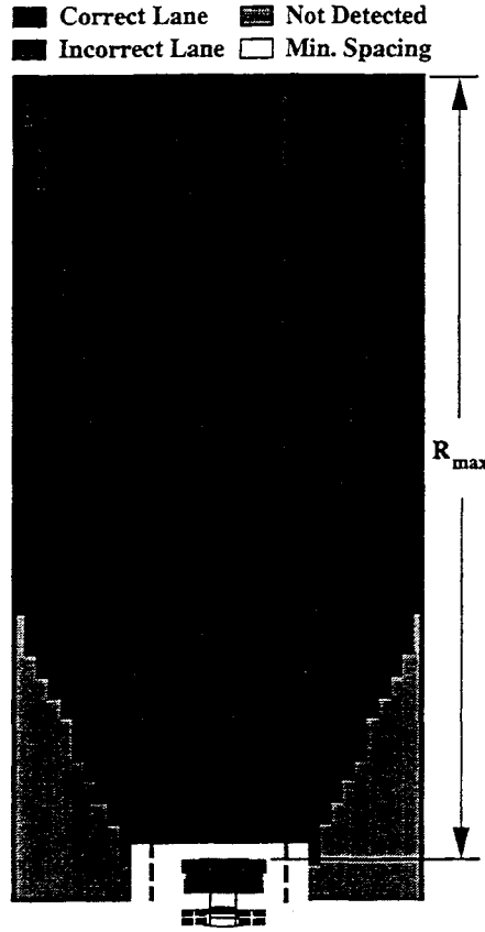
Figure 4.8: L_{id_{error}} plot example.
