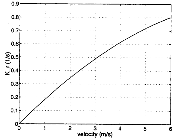
Figure B.3: Plot of K_r versus V_{long} .
