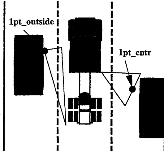
Figure 4.3: The 1 pt.cntr and 1 pt.outside target models for reducing measurement error.
