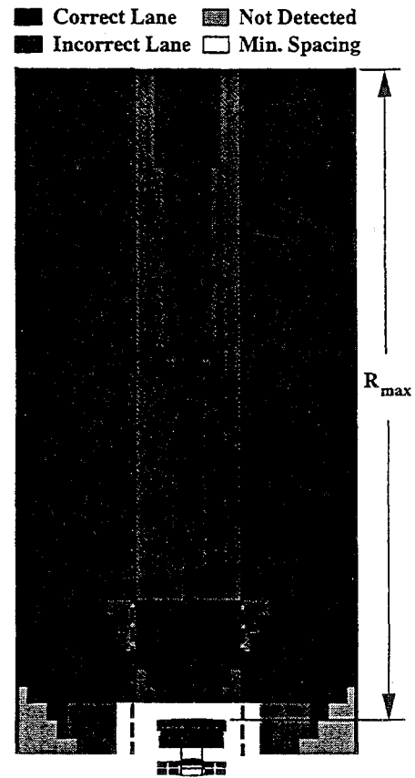
Figure 4.16: Lane identification plot using configuration 3A.
