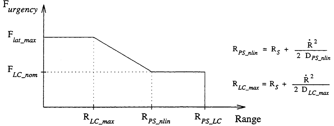
Figure 2.23: Magnitude of F_{urgency} as a function of the measured range.
