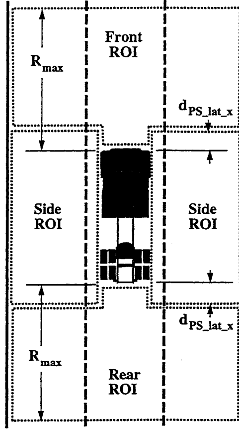
Figure 2.18: Regions of Interest for the lane change system.
