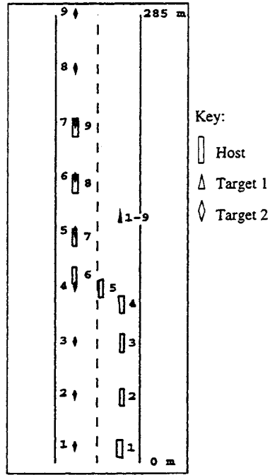
Figure 5.13: Time history of the vehicle-road configuration for "Waiting to overtake" scenario. V_{const} = V_{T1} and \Delta T = 6.6 seconds.
