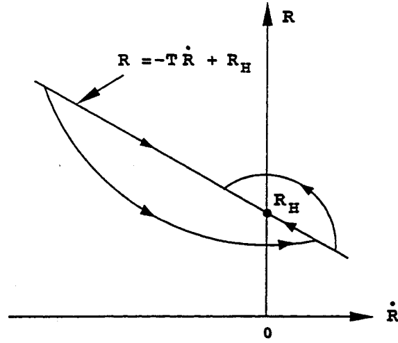
Figure 2.2: Typical trajectories in the R, \dot{R} plane for headway controller.
