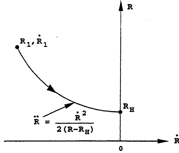
Figure 2.3: Constant deceleration trajectory in the R, \dot{R} .
