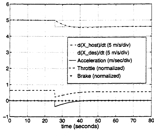
Figure A.6: Velocity controller response to a -2.0 \text{ m/s} step input.
