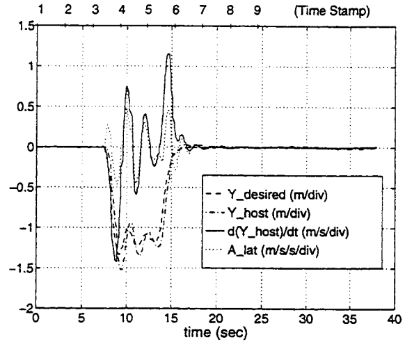
Figure 5.18: Time history of lateral parameters for “Drifting car” scenario.
