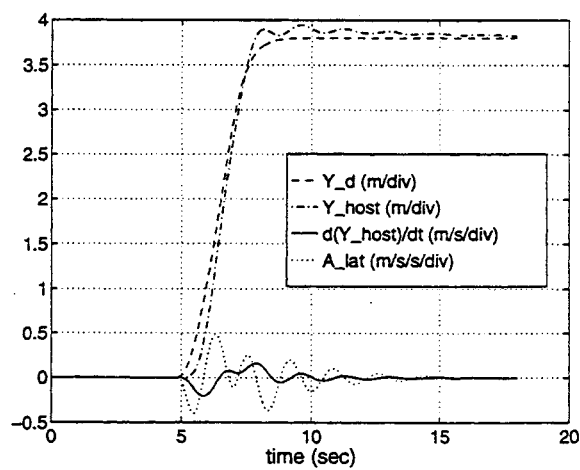
Figure B.14: Plot of lateral parameters for lane change maneuver with V_{long} = 25.0 \text{ m/s} .
