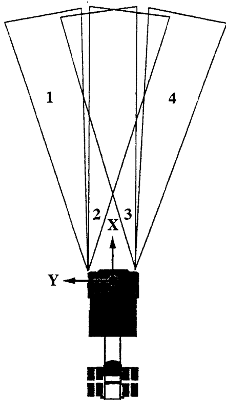
Figure 4.11: Range sensor placement configuration 2.
