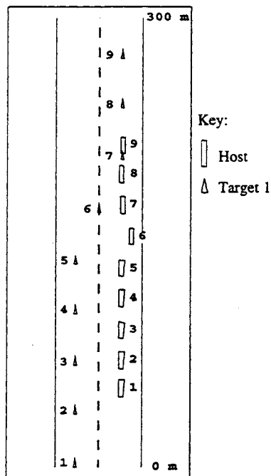
Figure 5.19: Time history of the vehicle-road configuration for "Passed and cut-off" scenario. V_{const} = 15 \text{ m/s} and \Delta T = 2.0 seconds.
