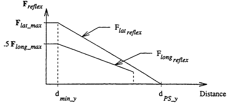
Figure 2.17: Magnitude of the lateral reflexive force equations.
