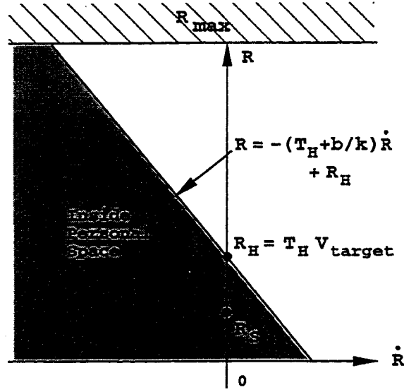
Figure 2.11: Personal space for the longitudinal linear force defined on the R, \dot{R} phase plane.
