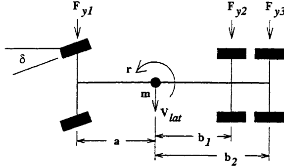
Figure B.1: Simple lateral model of truck with applied forces.
