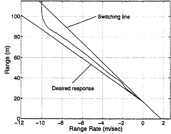
Figure 3.2: R, \dot{R} plot with b = 2.132 , k = .232 and T = 1 .
