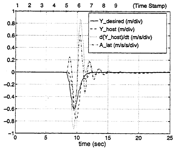
Figure 5.21: Time history of lateral parameters for "Passed and cut-off" scenario.
