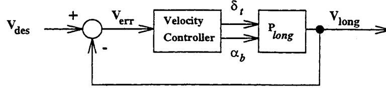
Figure A.3: Block diagram for velocity control loop.
