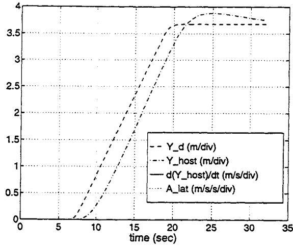
Figure B.5: Plot of lateral parameters for lane change maneuver with V_{long} = 1.0 \text{ m/s} .
