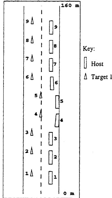
Figure 5.17: Time history of the vehicle-road configuration for “Drifting car” scenario. V_{const} = 20 \text{ m/s} and \Delta T = 3.0 seconds.
