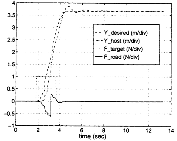
Figure 3.23: Emergency lane change maneuver with compensation for the tracking error of the lateral controller.
