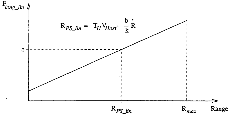
Figure 2.10: Longitudinal linear force vs. range for constant V_{host} and constant V_{target} .
