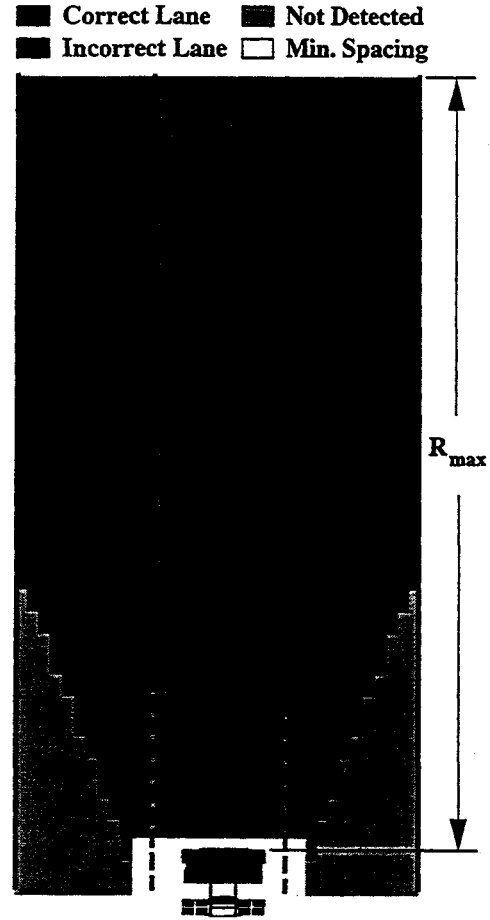
Figure 4.14: Lane identification plot using sensor configuration 2C with sensor orientation per Table 4.4
