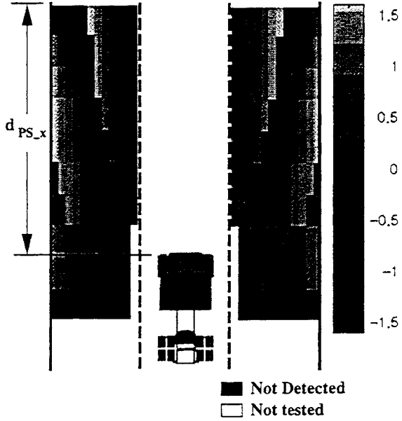
Figure 4.21: Lateral error plot for configuration 4A using 2 pt target model for the Amerigon sensors.
