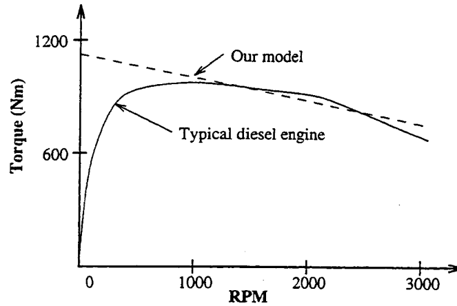
Figure A.1: Engine torque vs. speed for typical diesel engine and for our engine model. The torque levels are based on full throttle actuation ( \delta_t = 1.0 ).
