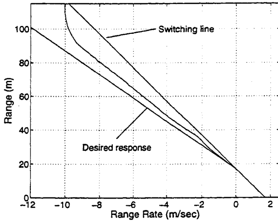
Figure 3.3: R, \dot{R} plot with b = 2.132 , k = .232 and T = 1.5 .
