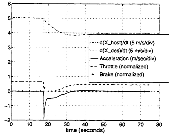
Figure A.7: Velocity controller response to a -5.0 \text{ m/s} step input.
