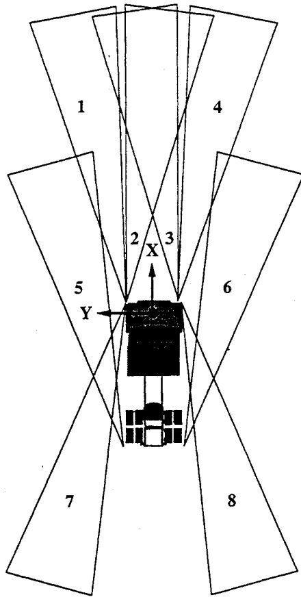
Figure 4.15: Range sensor configuration 3.
