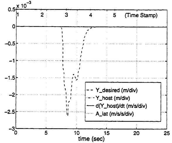
Figure 5.6: Time history of lateral parameters for “Passed by car” scenario
