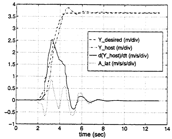
Figure 3.19: Emergency lane change maneuver when traveling at 25 m/s (55.9 mph).
