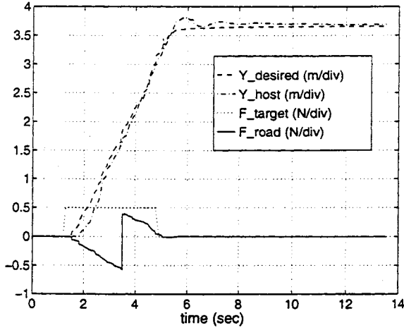
Figure 3.22: Nominal lane change maneuver with compensation for the tracking error of the lateral controller.
