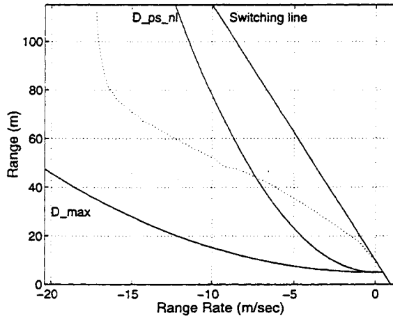
Figure 3.15: (R, \dot{R}) plot for headway tracking when nonlinear forces are used. V_{host} = 25.0 m/s initially and V_{target} = 8.0 m/s for the maneuver.
