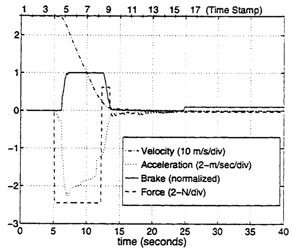
Figure 5.29: Time history of longitudinal parameters for "Approaching traffic jam" scenario.
