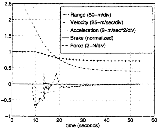
Figure 3.13: Time domain plot with dominant pole of .2 with \zeta = 2.0 .
