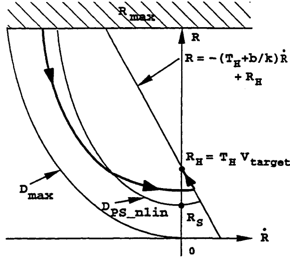
Figure 2.14: R, \dot{R} diagram for headway tracking using nonlinear forces.
