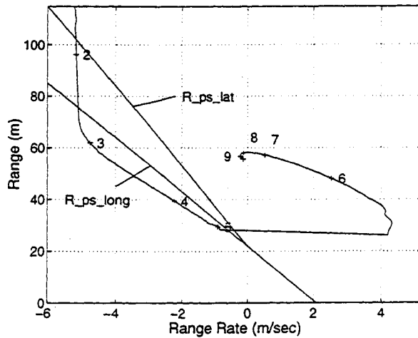
Figure 5.15: (R, \dot{R}) phase plot for "Waiting to overtake" scenario.
