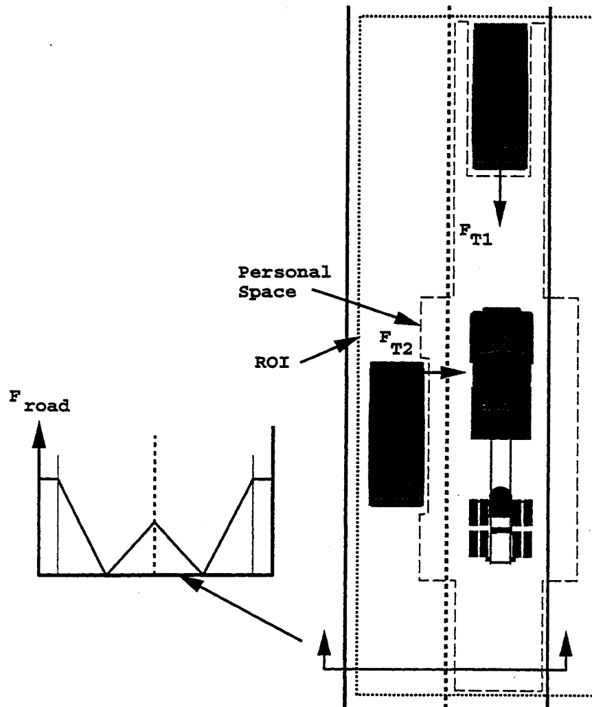
Figure 2.1: Virtual bumper control schematic for highway vehicle.
