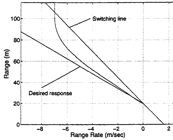
Figure 3.7: R, \dot{R} plot dominant pole of .2 with \zeta = 1.3 .
