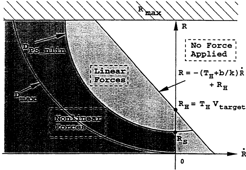
Figure 2.13: Linear and nonlinear longitudinal force zones defined in the R, \dot{R} plane.
