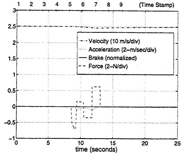
Figure 5.20: Time history of longitudinal parameters for "Passed and cut-off" scenario.
