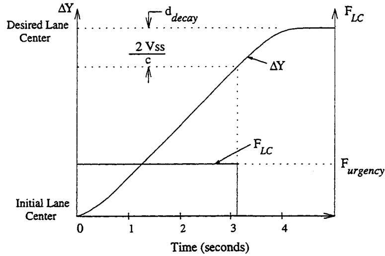
Figure 2.21: Lane change profile for the F_{LC} pulse function.
