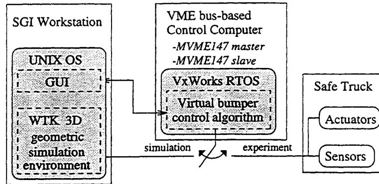
Figure 5.1: Schematic of the real-time simulation environment.
