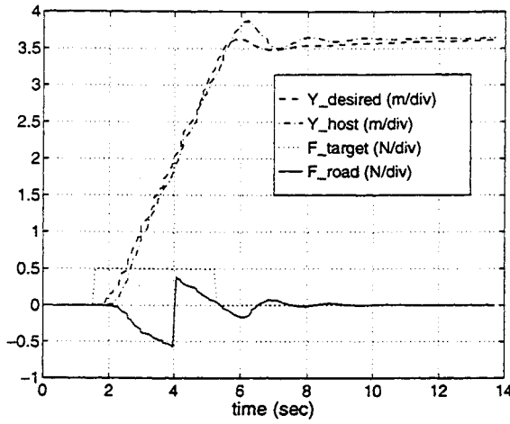
Figure 3.20: Nominal lane change maneuver without compensation for the tracking error of the lateral controller.
