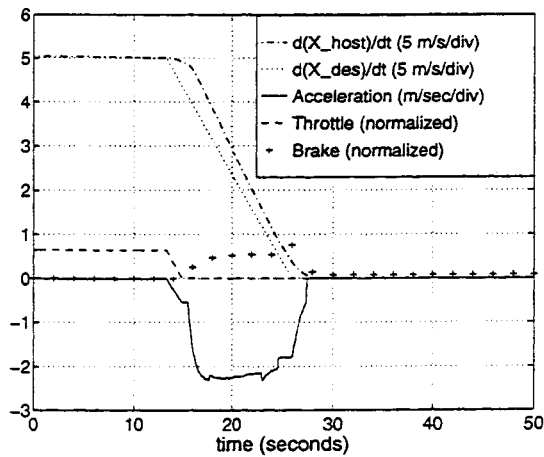
Figure A.8: Velocity controller response to a constant deceleration profile of -0.2 \text{ g/s} .
