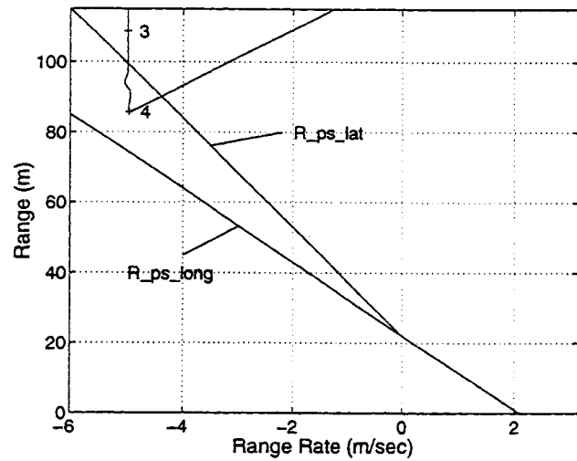
Figure 5.11: (R, \dot{R}) phase plot for "Overtaking" scenario.
