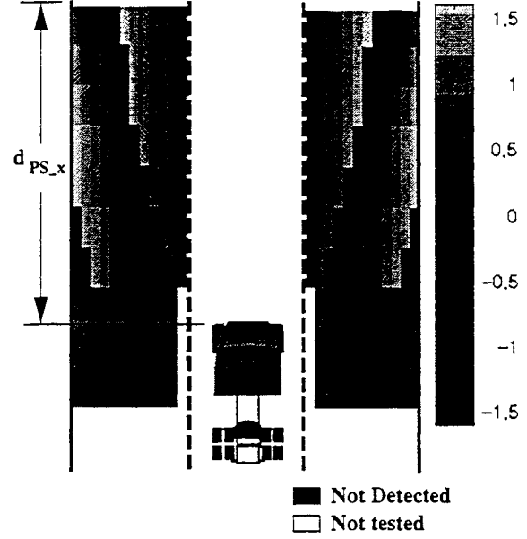
Figure 4.22: Lateral error plot for configuration 4A using 1 pt.cntr target model for the Amerigon sensors.
