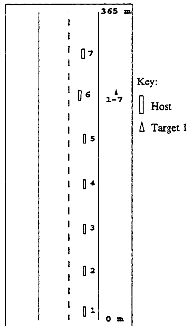
Figure 5.7: Time history of the vehicle-road configuration for "Passing parked car" scenario. V_{const} = 0 and \Delta T = 2.0 seconds.
