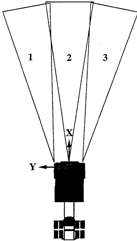
Figure 4.9: Range sensor placement configuration 1 with only the three forward facing sensors shown.
