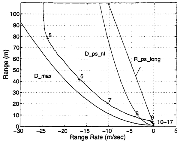
Figure 5.28: (R, \dot{R}) phase plot for "Approaching traffic jam" scenario.
