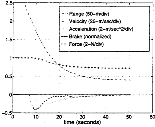
Figure 3.11: Time domain plot with dominant pole of .2 with \zeta = 1.3 .
