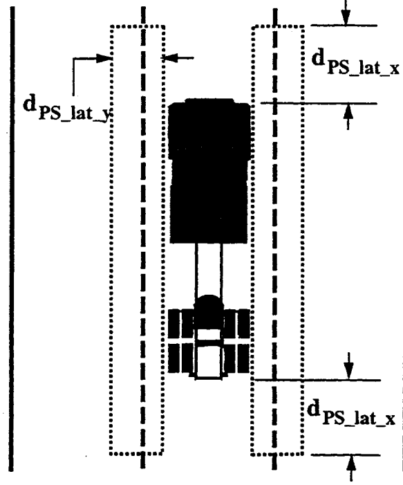
Figure 2.16: Lateral personal space for the host vehicle.
