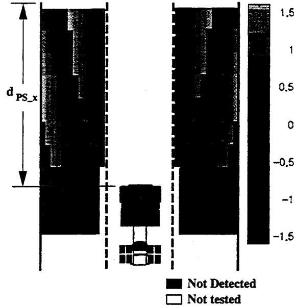
Figure 4.23: Lateral error plot for configuration 4B using 1 pt.cntr target model for the Amerigon sensors.
