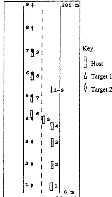
Figure 5.4: Example of a time history of the vehicle-road configuration for “Waiting to Overtake” scenario. V_{const} = V_{T1} and \Delta T = 6.6 seconds.
