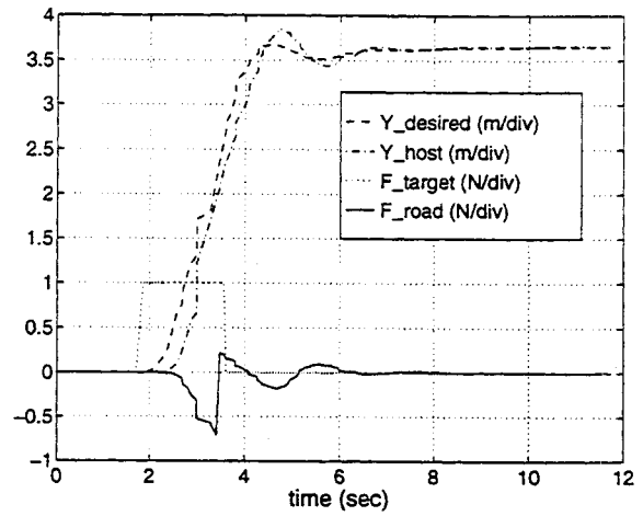
Figure 3.21: Emergency lane change maneuver without compensation for the tracking error of the lateral controller.
