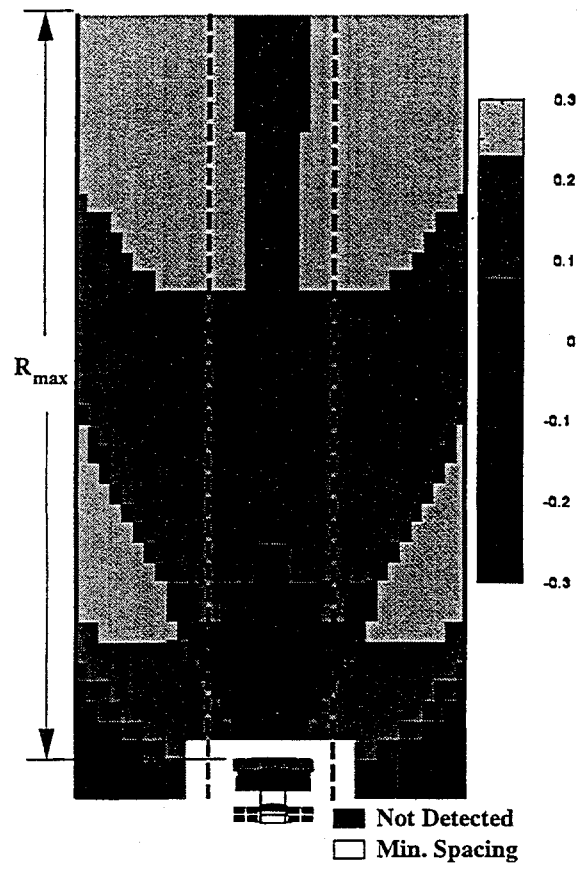
Figure 4.17: R_{error} plot using configuration 3A.
