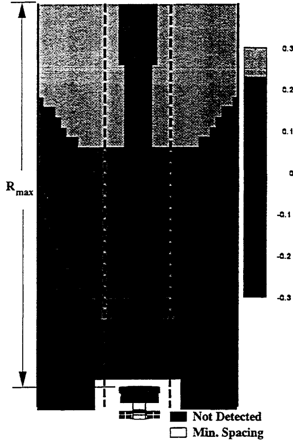
Figure 4.5: Range error plot example.
