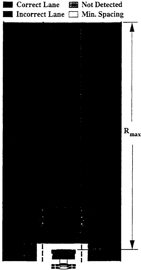
Figure 4.24: Lane identification plot using configuration 4A.
