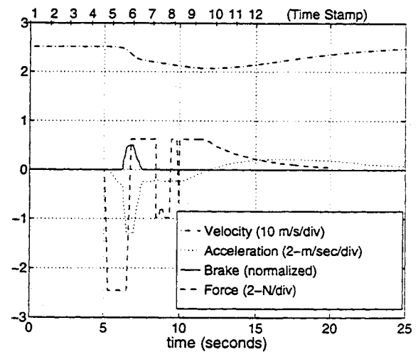
Figure 5.25: Time history of longitudinal parameters for "Stalled car on highway" scenario.
