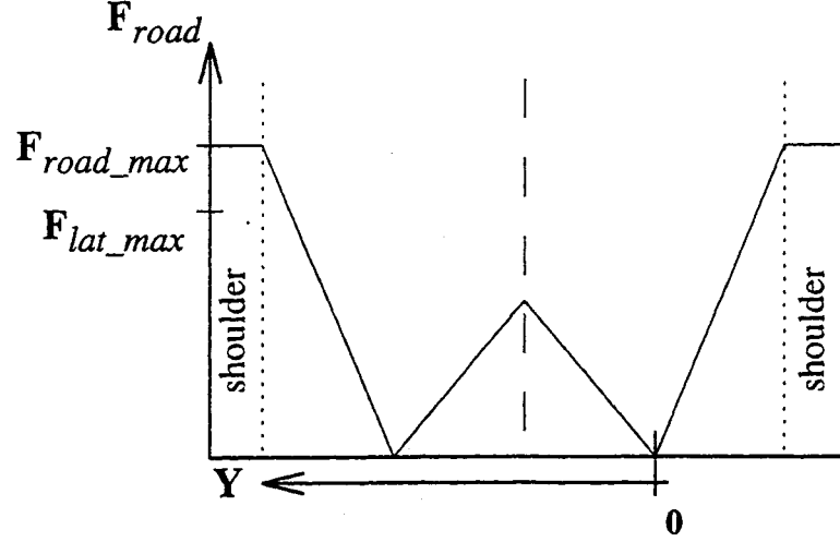
Figure 2.24: Virtual road force profile for a two-lane highway.
