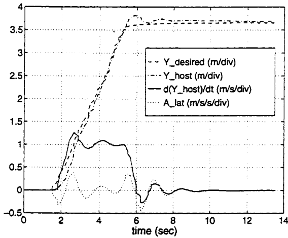
Figure 3.18: Nominal lane change maneuver when traveling at 25 m/s (55.9 mph).
