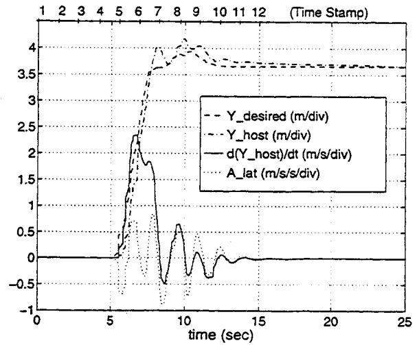
Figure 5.23: Time history of lateral parameters for "Stalled car on highway" scenario.
