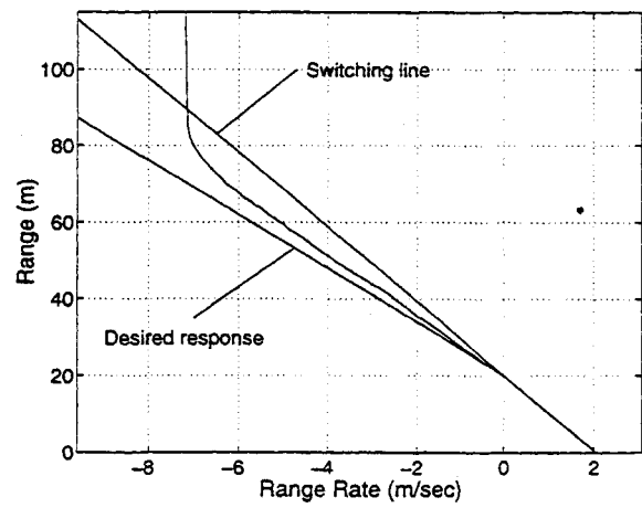
Figure 3.10: R, \dot{R} plot dominant pole of .2 with \zeta = 3.0 .
