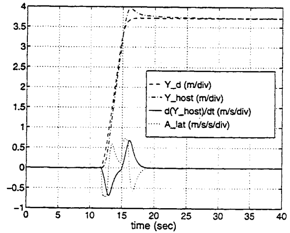
Figure B.8: Plot of lateral parameters for lane change maneuver with V_{long} = 4.0 \text{ m/s} .
