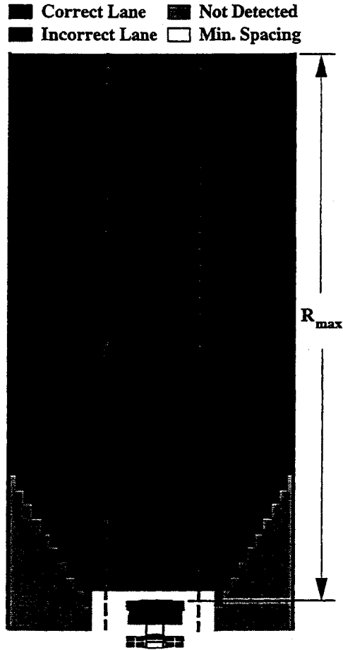
Figure 4.13: Lane identification plot using sensor configuration 2B with sensor orientation per Table 4.4
