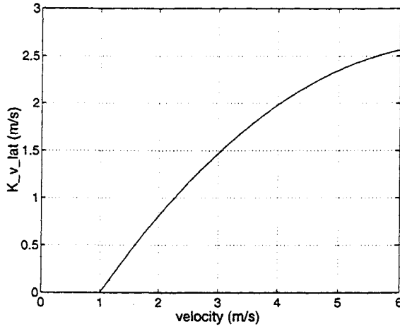
Figure B.2: Plot of K_{V_{lat}} versus V_{long} .
