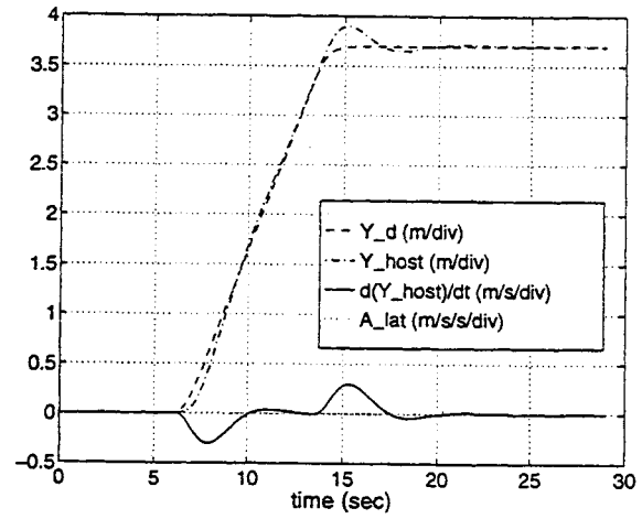
Figure B.6: Plot of lateral parameters for lane change maneuver with V_{long} = 2.0 \text{ m/s} .
