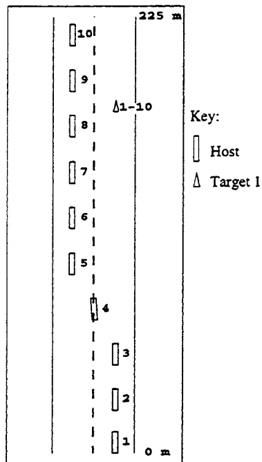
Figure 5.10: Time history of the vehicle-road configuration for "Overtaking" scenario. V_{const} = V_{T1} and \Delta T = 4.5 seconds.
