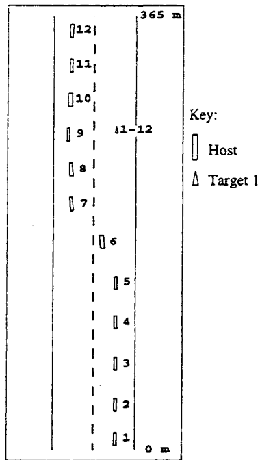
Figure 5.22: Time history of the vehicle-road configuration for "Stalled car on highway" scenario. V_{const} = 0 \text{ m/s} and \Delta T = 1.3 \text{ seconds} .
