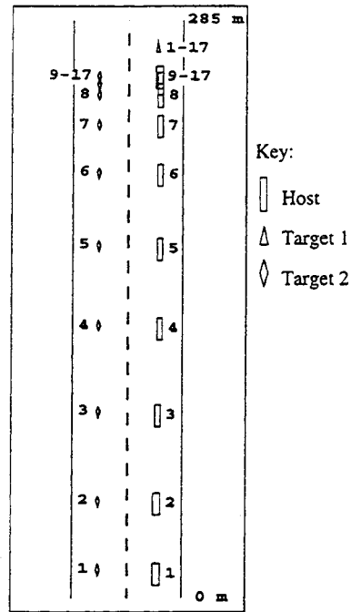
Figure 5.26: Time history of the vehicle-road configuration for "Approaching traffic jam" scenario. V_{const} = 0 \text{ m/s} and \Delta T = 1.6 \text{ seconds} .
