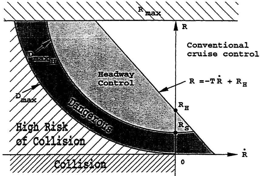
Figure 2.4: Regions in the R, \dot{R} phase diagram.
