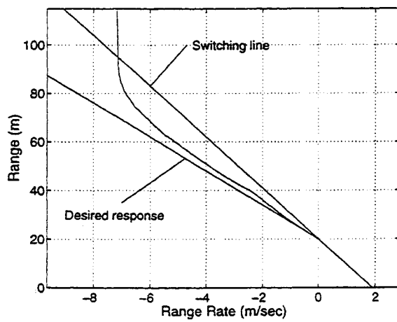
Figure 3.9: R, \dot{R} plot dominant pole of .2 with \zeta = 2.0 .
