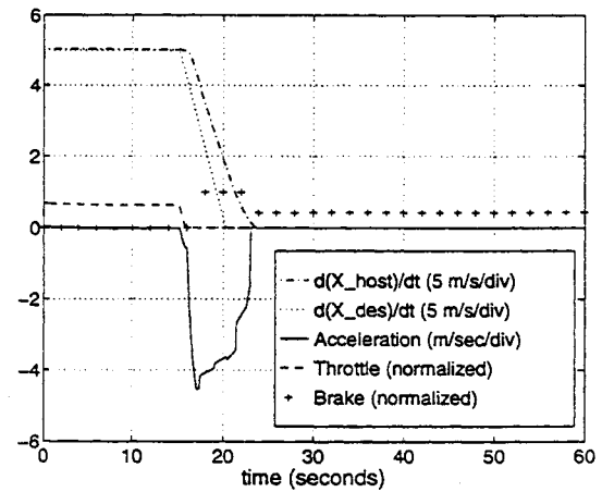
Figure A.9: Velocity controller response to a constant deceleration profile of -0.5 \text{ g/s} .
