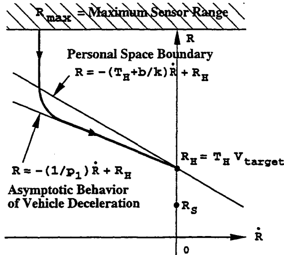
Figure 2.12: R, \dot{R} diagram for typical headway tracking.
