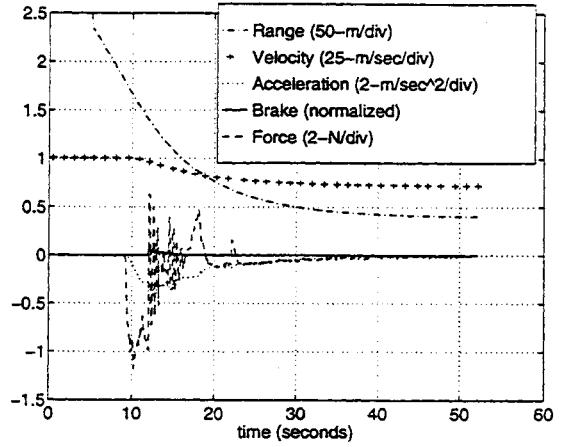
Figure 3.14: Time domain plot with dominant pole of .2 with \zeta = 3 .
