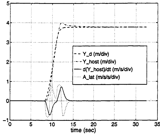
Figure B.9: Plot of lateral parameters for lane change maneuver with V_{long} = 5.0 m/s.
