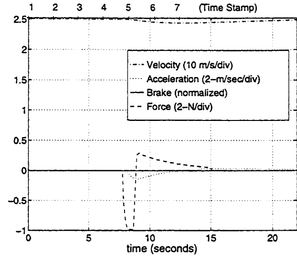
Figure 5.8: Time history of longitudinal parameters for "Passing parked car" scenario.
