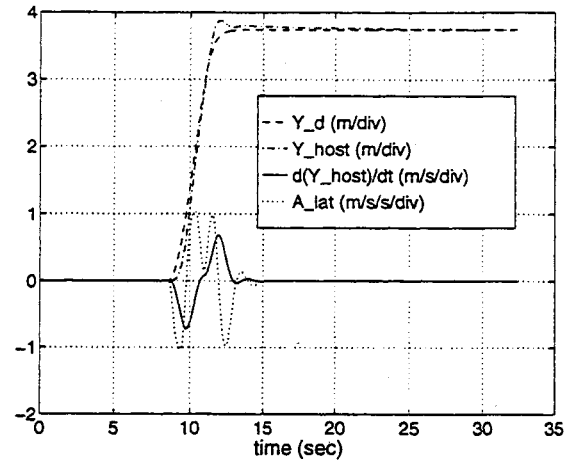
Figure B.10: Plot of lateral parameters for lane change maneuver with V_{long} = 7.5 m/s.
