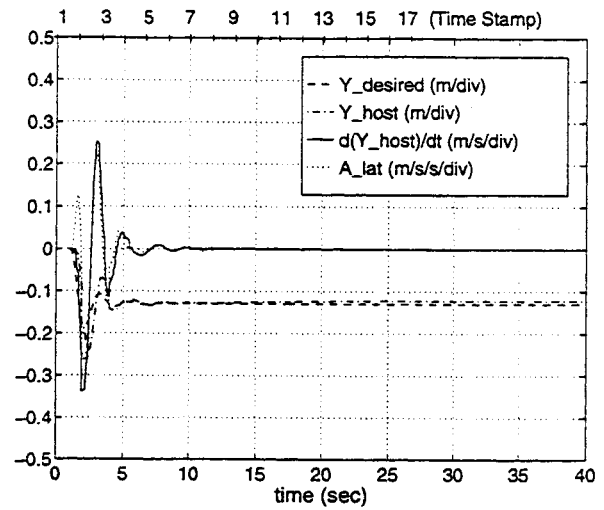
Figure 5.27: Time history of lateral parameters for "Approaching traffic jam" scenario.
