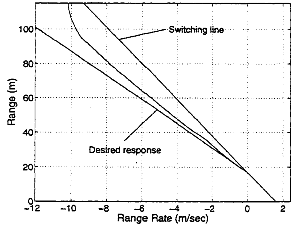
Figure 3.4: R, \dot{R} plot with b = 2.132 , k = .232 and T = 2 .
