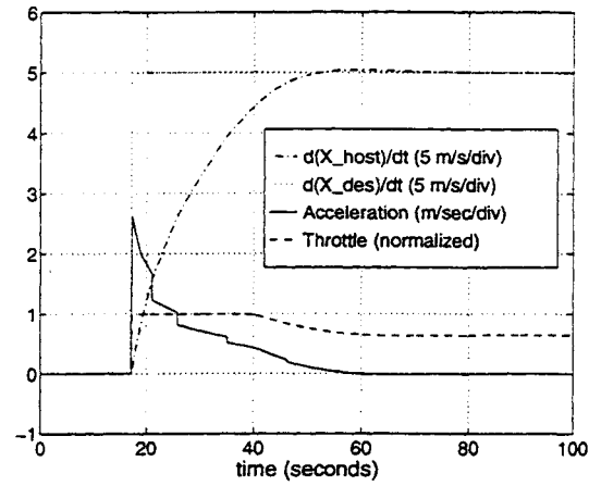
Figure A.5: Velocity controller response to a 25.0 m/s step input.
