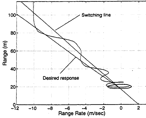
Figure 3.1: R, \dot{R} plot with b = 2.132 , k = .232 and T = 0 (no predictive terms).
