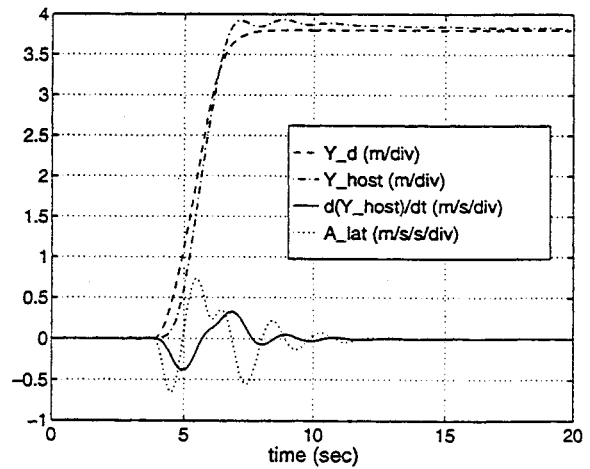
Figure B.12: Plot of lateral parameters for lane change maneuver with V_{long} = 15.0 m/s.
