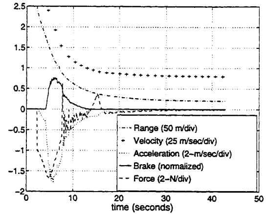
Figure 3.16: Time domain plot for headway tracking when nonlinear forces are used. V_{host} = 25.0 m/s initially and V_{target} = 8.0 m/s for the maneuver.
