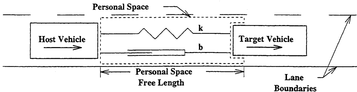
Figure 2.7: One dimensional impedance control for highway vehicle.
