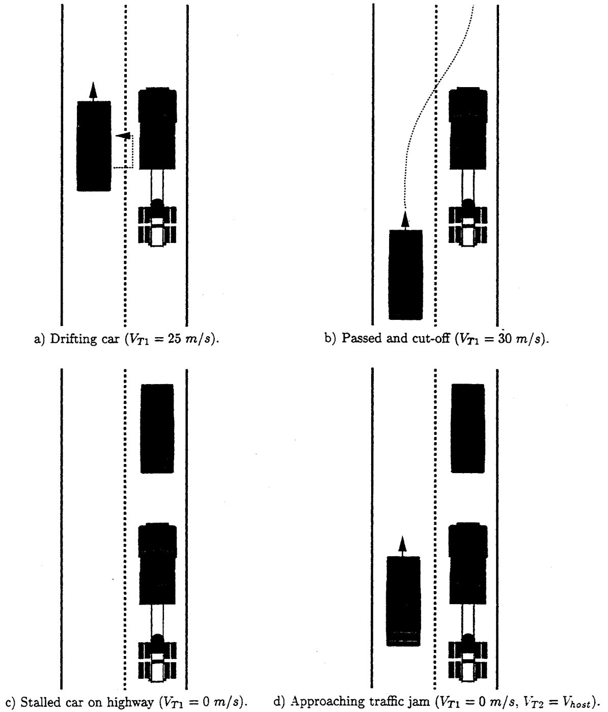
Figure 5.3: Emergency driving scenarios.
