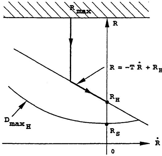
Figure 2.5: Typical R, \dot{R} trajectories for small initial relative velocity.
