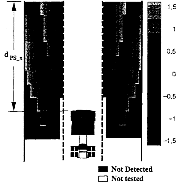
Figure 4.6: Lateral error plot example.
