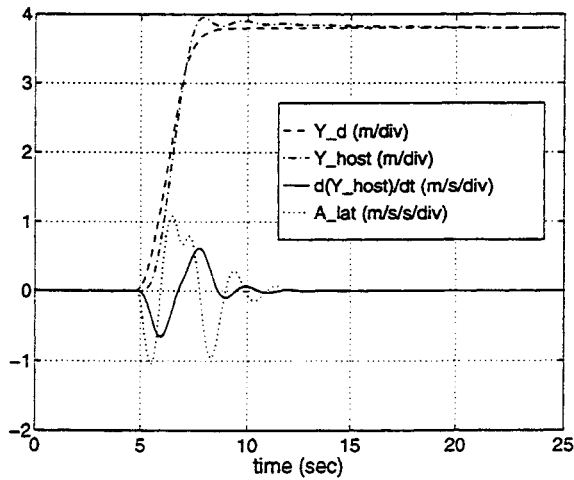
Figure B.11: Plot of lateral parameters for lane change maneuver with V_{long} = 10.0 m/s.
