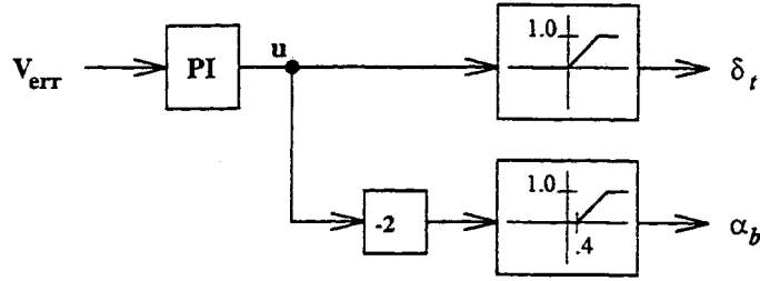
Figure A.4: Block diagram for only the velocity controller.
