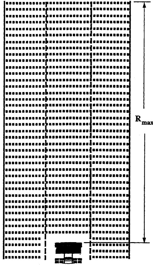
Figure 4.4: Grid of target location points for evaluation of sensor measurements.
