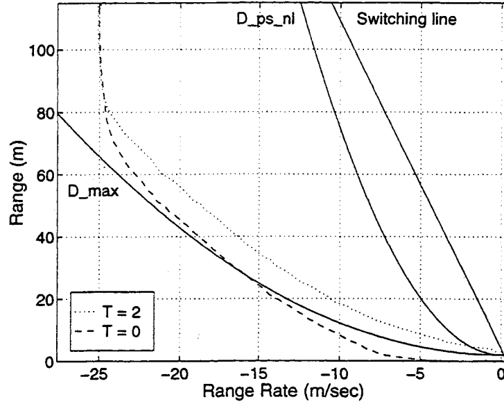
Figure 3.5: (R, \dot{R}) plot showing effect of nonlinear force with and without the predictive compensation during emergency braking.
