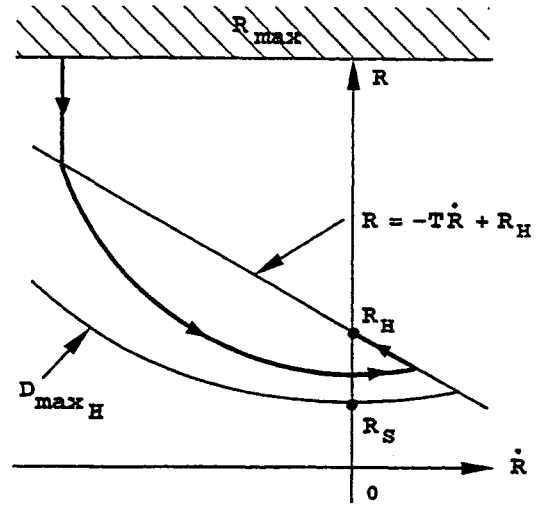
Figure 2.6: Typical R, \dot{R} trajectories for large initial relative velocity.
