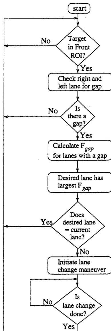
Figure 2.19: Flow chart for selecting the desired lane.
