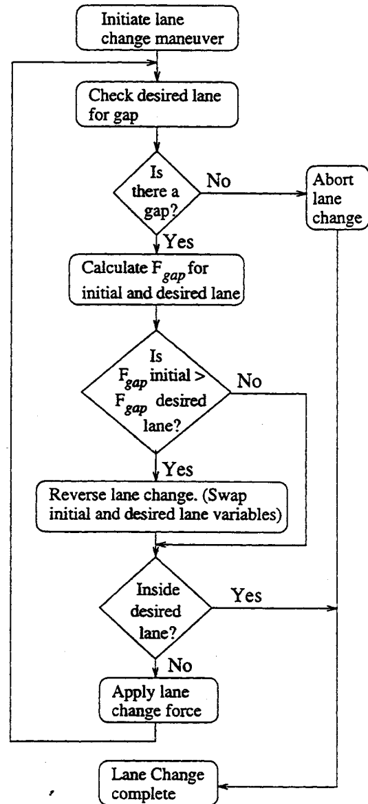
Figure 2.20: Flow chart for performing a lane maneuver.
