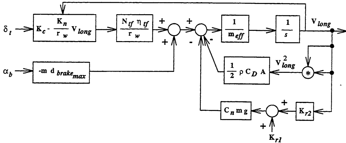
Figure A.2: Block diagram for longitudinal dynamic model of vehicle.
