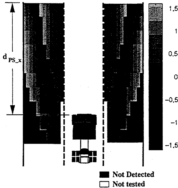
Figure 4.18: Y_{error} plot using configuration 3A.
