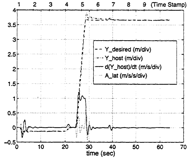
Figure 5.14: Time history of lateral parameters for "Waiting to overtake" scenario.
