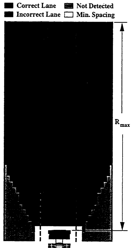
Figure 4.12: Lane identification plot using sensor configuration 2A.
