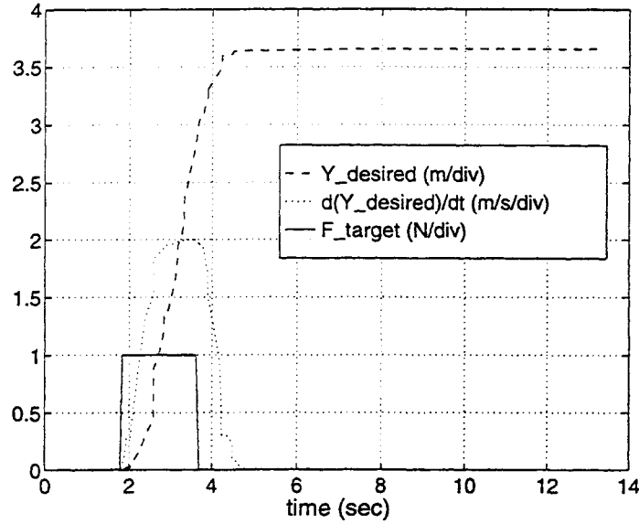
Figure 3.17: Emergency lane change profile when F_{lat_{max}} is used in lane change force.
