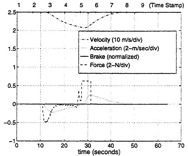
Figure 5.16: Time history of longitudinal parameters for "Waiting to overtake" scenario.
