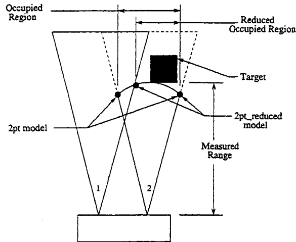
Figure 4.2: Overlapping sensors to reduce the occupied region.
