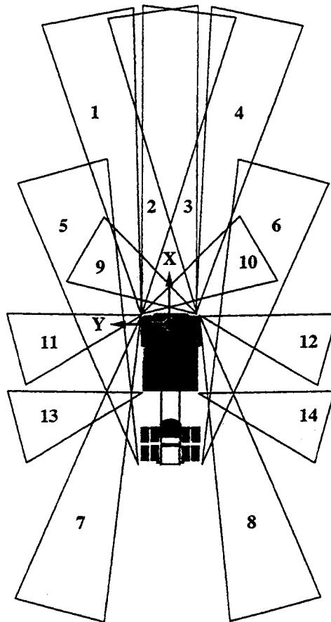
Figure 4.20: Range sensor configuration 4.
