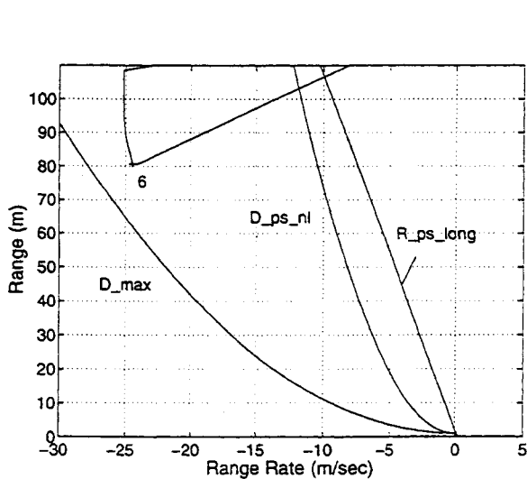
Figure 5.24: (R, \dot{R}) phase plot for "Stalled car on highway" scenario.
