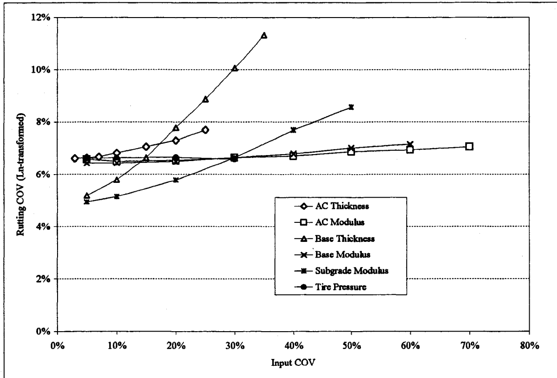
Figure 4.5 Phase II Rutting Variability Comparison.
