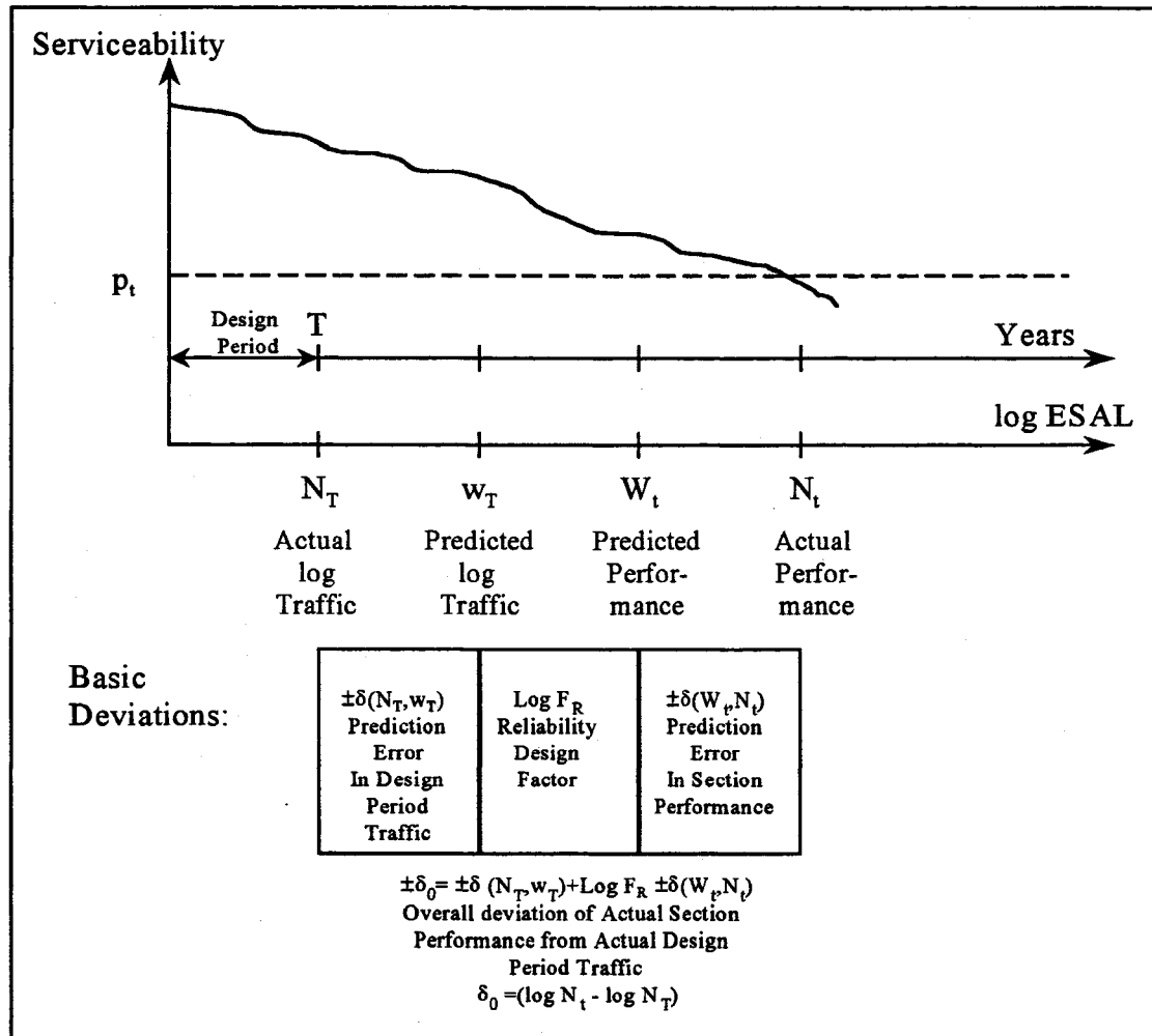
Figure 2.2 Basic Deviations of AASHTO Reliability (2).
