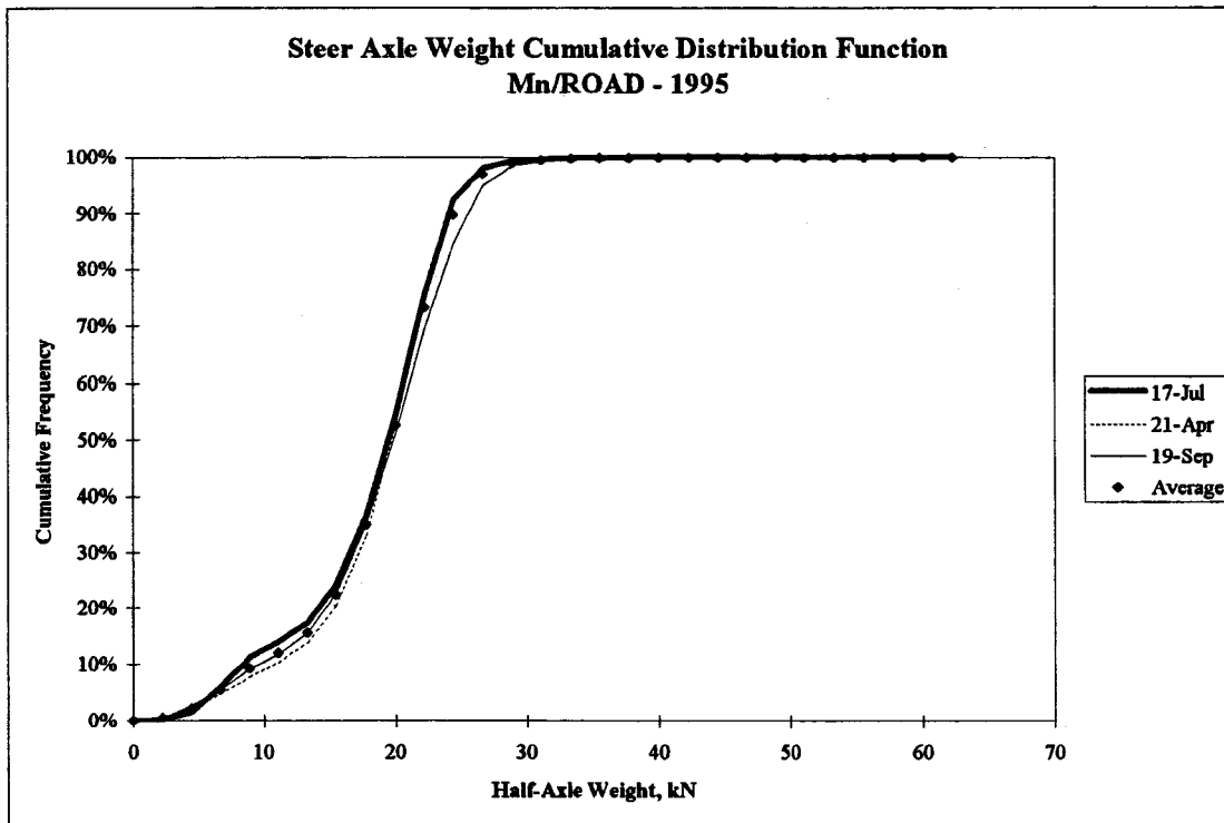
Figure 3.7 Steer Axle Weight – Cumulative Distribution Function.
