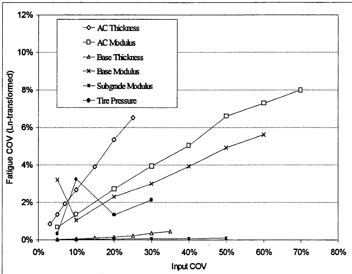
Figure 4.2 Phase I Fatigue Variability Comparison.
