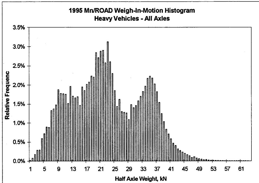
Figure 3.3 Half-Axle Weight Distribution at Mn/ROAD.
