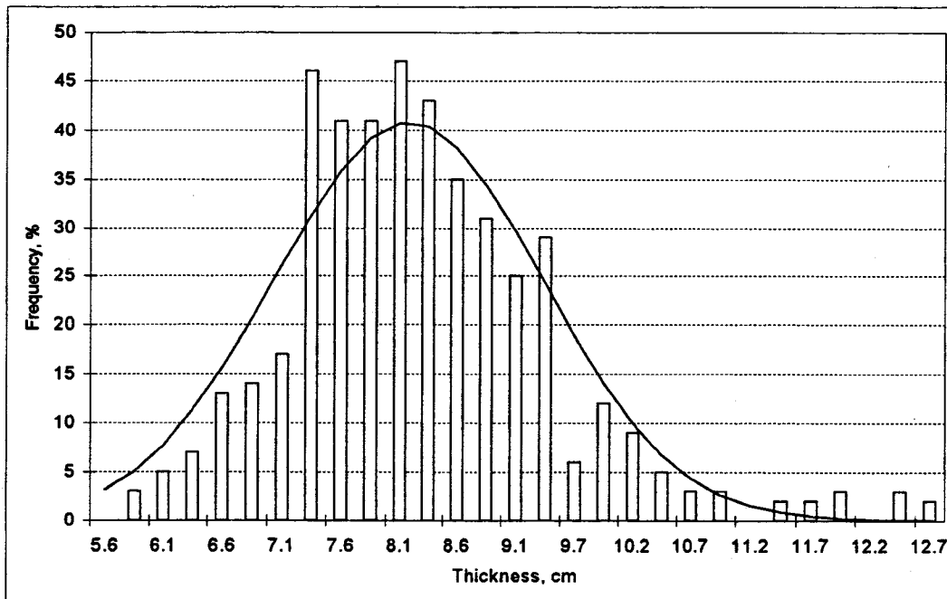
Figure 3.2 Surface Thickness Distribution of Cells 24, 27, 28, 31 at Mn/ROAD.
