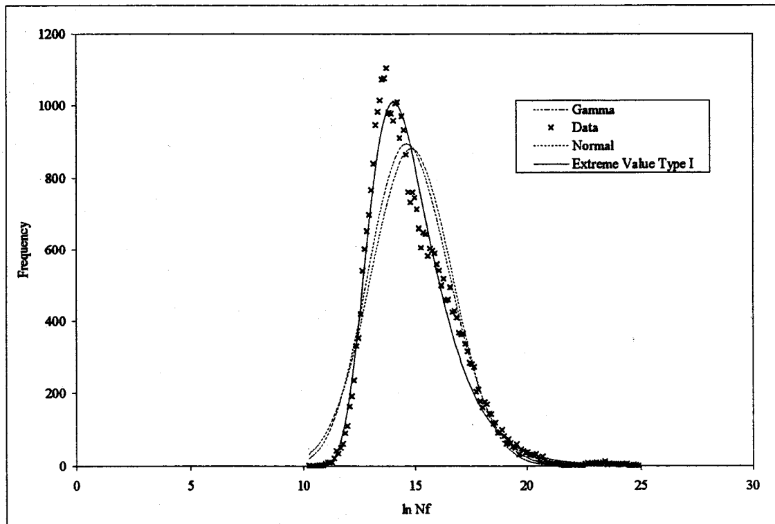
Figure 4.9 Phase III – Fatigue Curve Fitting, Tandem Axle Output.
