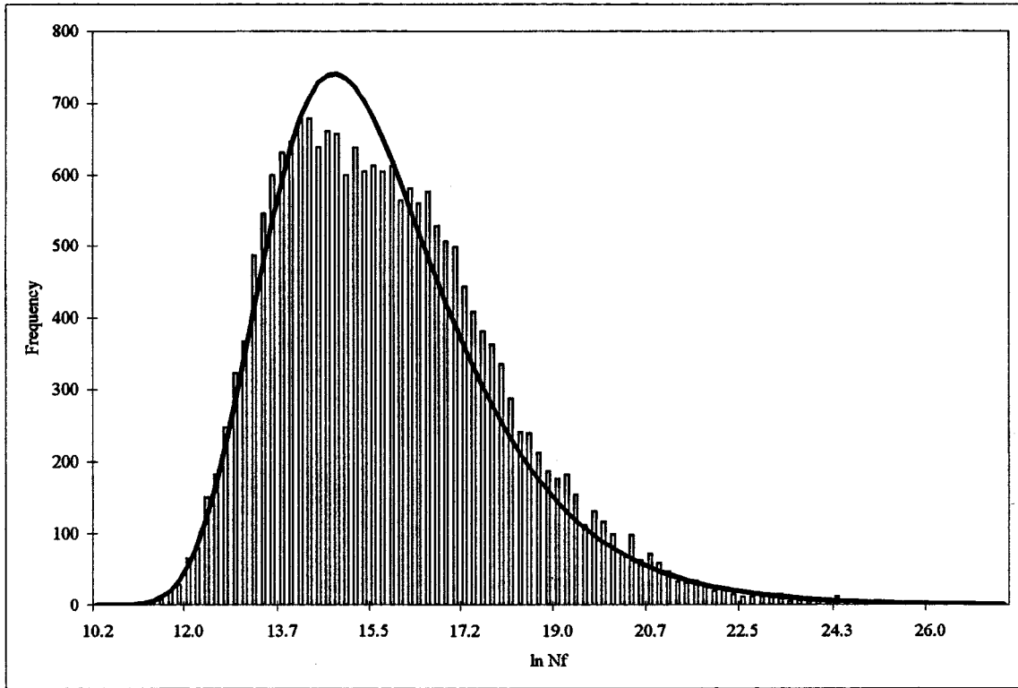
Figure 4.11 Phase III – Fatigue Curve Fitting, All Axle Output.
