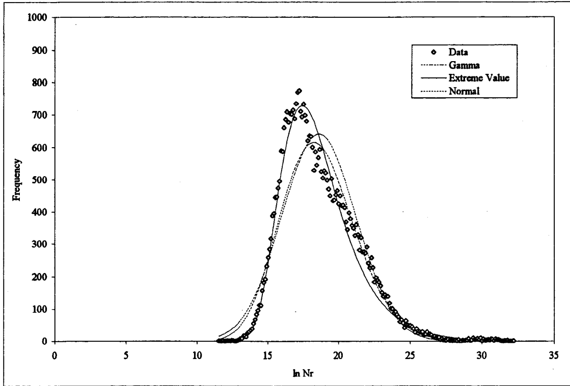
Figure 4.10 Phase III – Rutting Curve Fitting, Tandem Axle Output.
