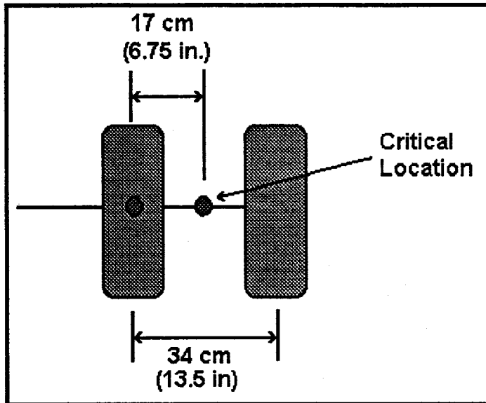
Figure A.6 Single Half-Axle Configuration in Plan View.
