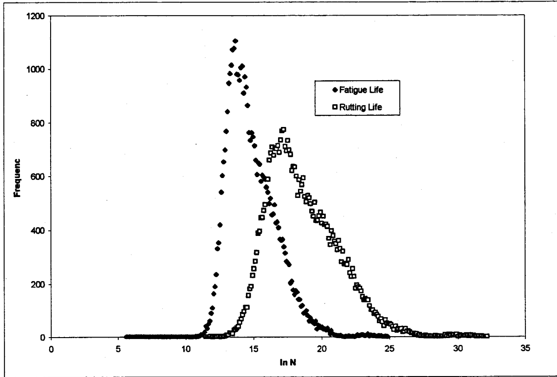
Figure 4.7 Phase III – Tandem Axle with Baseline Variability.
