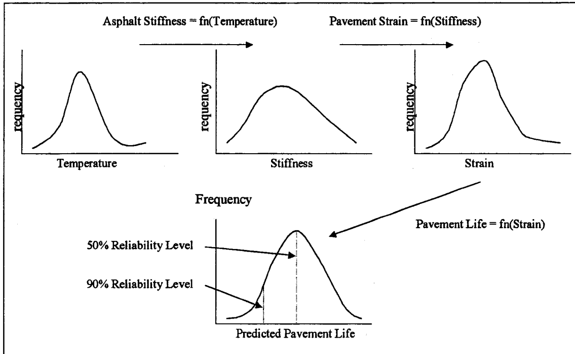
Figure 1.2 Example of Variability and Reliability.
