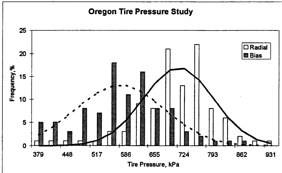
Figure 2.6 Tire Pressure Distribution by Tire Type (39).
