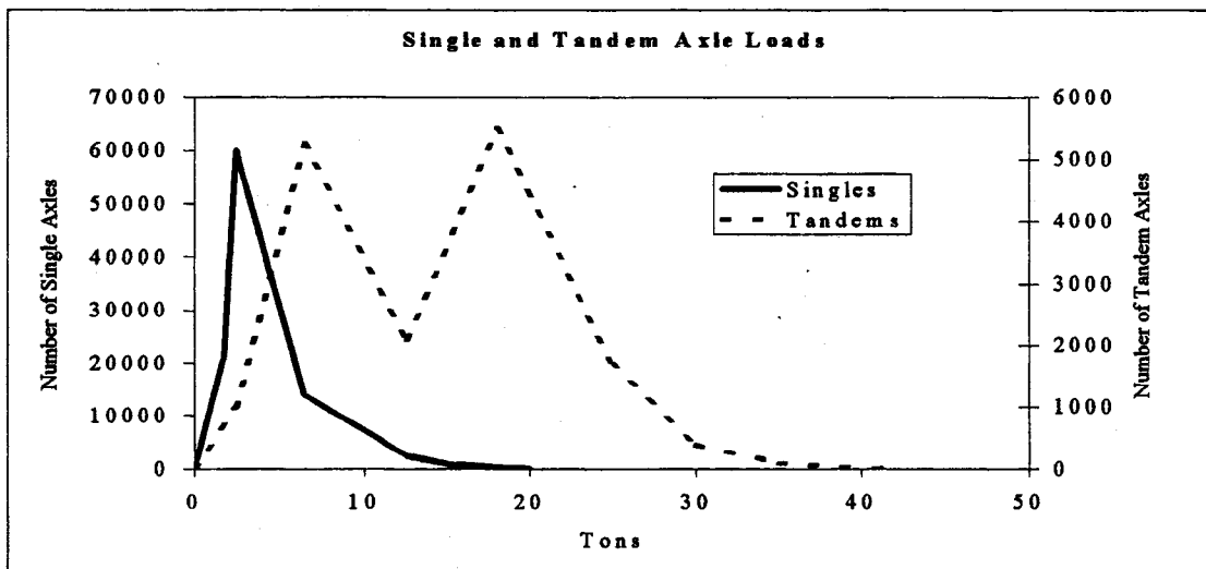
Figure 2.5 Single and Tandem Axle Load Distributions (32).
