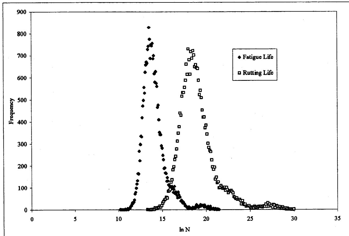
Figure 4.8 Phase III – Steer Axle with Baseline Variability.
