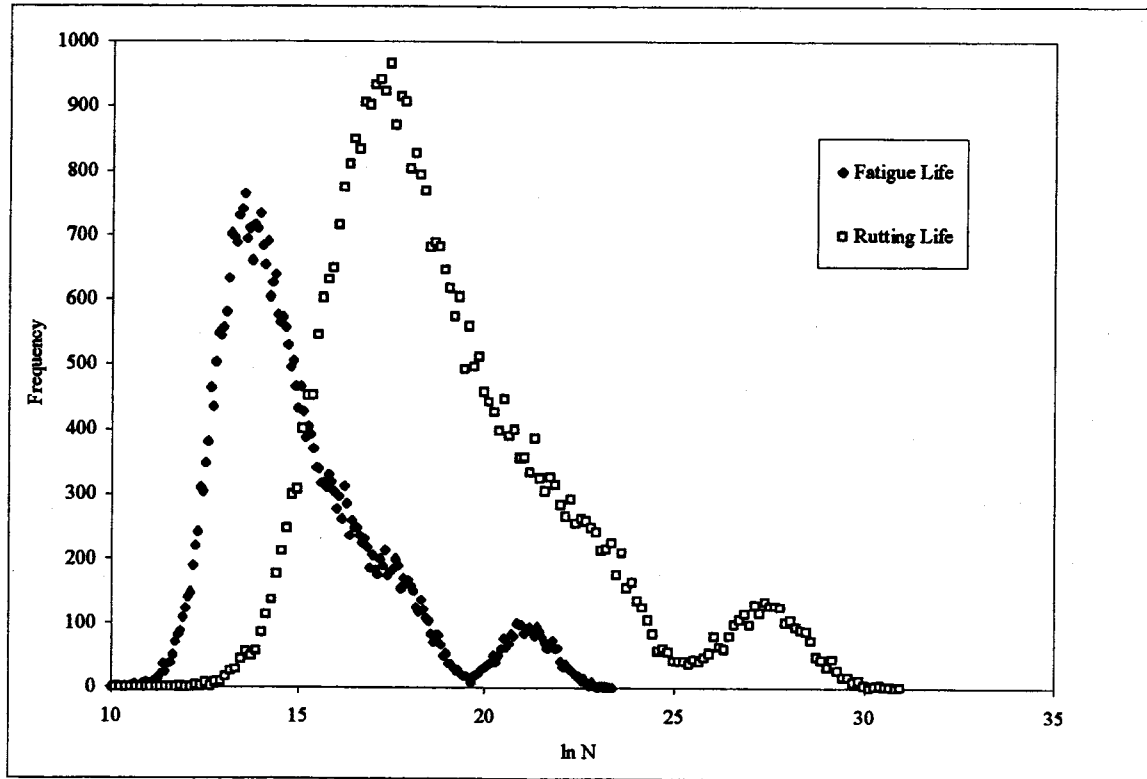
Figure 4.6 Phase III - Single Axle with Baseline Variability.
