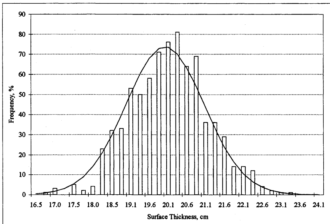
Figure 3.1 Surface Thickness Distribution of Cells 16-22 at Mn/ROAD.
