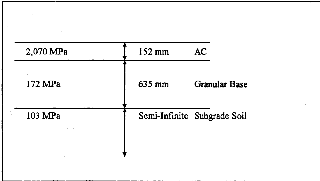
Figure 4.1 Three-Layer Pavement Structure.
