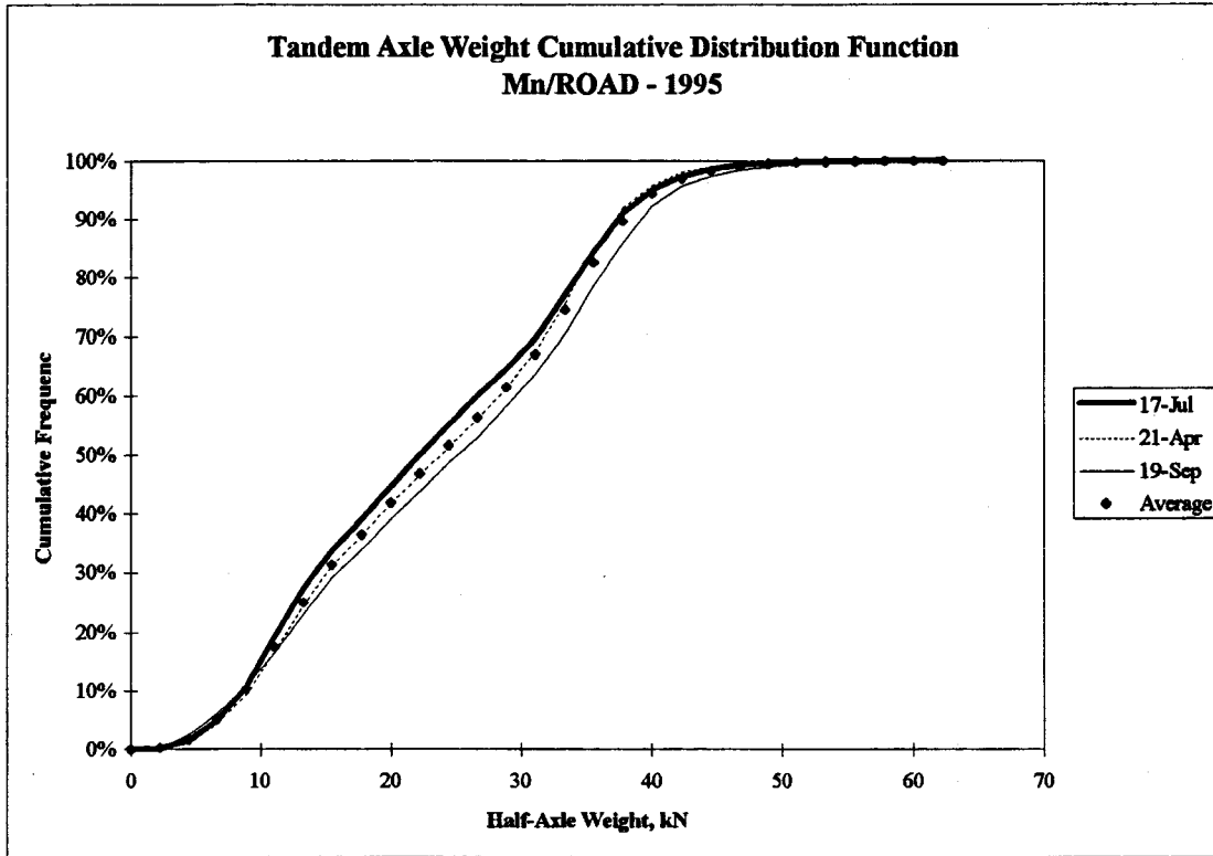
Figure 3.6 Tandem Axle Weight – Cumulative Distribution Function.
