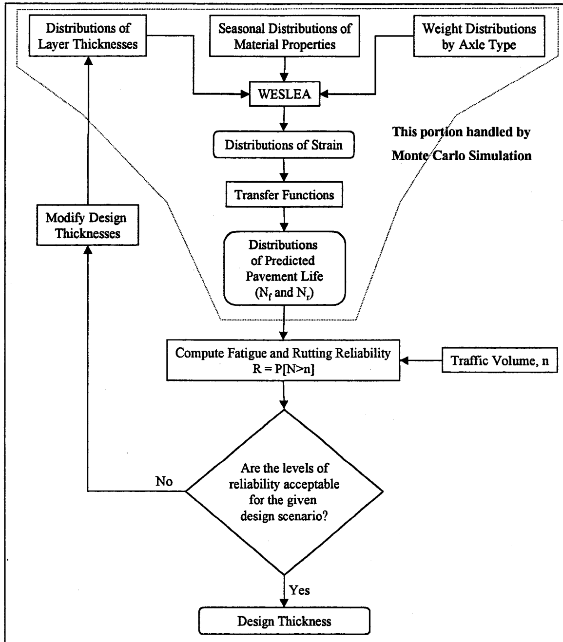
Figure 3.10 Reliability-Based Design Procedure.
