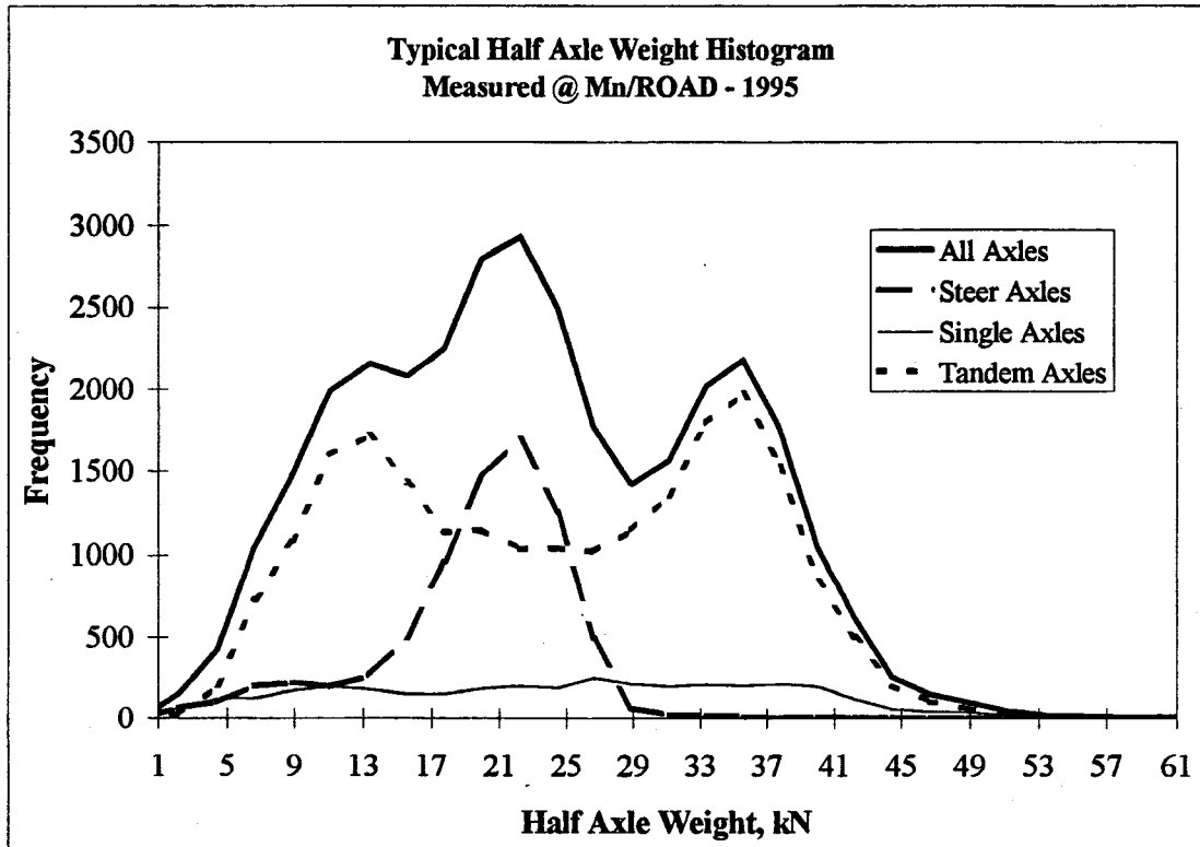
Figure 3.4 Weight Distributions by Axle Configuration.
