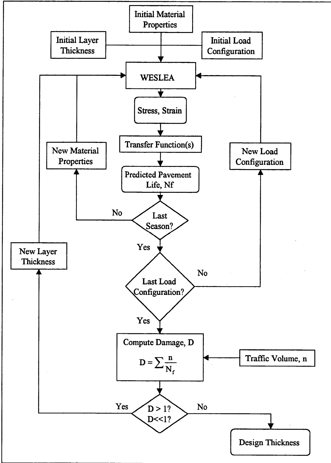
Figure 1.1 Mechanistic-Empirical Design Flow Chart (1).
