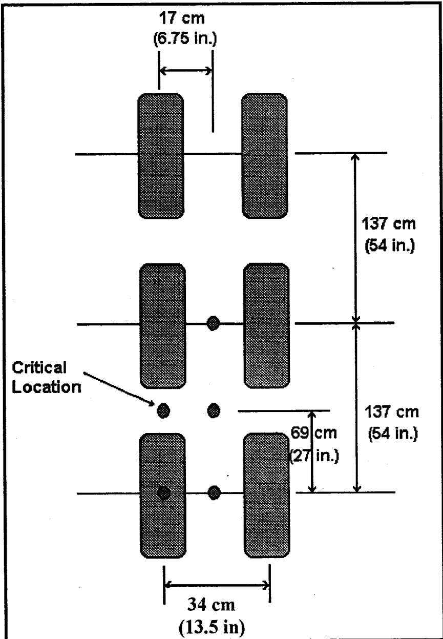
Figure A.8 Tridem Half-Axle Configuration in Plan View.
