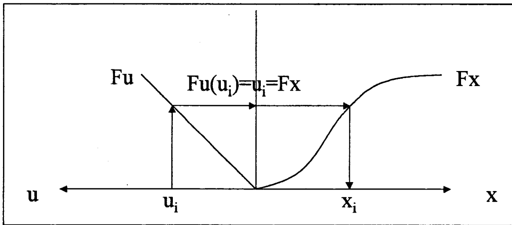
Figure 3.8 Steps 3, 4 and 5 of Monte Carlo Simulation.
