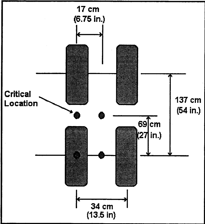
Figure A.7 Tandem Half-Axle Configuration in Plan View.
