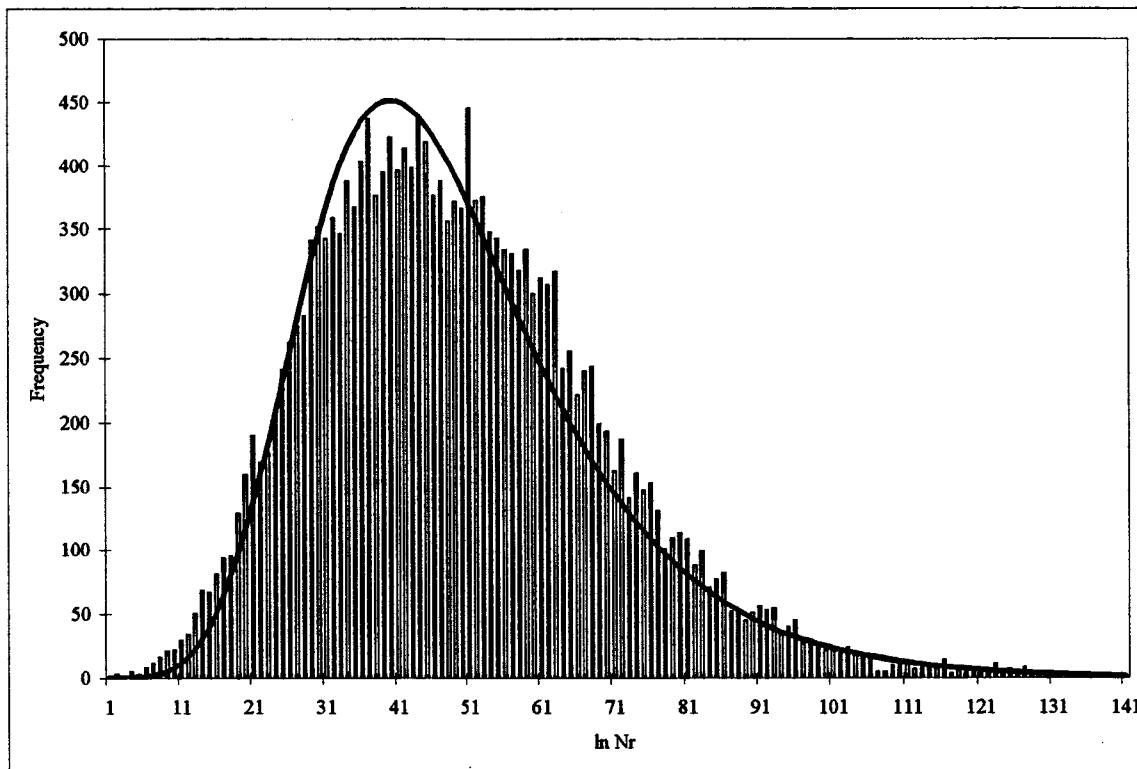
Figure 4.12 Phase III – Rutting Curve Fitting, All Axle Output.
