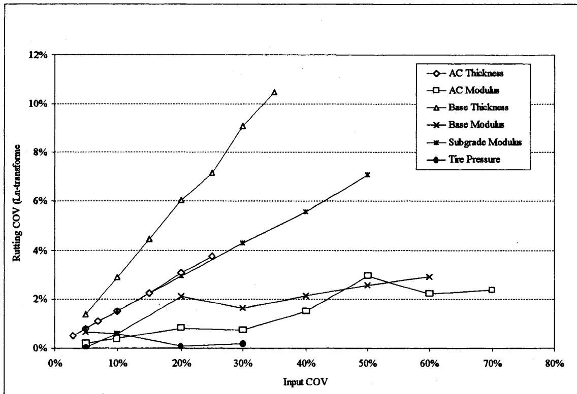
Figure 4.3 Phase I Rutting Variability Comparison.
