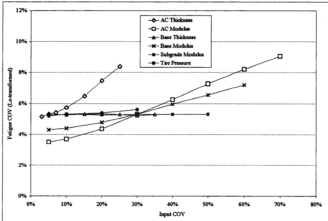
Figure 4.4 Phase II Fatigue Variability Comparison.
