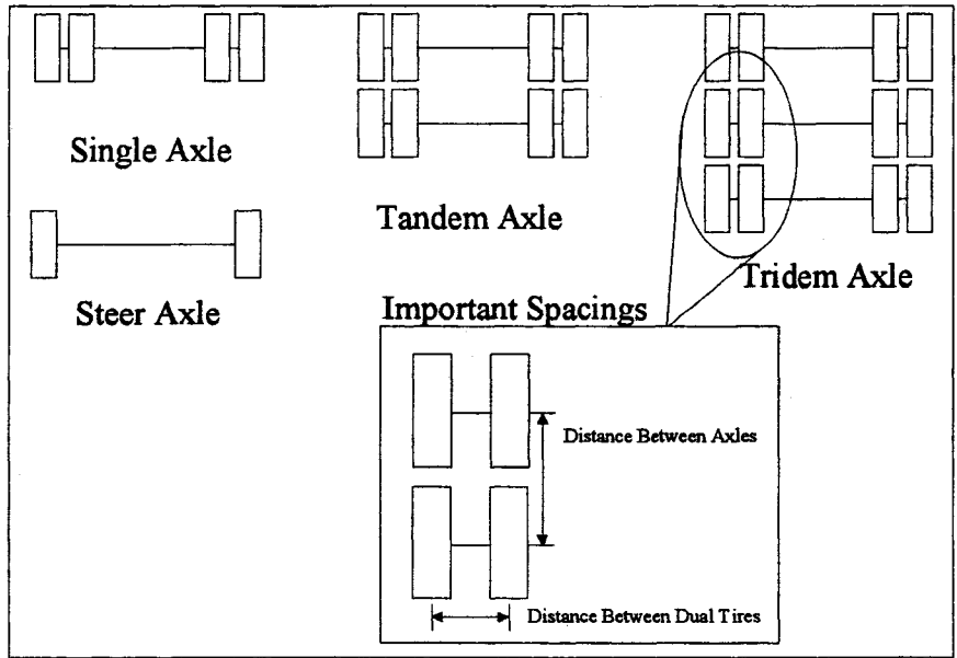
Figure 2.7 Typical Axle Groups and Important Tire Spacings.
