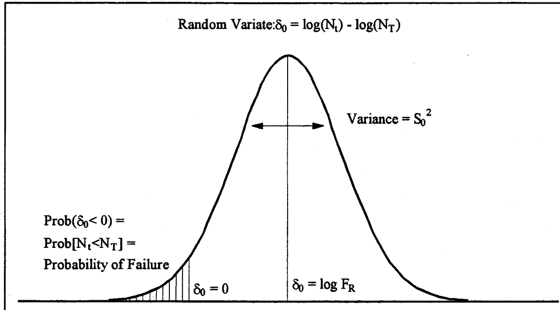
Figure 2.3 Definition of AASHTO Reliability (2).
