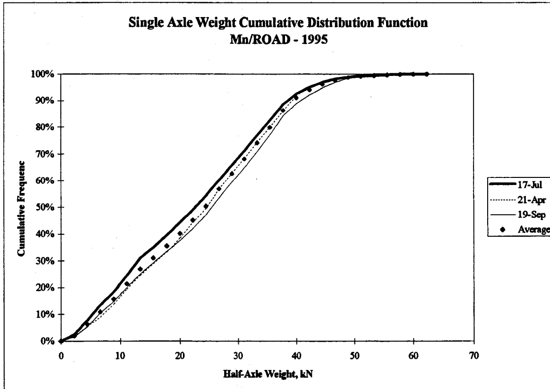
Figure 3.5. Single Axle Weight – Cumulative Distribution Function.
