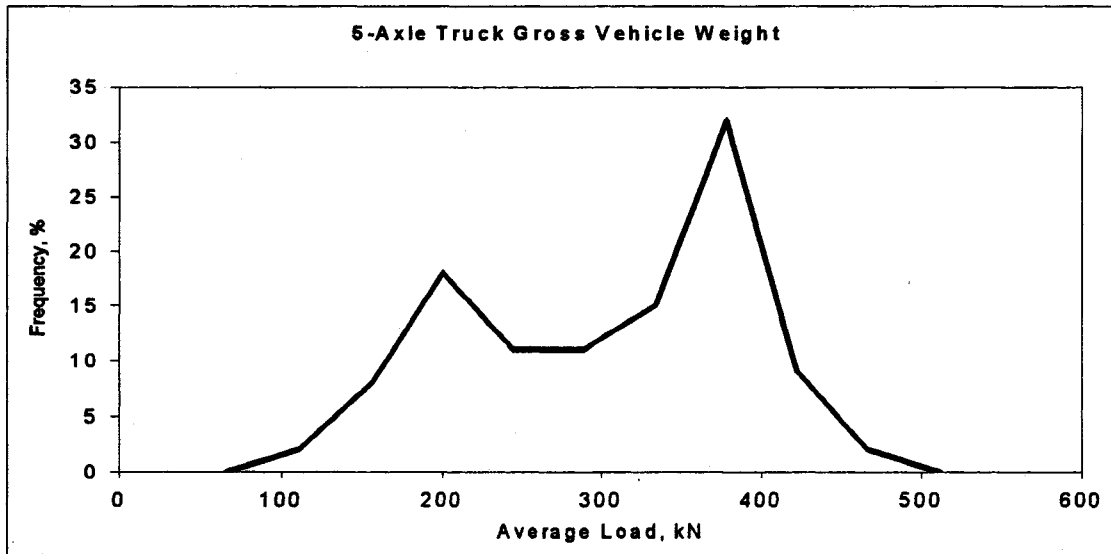
Figure 2.4 Gross Vehicle Weight Distribution (30).
