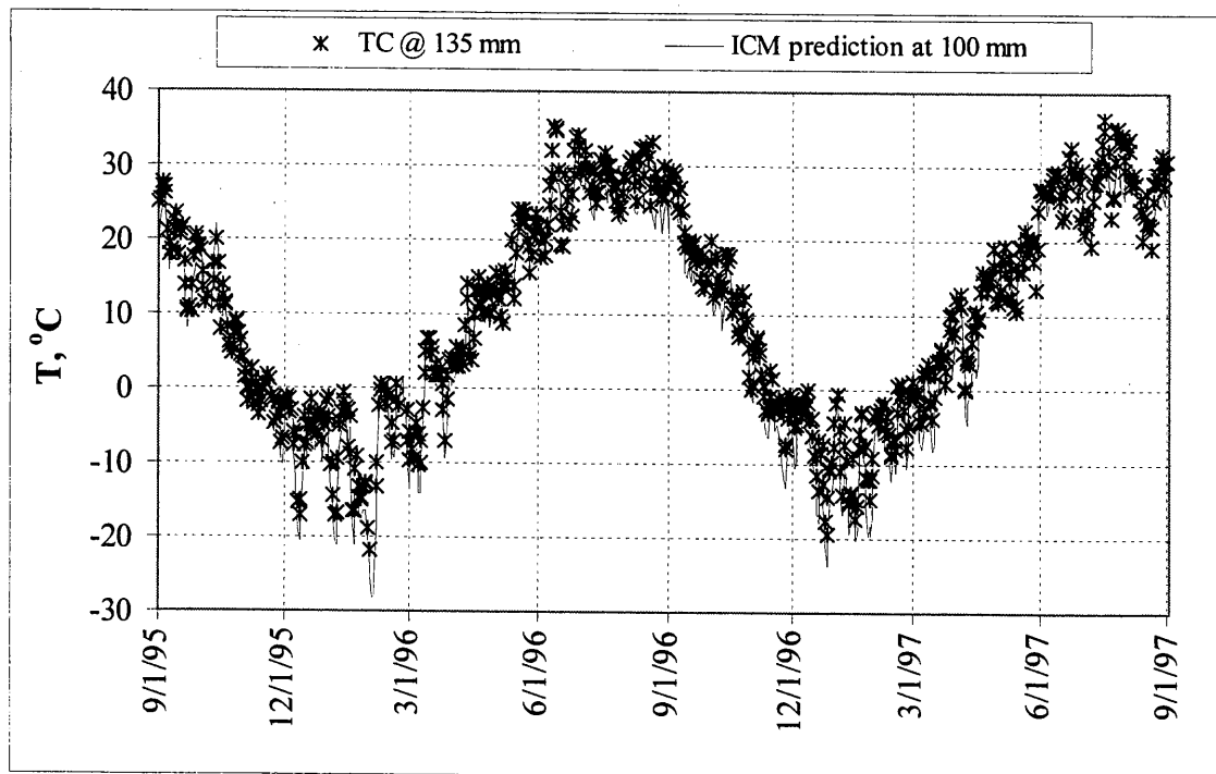
Figure 6.4. Comparison of predicted and measured temperatures in the HMA layer in test section 22.
