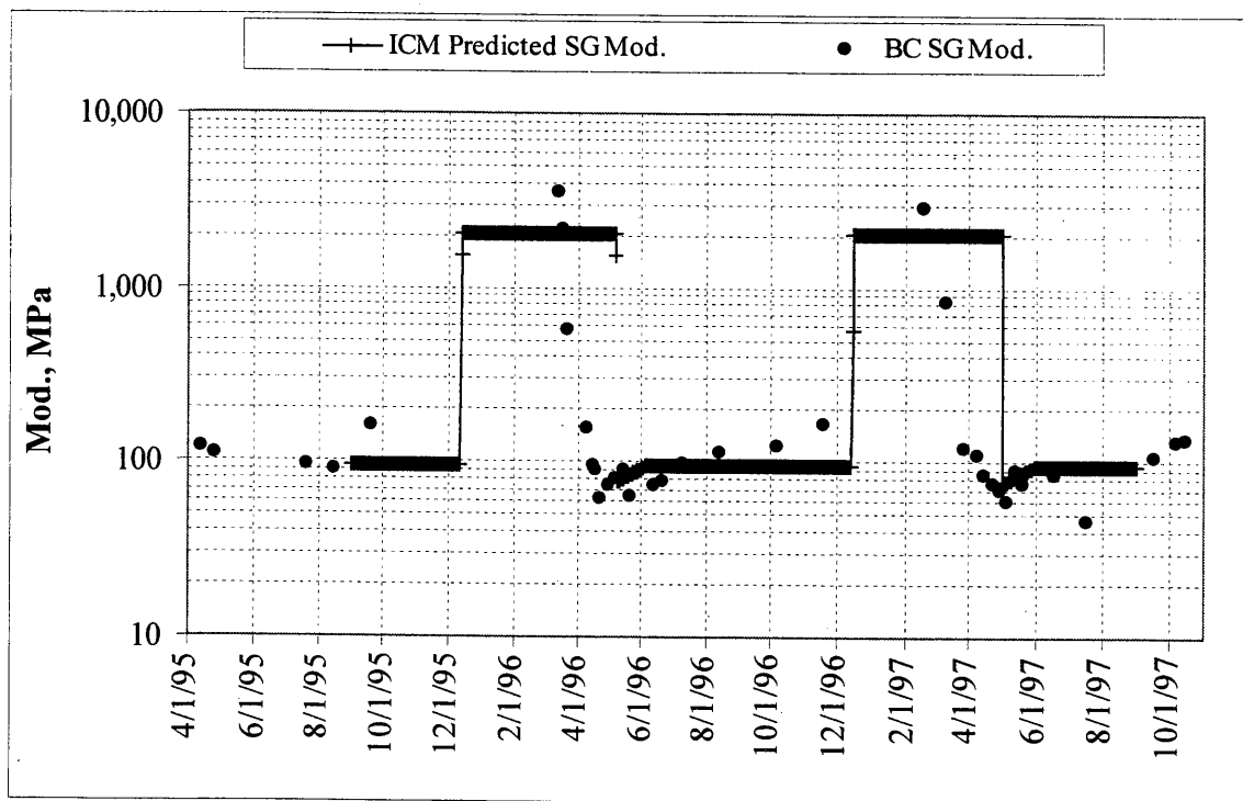
Figure 6.14. Comparison of predicted and backcalculated subgrade layer moduli for test section 17.
