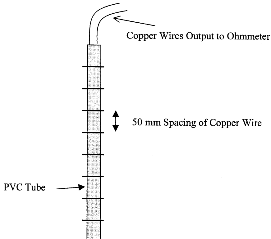
Figure 2.13. Section of a resistivity probe at Mn/ROAD.
