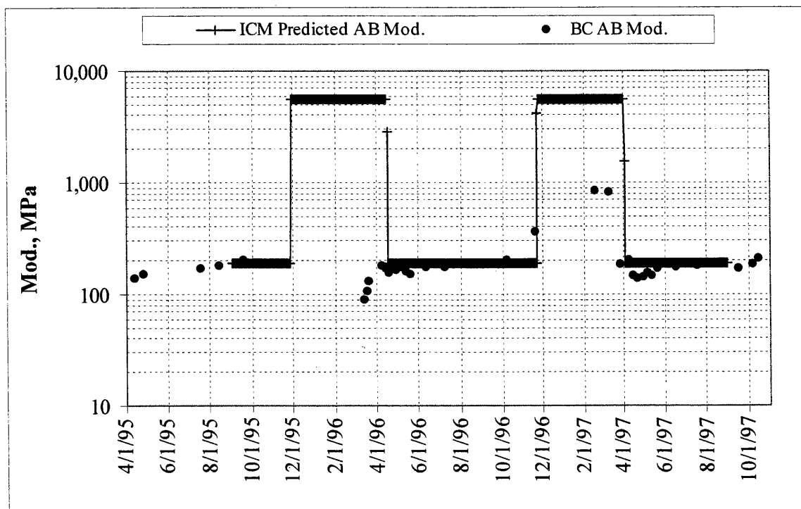
Figure 6.12. Comparison of predicted and backcalculated base layer moduli for test section 17.
