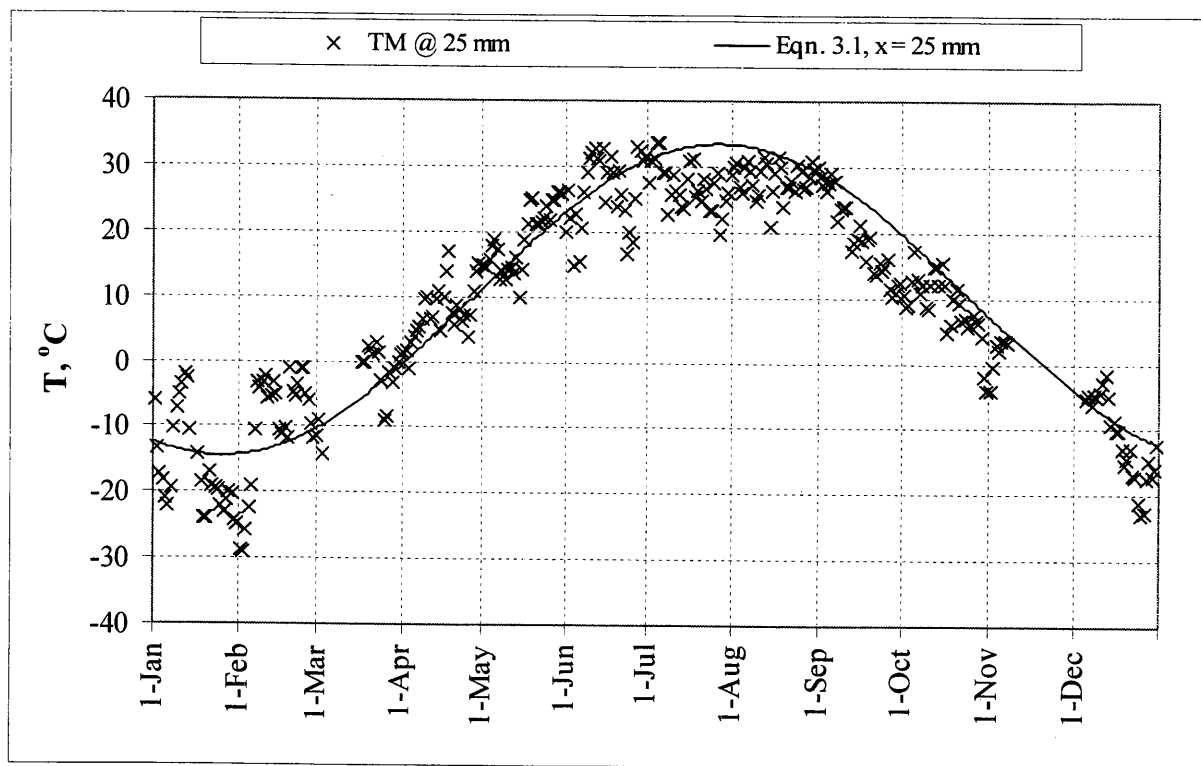
Figure 5.4. Predicted temperature using Equation 3.1 and TM temperature measured at 25 mm in the HMA layer of the Bemidji site (# 27-6251), 1996.
