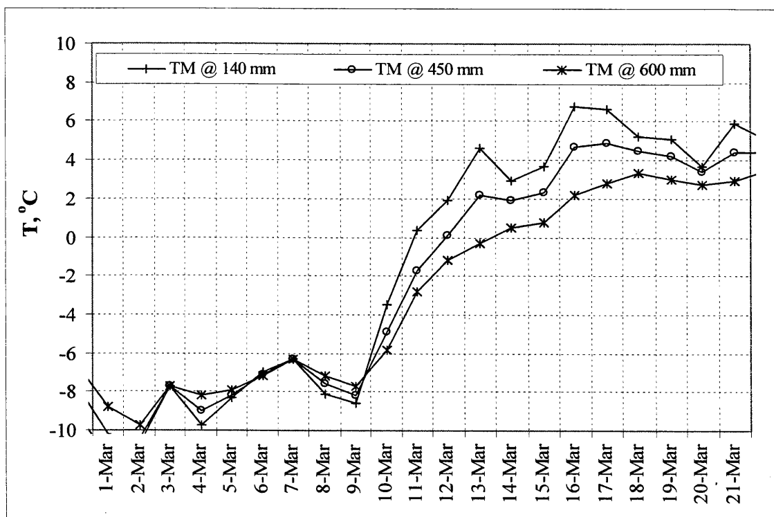
Figure 5.6. TM data from the Bemidji site (#27-6251), March 1995.
