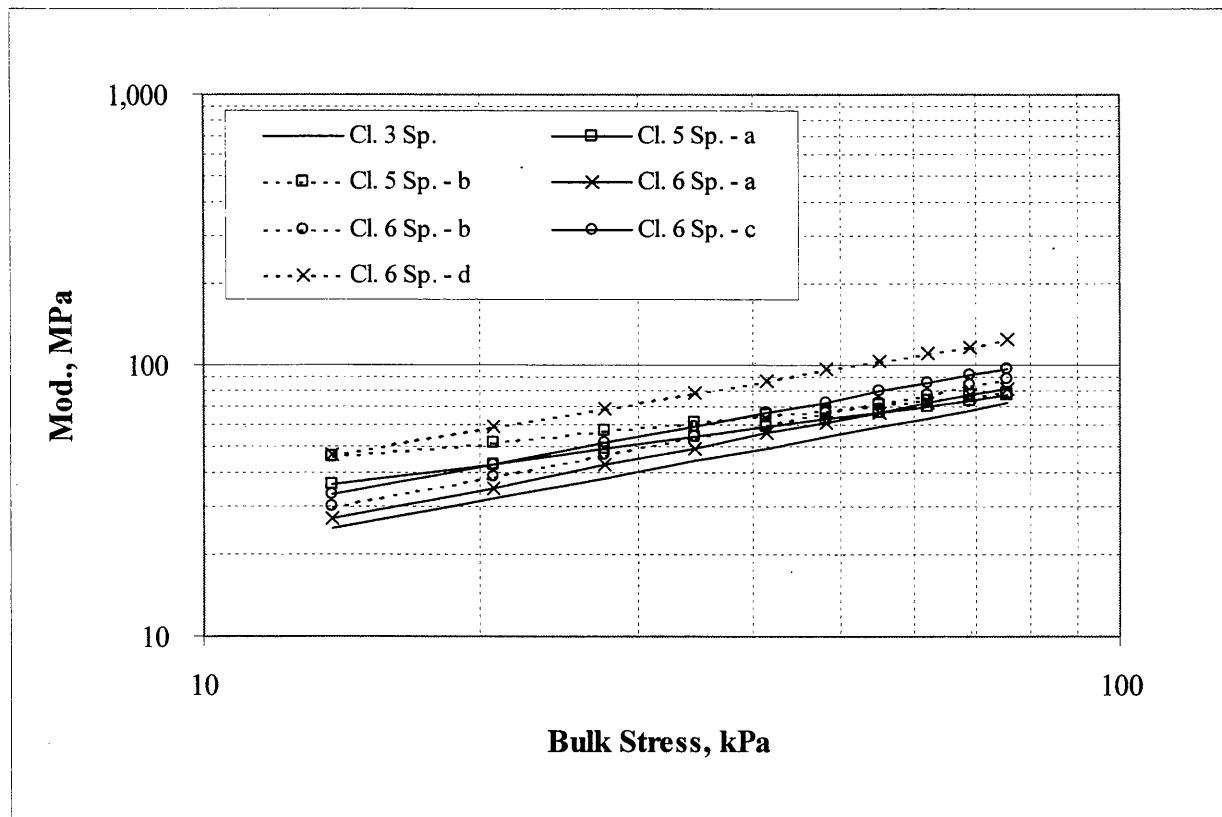
Figure 4.23. Illinois modulus models [50] for Mn/ROAD base materials.
