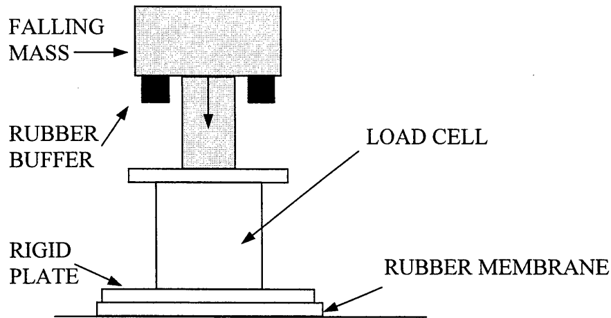
Figure 2.7. Sketch of a falling mass system [27].
