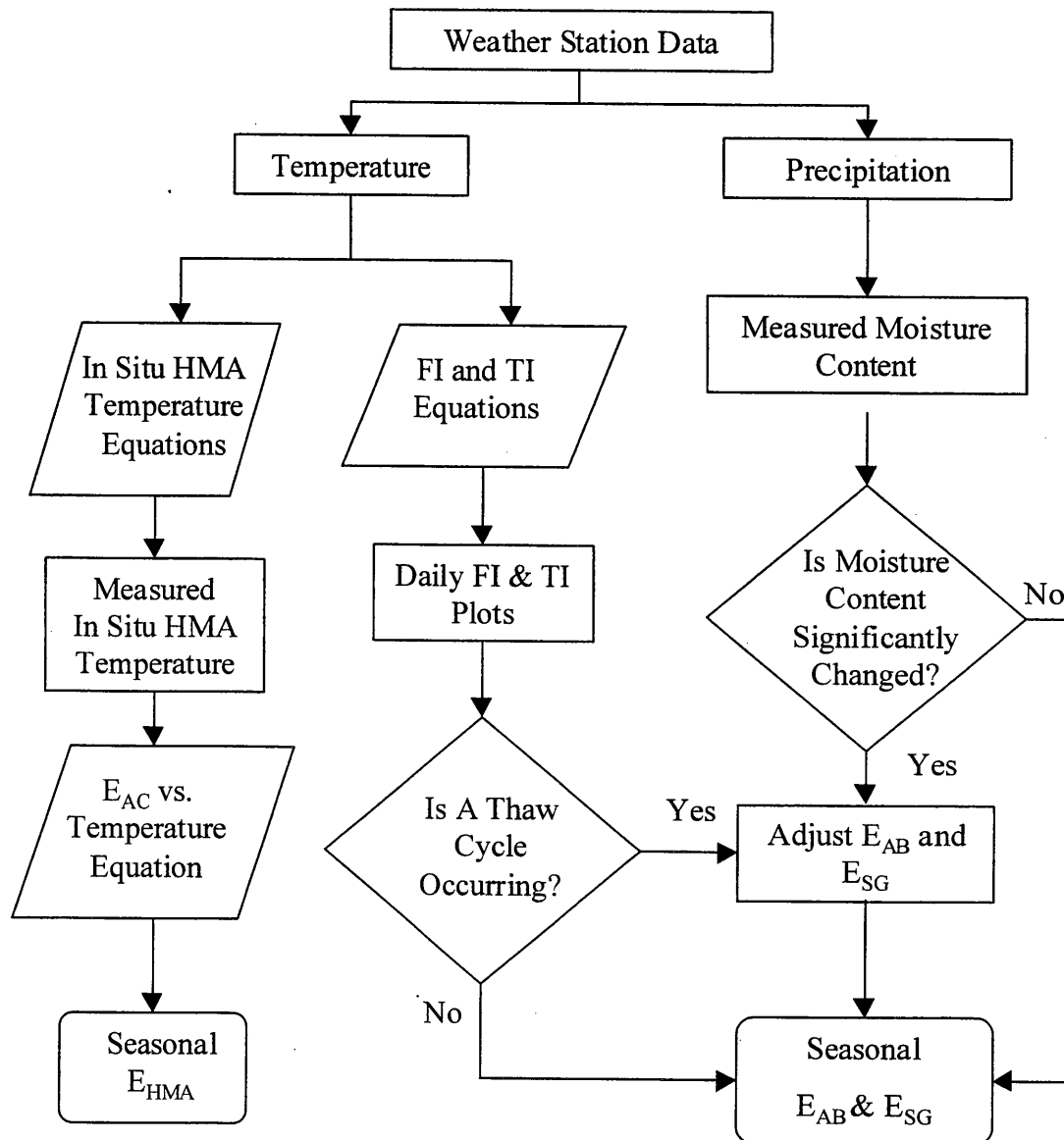
Figure 1. Process used to quantify the relationships between climate factors and pavement material properties for M-E design.
