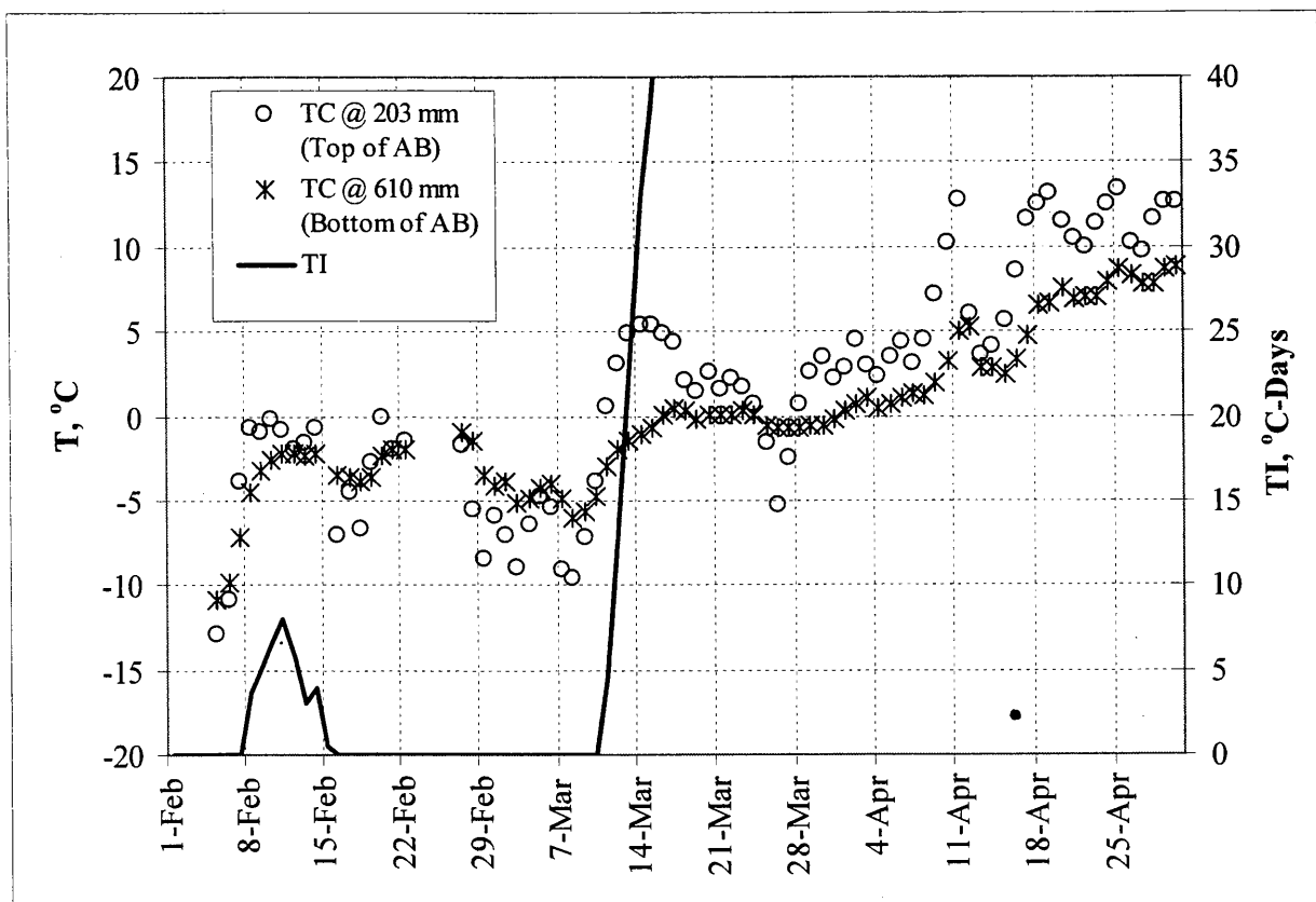
Figure 4.13. TI and TC data in test section 22, Cl. 6 Sp. base, spring 1996.
