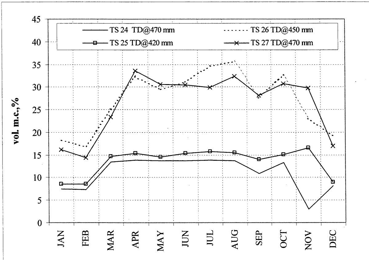
Figure 4.11. Moisture content of different subgrade materials at similar depths.
