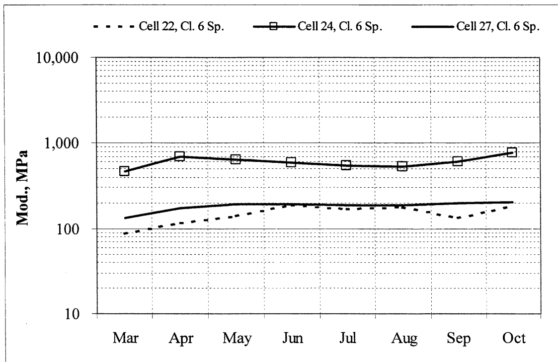
Figure 4.22. Seasonal variations in Cl. 6 Sp. moduli, 1996, test sections 22, 24 and 27.
