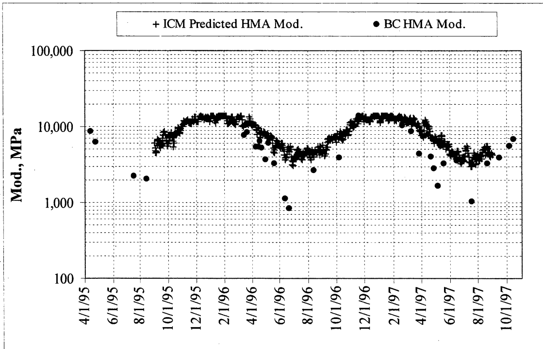
Figure 6.10. Comparison of predicted and backcalculated HMA moduli in test section 17.
