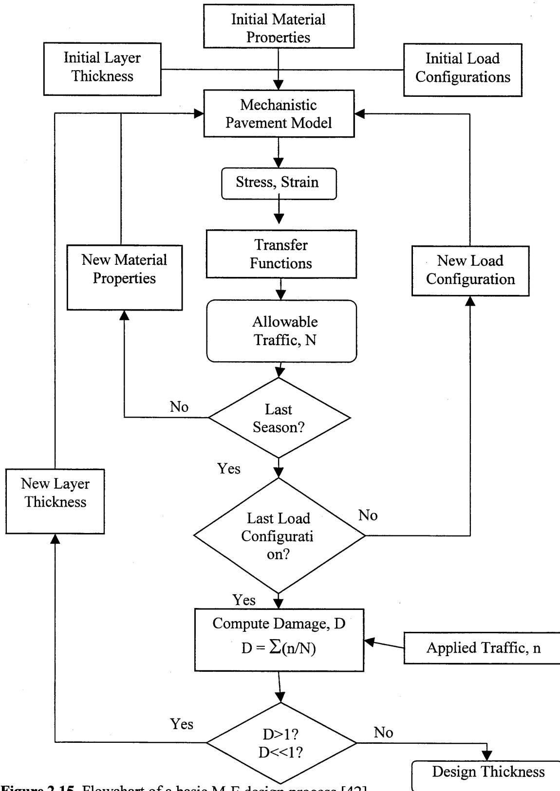
Figure 2.15. Flowchart of a basic M-E design process [42].
