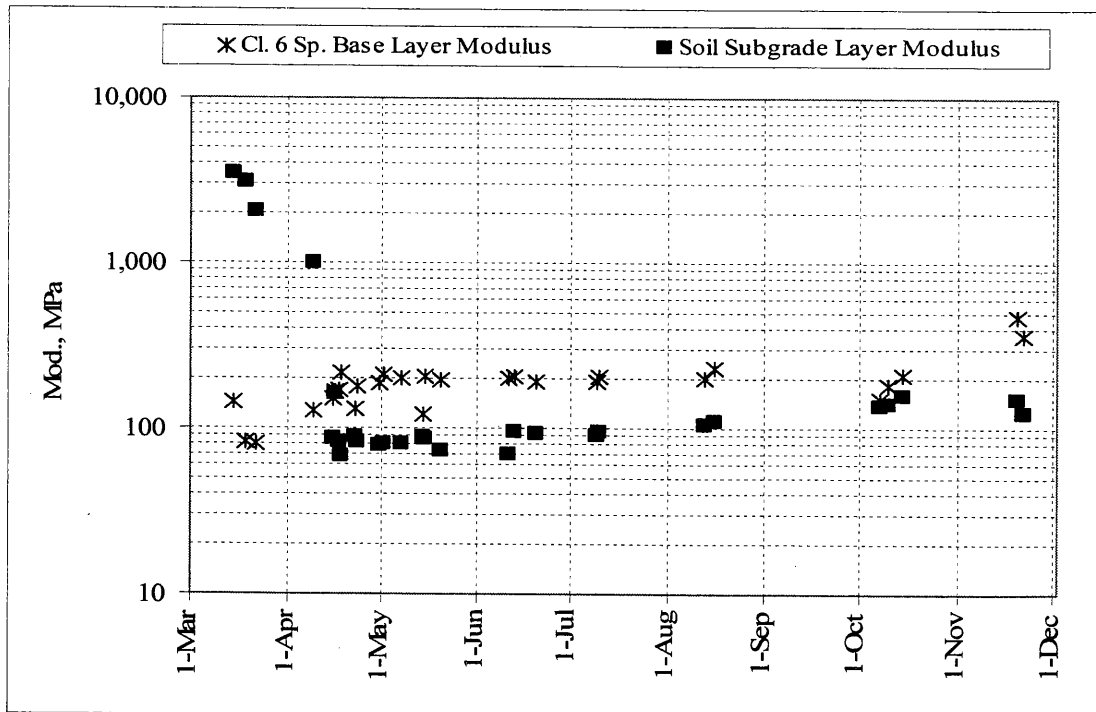
Figure 4.20. Cl. 6 Sp. aggregate base and subgrade moduli in 1996 in test section 22.
