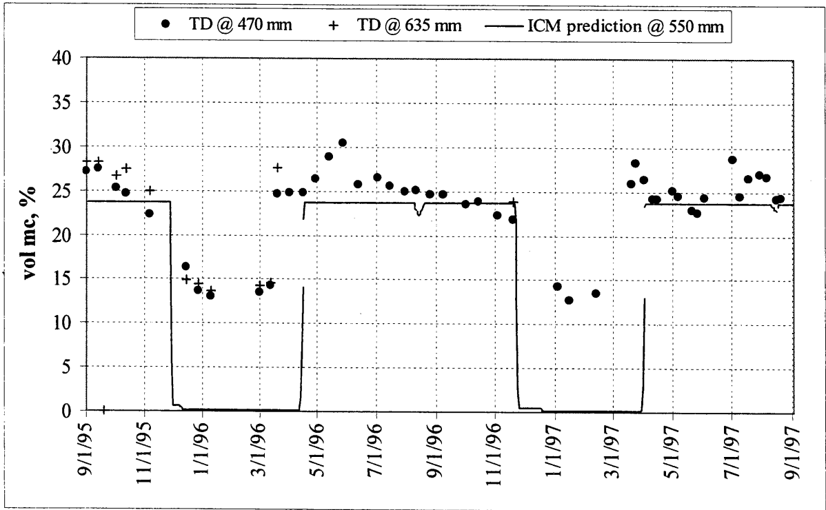
Figure 6.6. Comparison between predicted and measured volumetric moisture content in the base layer of test section 17.
