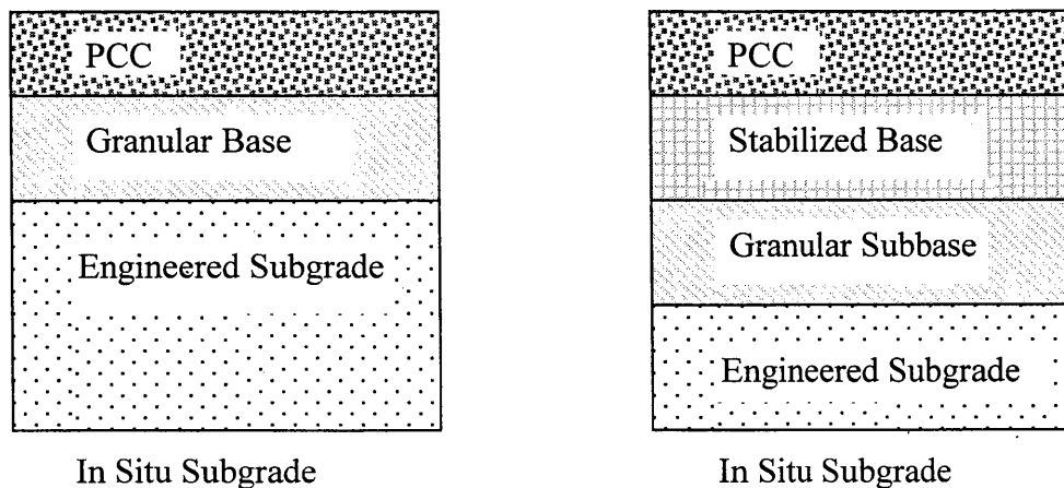
Figure 2.4. Typical cross-section of a rigid pavement.
