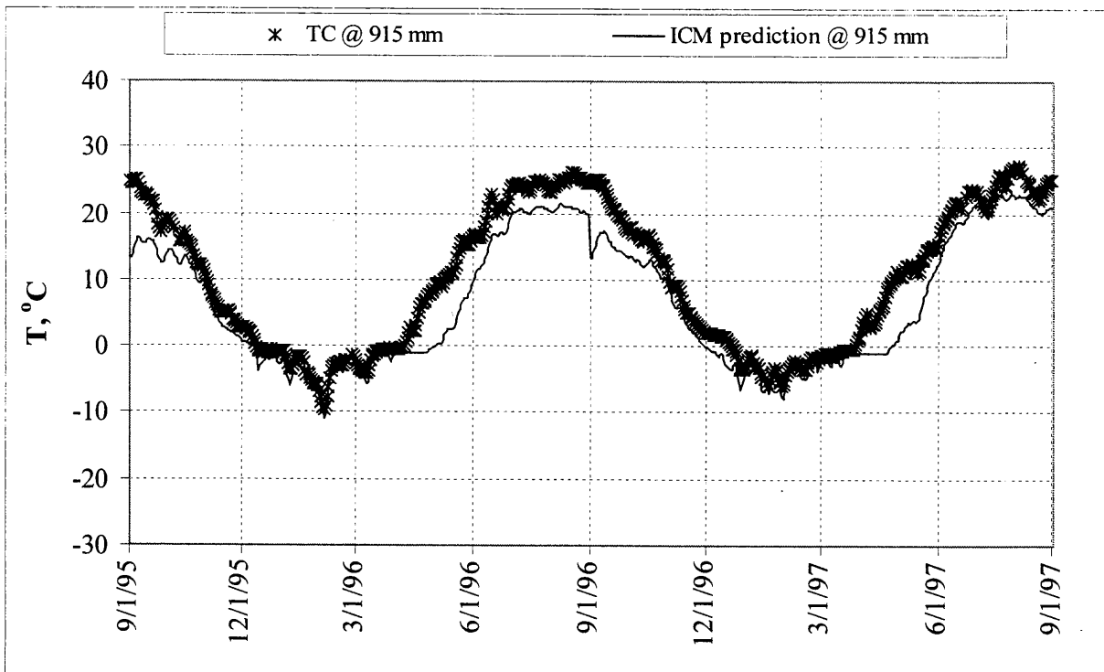
Figure 6.3. Comparison of predicted and measured temperatures in the Cl. 3 Sp. base layer in test section 17.
