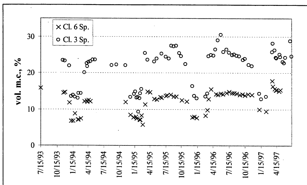
Figure 4.12. TDR data at mid-depth of Cl. 3 Sp. and Cl. 6 Sp. base materials in OWP.
