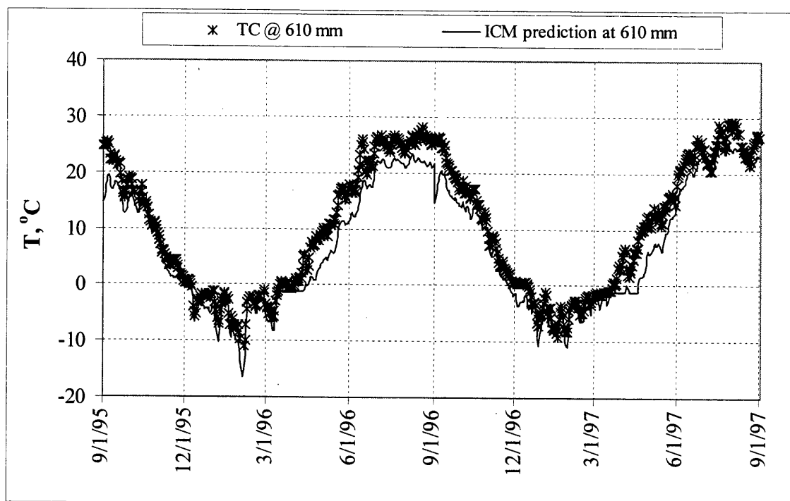
Figure 6.5. Comparison of predicted and measured temperatures in the Cl. 6 Sp. base layer in test section 22.
