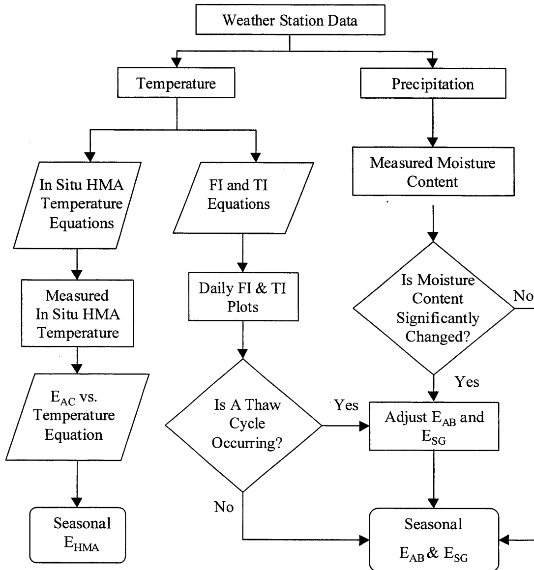
Figure 3.1. Process used to quantify the relationships between climate factors and pavement material properties for M-E design.
