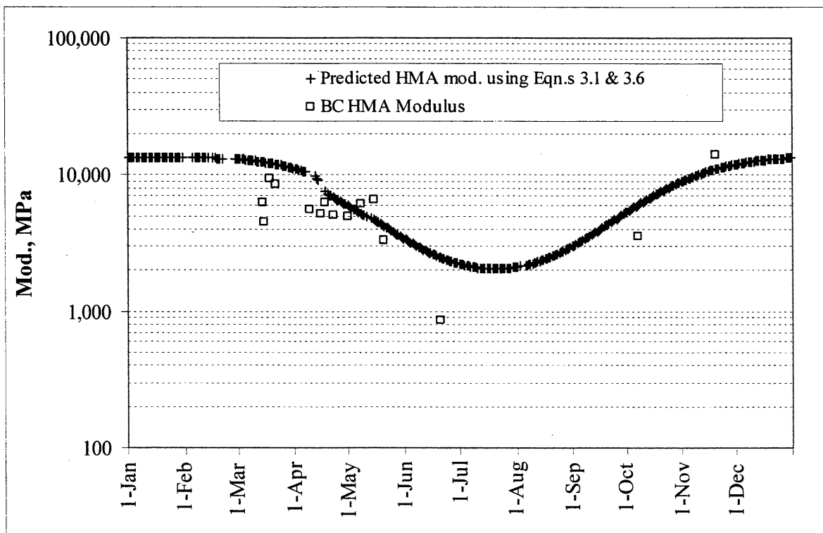
Figure 4.19. A comparison between backcalculated and predicted HMA modulus.
