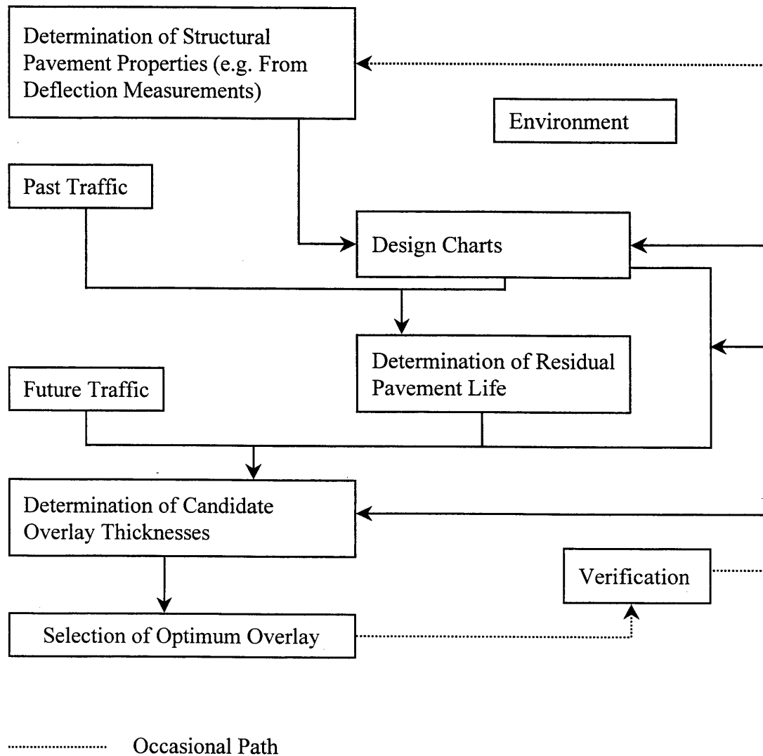
Figure 2.17. Flowchart of Shell overlay design method [47].
