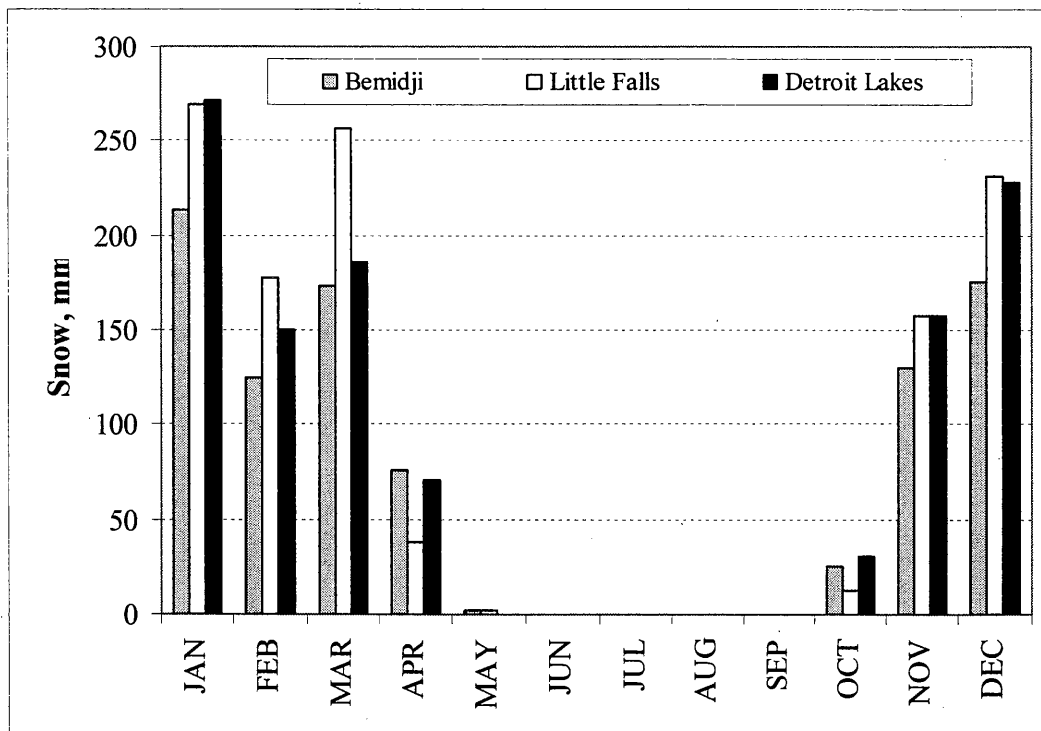
Figure 5.3. 30-year mean monthly snowfall for the LTPP SMP sites in Minnesota.
