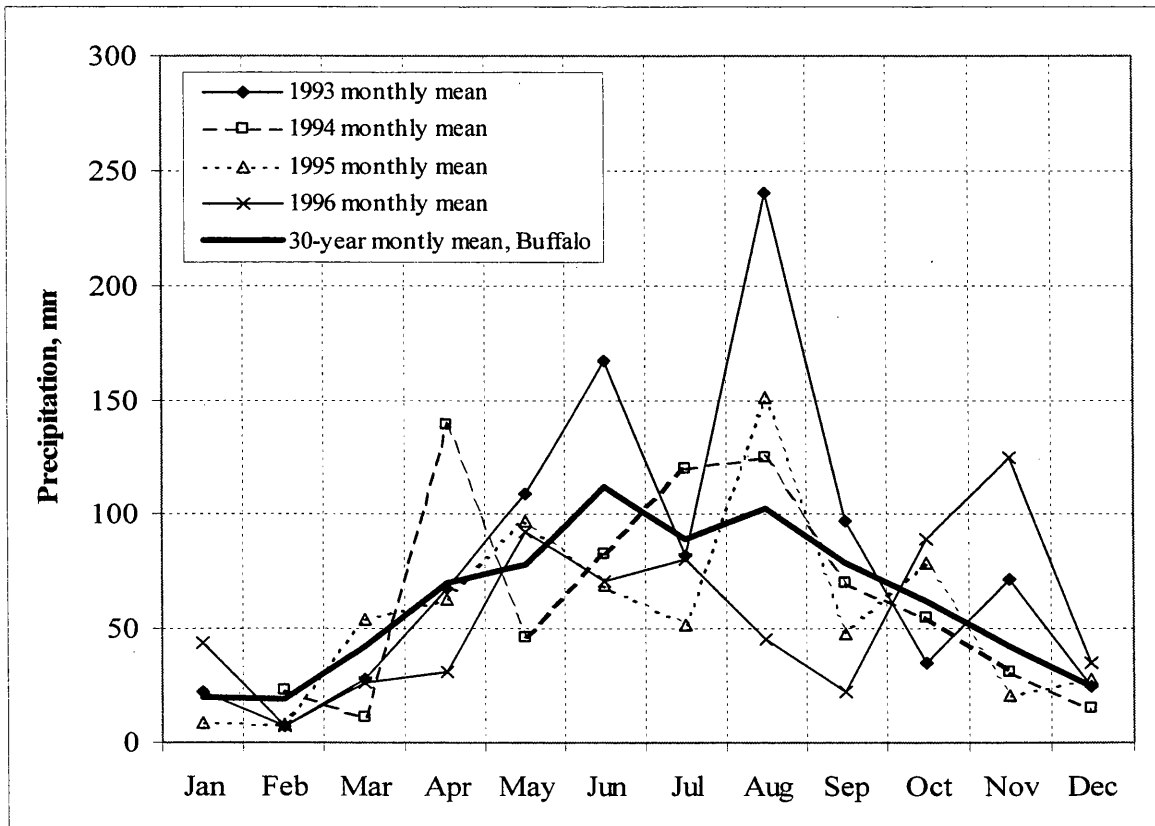
Figure 4.7. Precipitation events at Mn/ROAD between 1993 and 1996 compared to 30-year mean data from Buffalo weather station.
