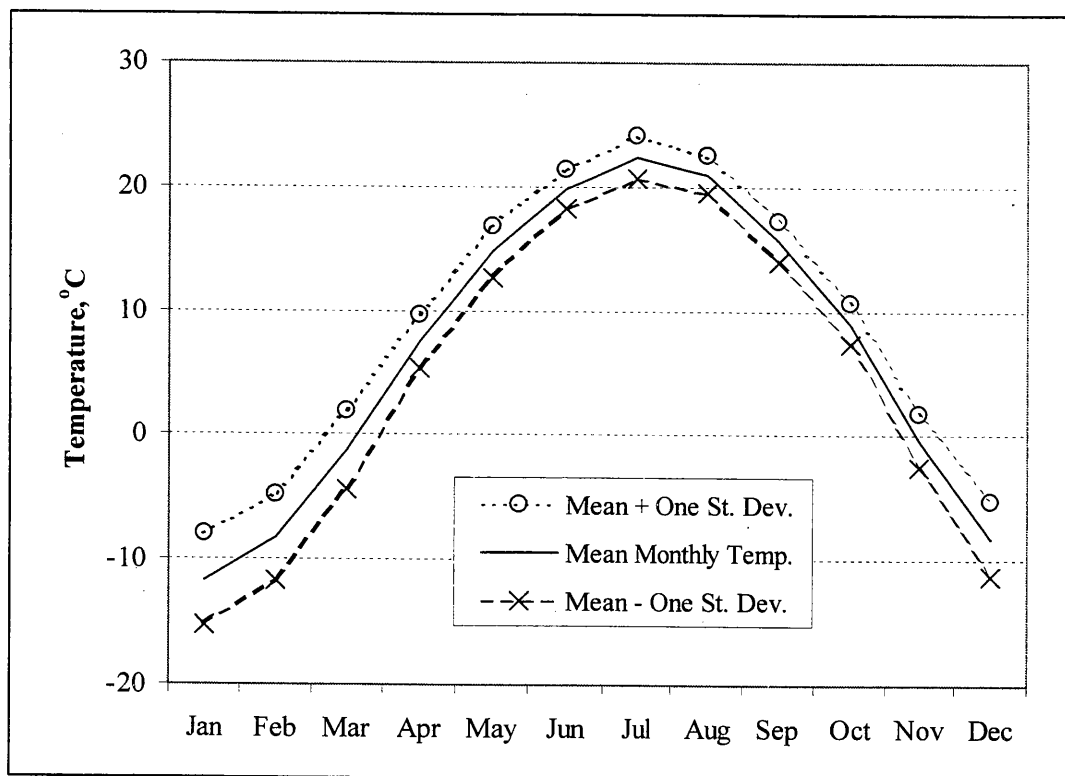
Figure 4.1. 30-year mean monthly temperature data for Buffalo (1965-1995).
