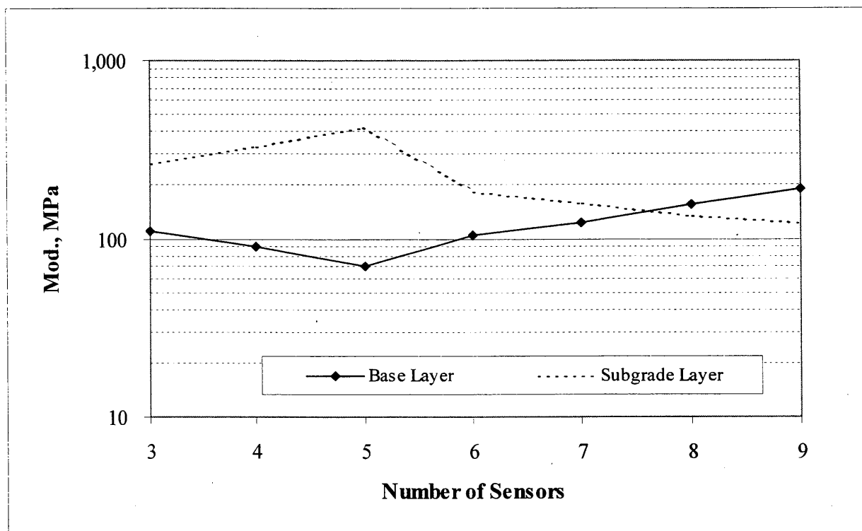
Figure 4.25. Modulus sensitivity for thick pavement, Cl. 5 Sp.
