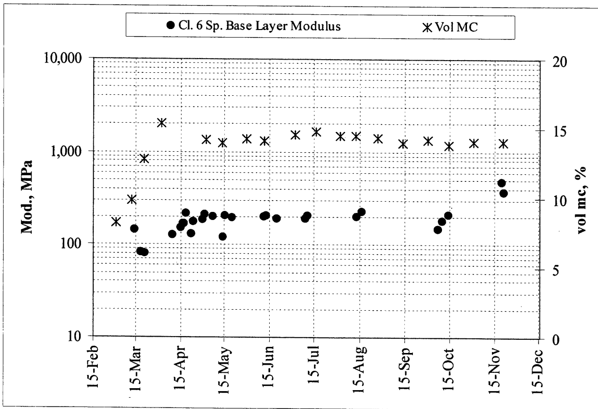
Figure 4.21. Seasonal variations in the base modulus and in the unfrozen volumetric moisture content, test section 22, 1996.
