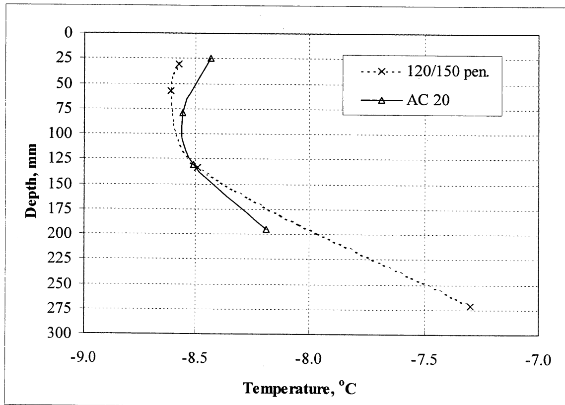
Figure 4.8. Mean monthly thermal gradient in January 1996 for test sections 19 (AC 20) and 20 (120/150 pen.).
