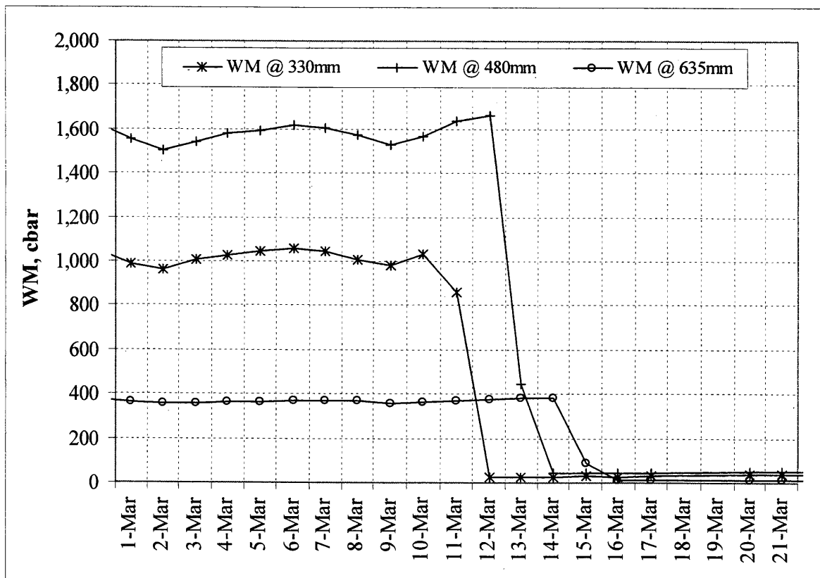
Figure 5.8. Mn/ROAD test section 17 spring 1995 frost depth data from WM sensors at 330 mm, 480 mm and 635 mm.
