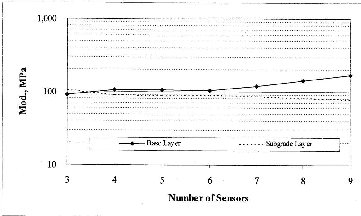
Figure 4.26. Modulus sensitivity for thin pavement, Cl. 5 Sp.
