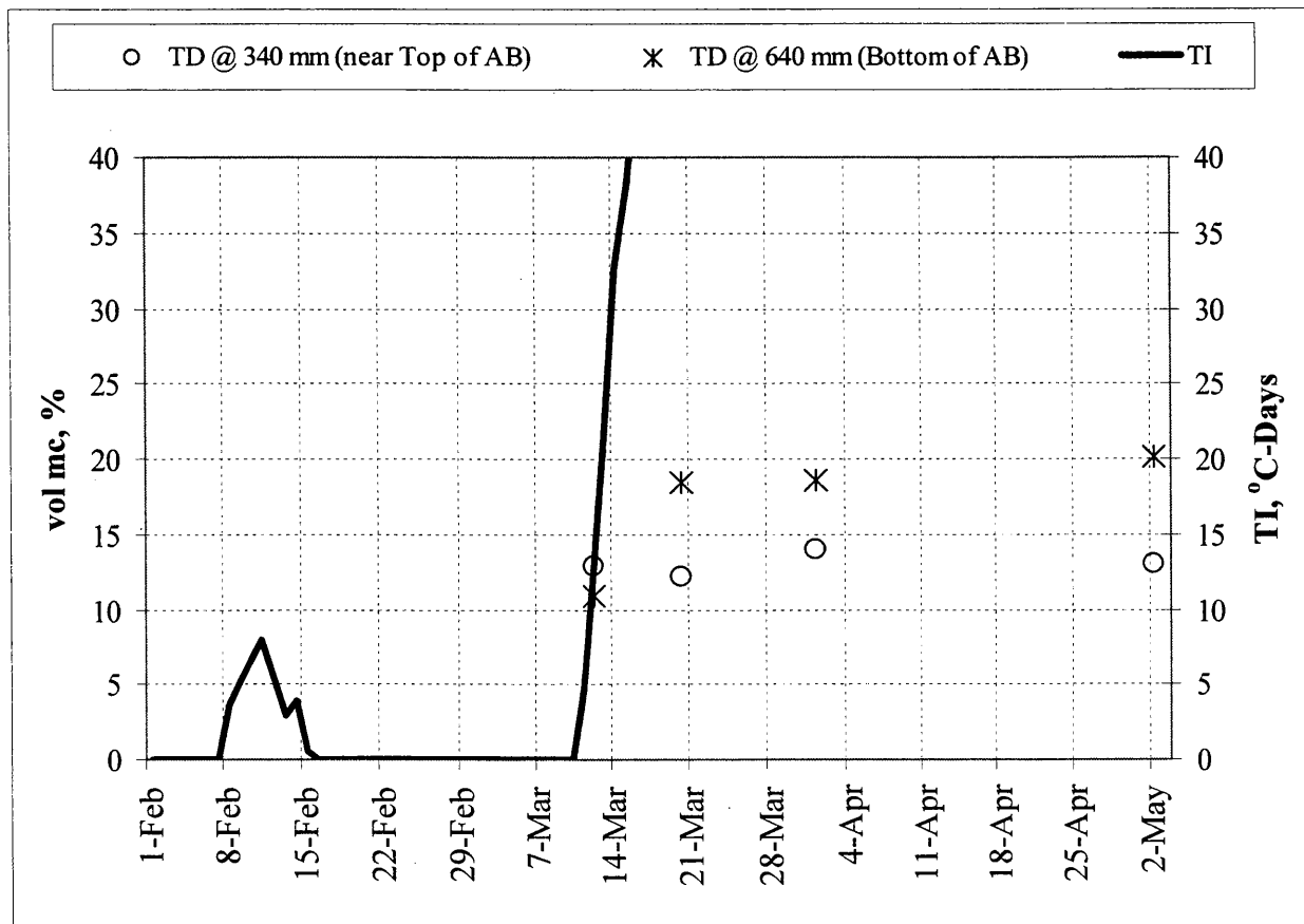
Figure 4.15. TI and TDR data for Cl. 6 Sp. base, spring 1996.
