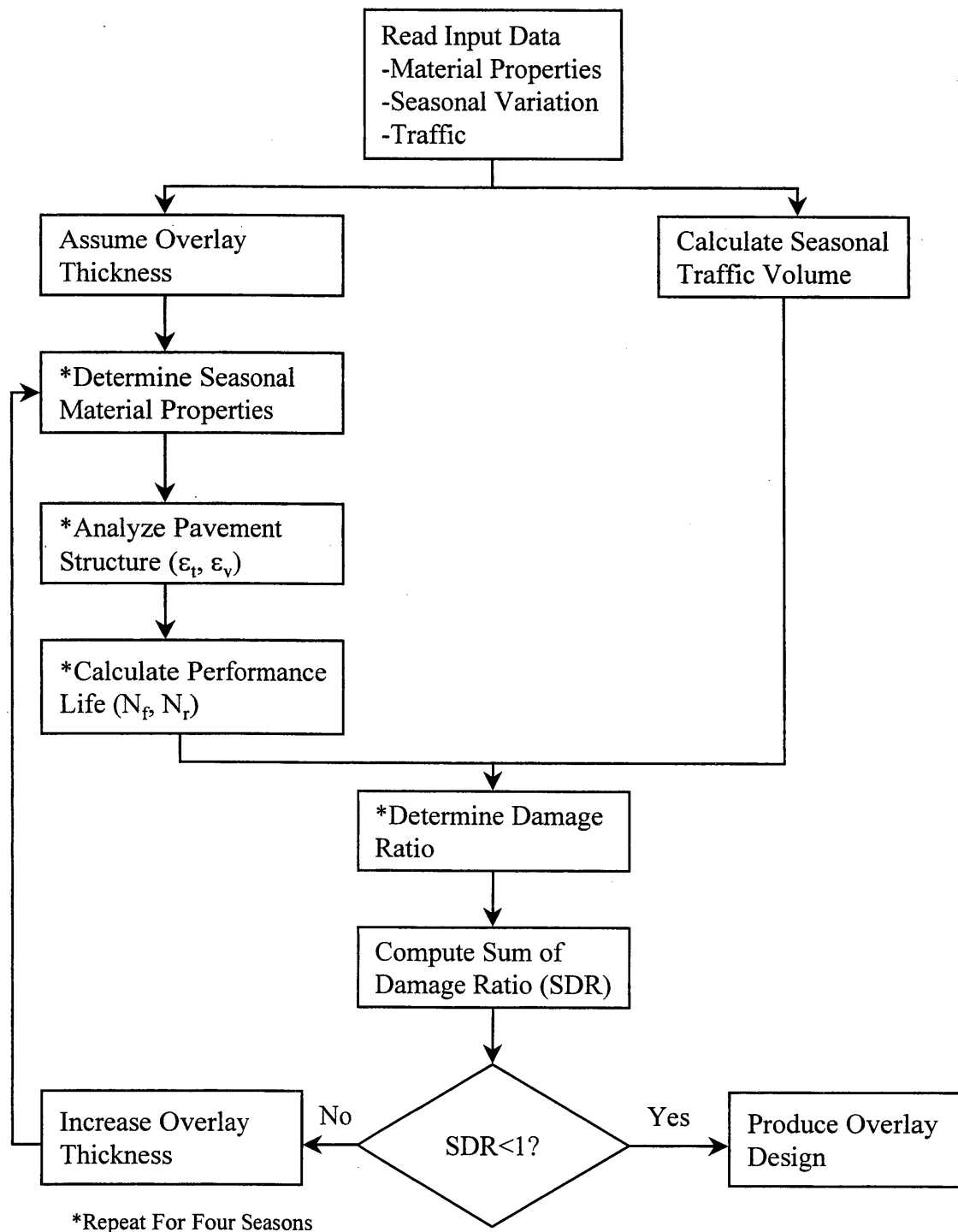
Figure 2.16. WSDOT overlay design flow chart [12].
