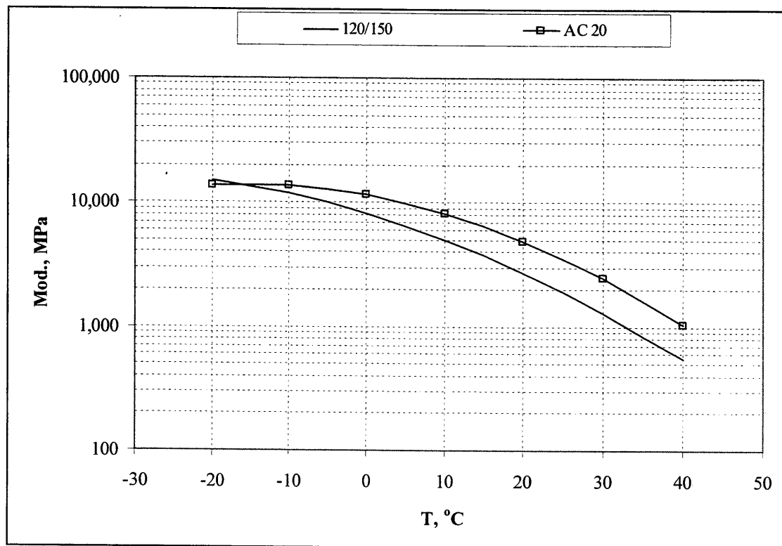
Figure 4.16. Equation 3.6 used to estimate HMA modulus from temperature data.
