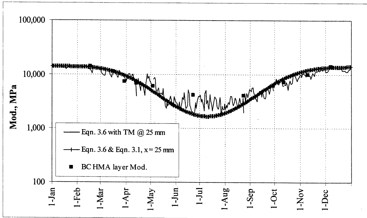
Figure 5.9. Bemidji site (#27-6251) predicted and backcalculated HMA modulus, 1994, using Equations 3.1 and 3.6.
