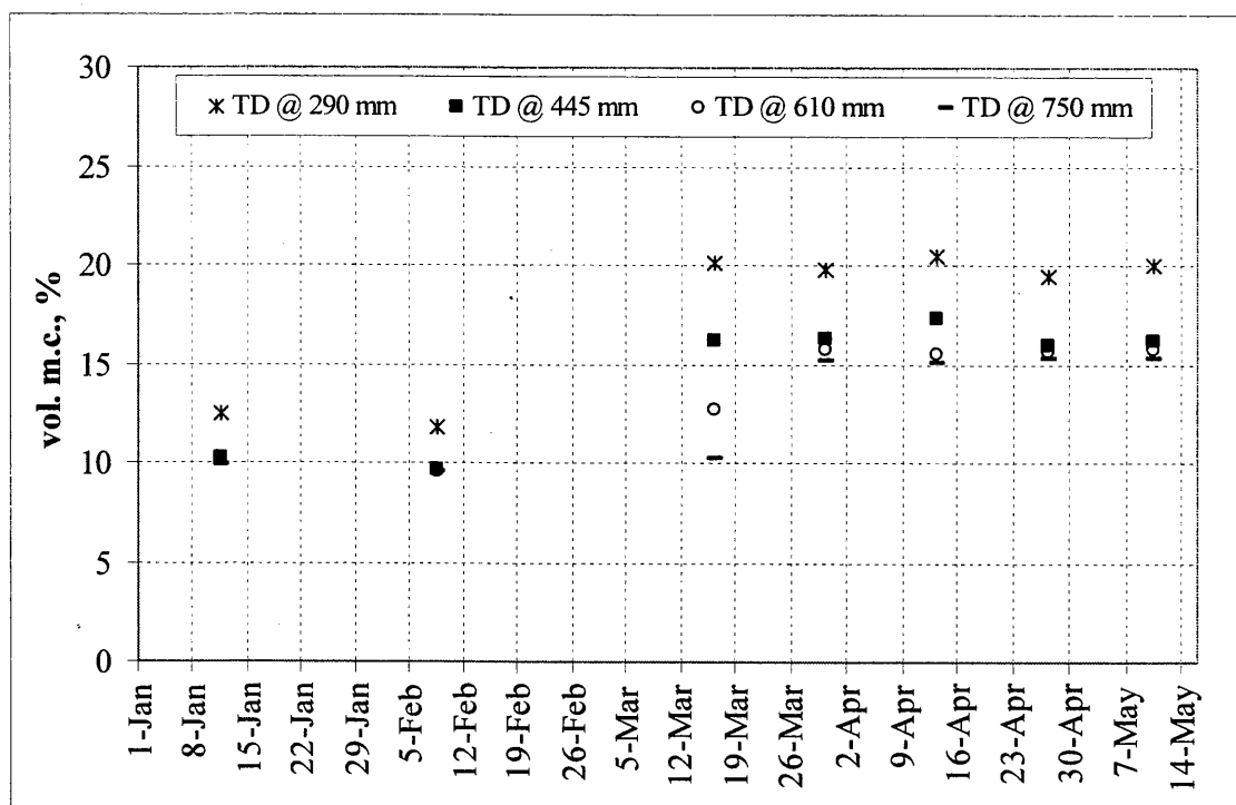
Figure 5.7. TDR data from the Bemidji site (#27-6251) beginning January 1, 1995.
