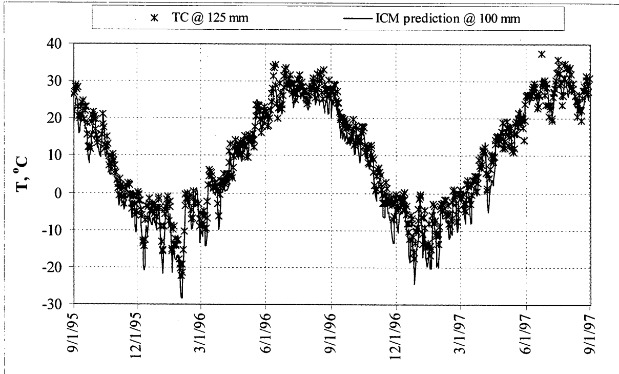
Figure 6.2. Comparison between predicted and the measured temperature in the HMA layer in test section 17.
