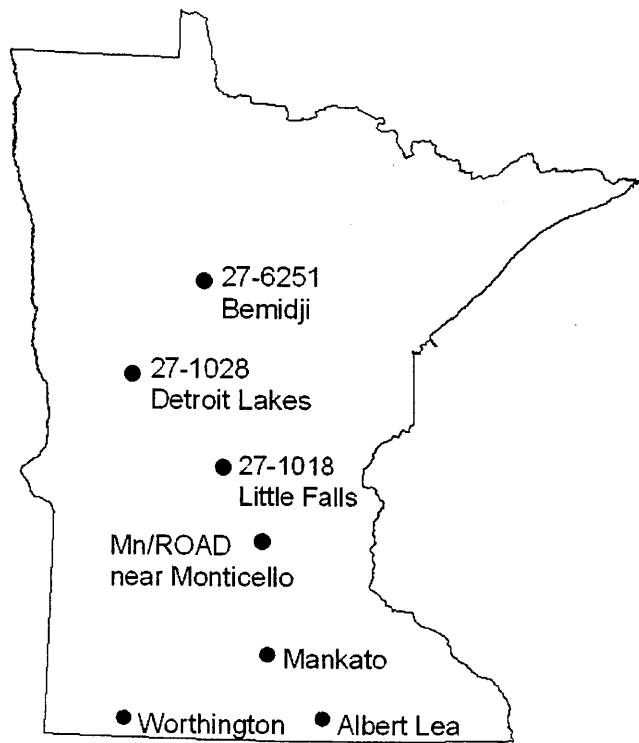
Figure 5.1. Location in Minnesota of the three LTPP SMP sites, Mn/ROAD, and the other weather stations used in this study.
