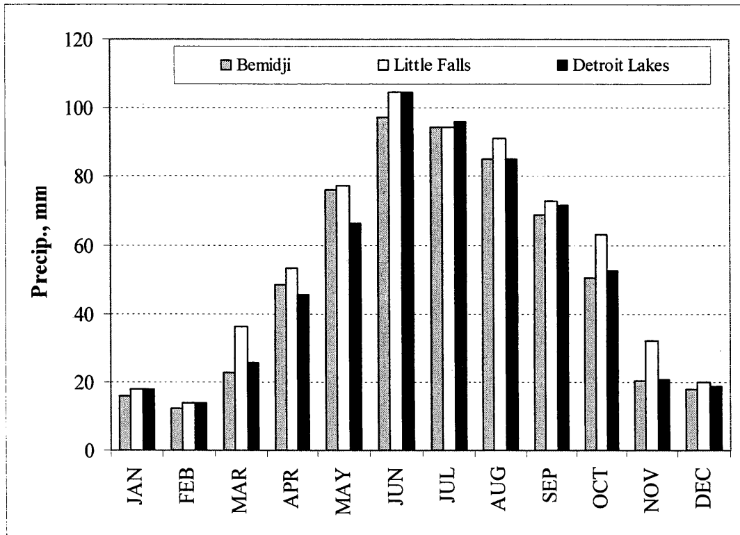
Figure 5.2. 30-year mean monthly precipitation events for the LTPP SMP sites in Minnesota.
