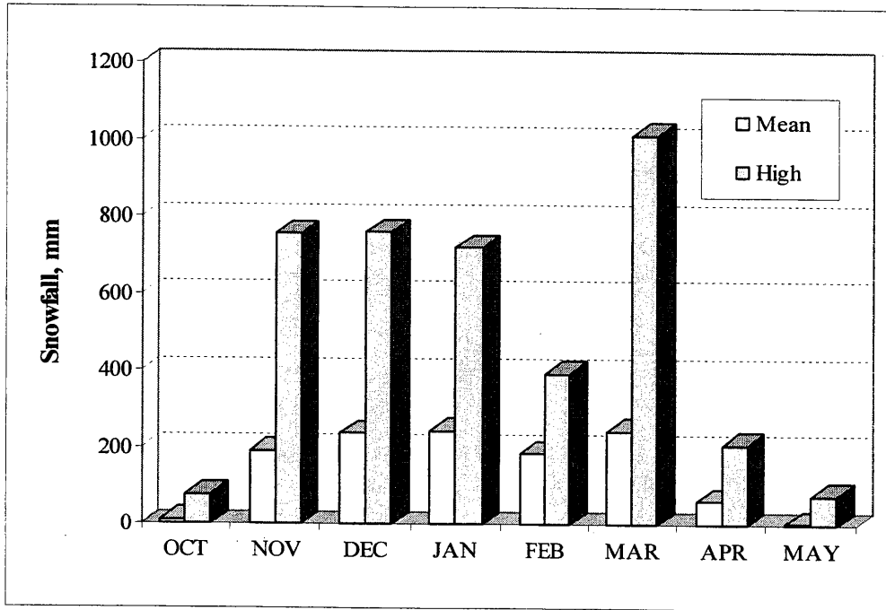
Figure 4.6. Mean and high monthly snowfall events, 1965 – 1995, Buffalo, MN weather station.
