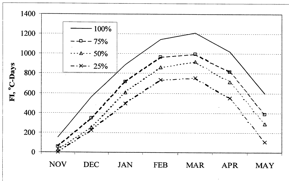
Figure 4.3. Distribution of FI over 30-years.
