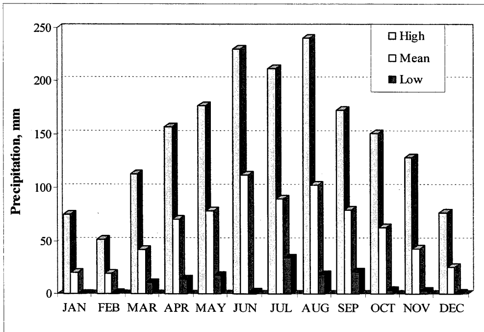
Figure 4.5. High, mean and low monthly precipitation events, 1965 - 1995, Buffalo, MN weather station.
