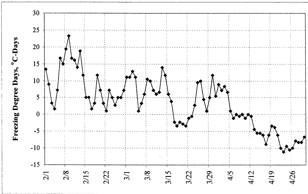
Figure 4.4. Freezing degree days beginning February 1, 1975, Buffalo.
