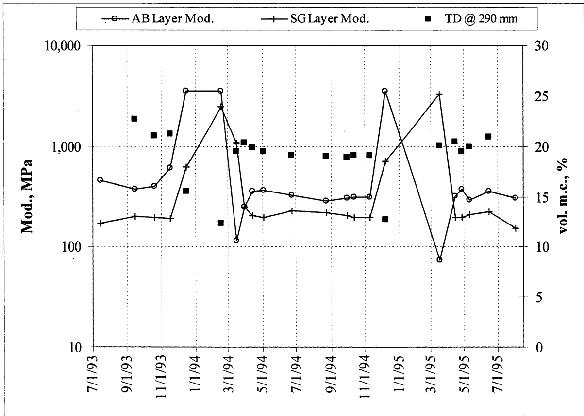
Figure 5.10. Seasonal variations in the AB and SG layer moduli compared to the volumetric moisture content at the Bemidji site.
