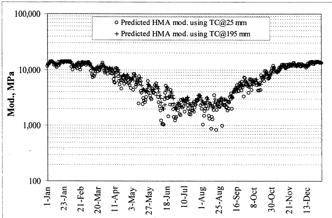
Figure 4.17. Predicted HMA modulus at 25 mm and 195 mm, in 1996.
