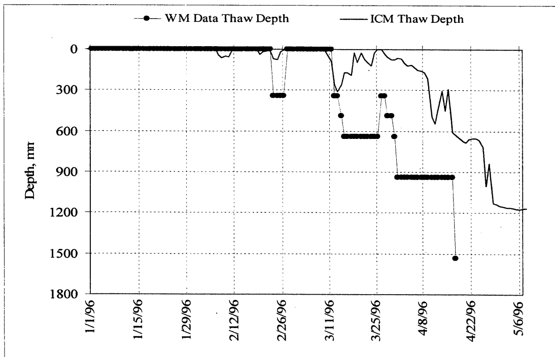
Figure 6.9. Predicted thawing front compared with WM data at test section 22, 1996.
