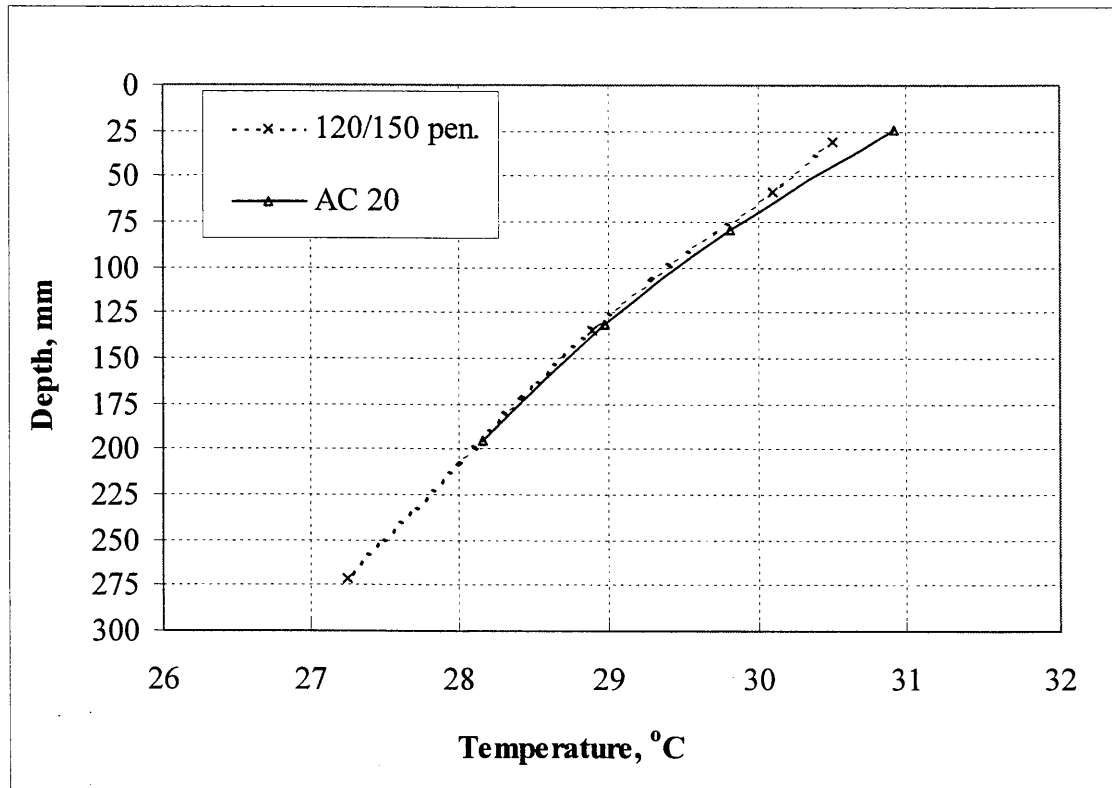
Figure 4.9. Mean monthly thermal gradient in July 1996 for test sections 19 (AC 20) and 20 (120/150 pen.).
