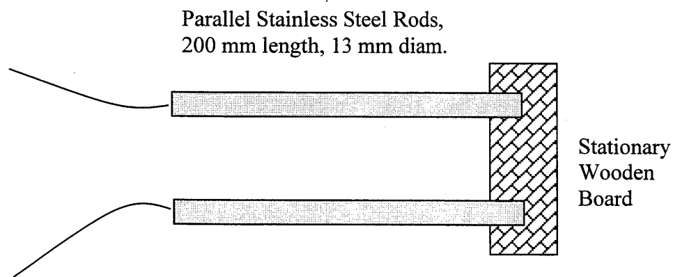
Figure 2.12. Time domain reflectometer at Mn/ROAD.
