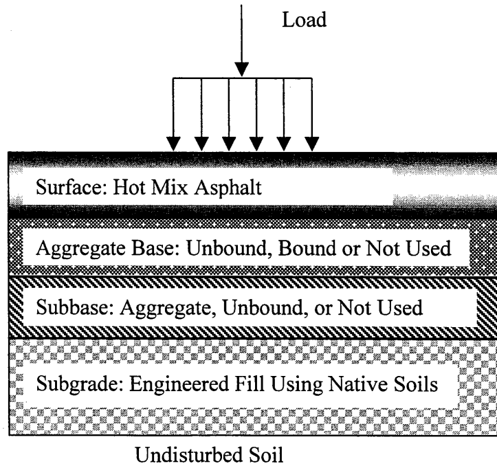
Figure 2.1. Typical materials used in HMA pavement structures.
