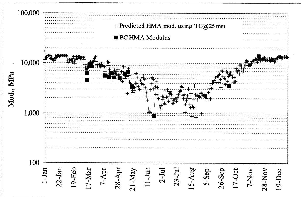
Figure 4.18. Predicted and backcalculated HMA modulus in 1996.
