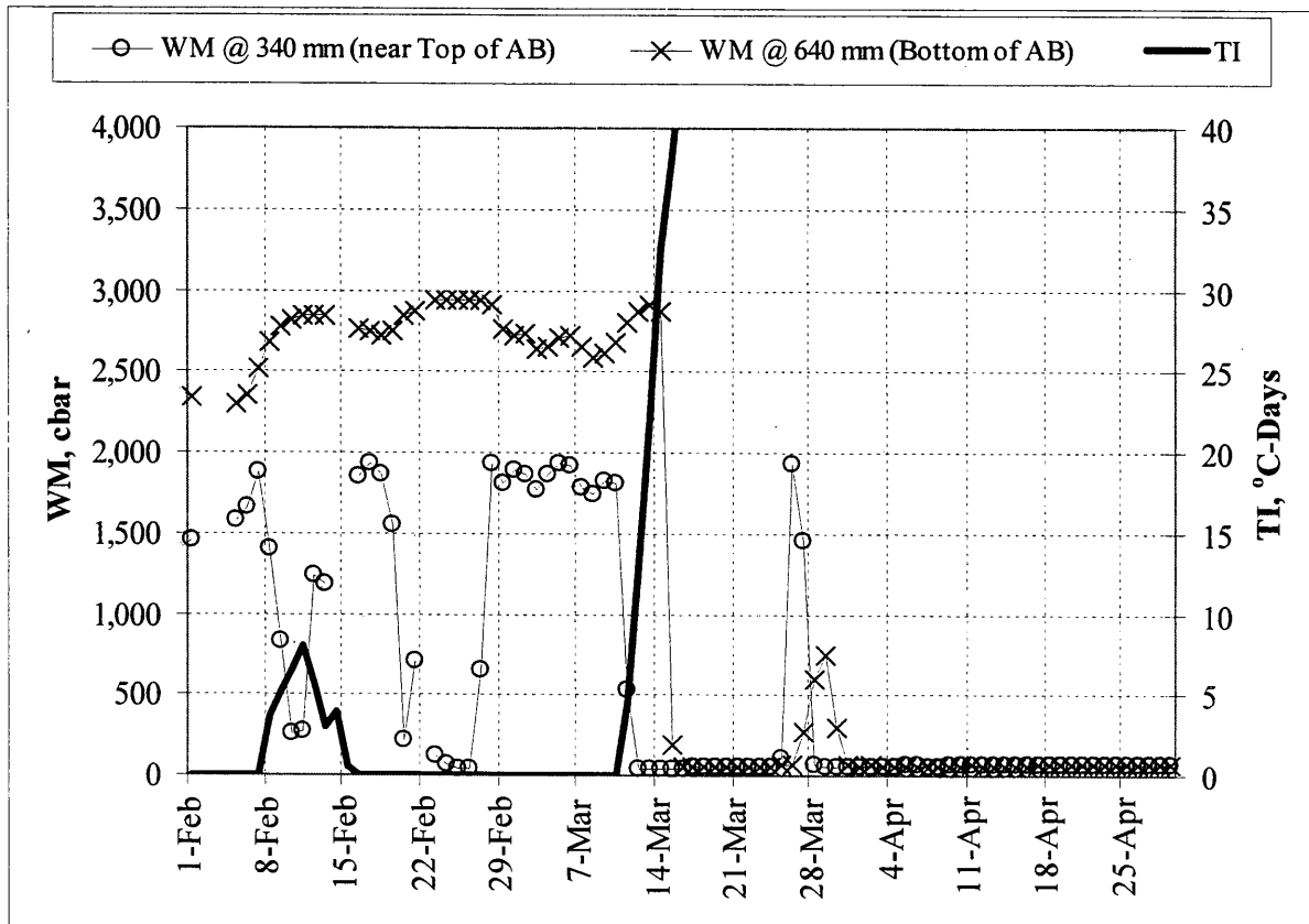
Figure 4.14. TI and WM data in test section 22, Cl. 6 Sp. base, spring 1996.
