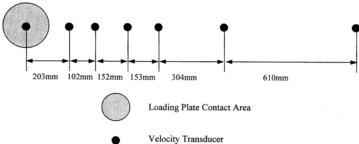
Figure 2.6. Planview of location of loading plate and velocity transducers for FWDs.
