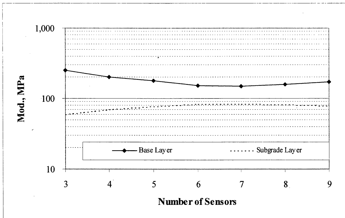
Figure 4.27. Modulus sensitivity for thin pavement, Cl. 5 Sp., E_{HMA} = 6000 MPa.
