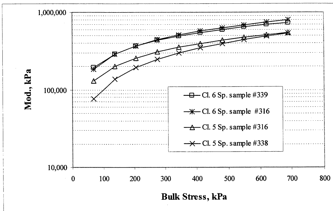
Figure 3.2. Modulus vs. bulk stress for Cl. 5 Sp. and Cl. 6 Sp. samples from Mn/ROAD [50].
