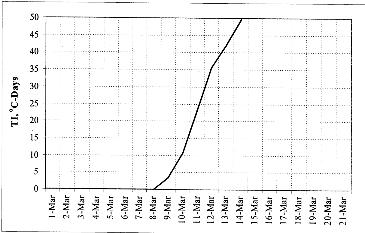
Figure 5.5. TI in Bemidji, spring 1995.
