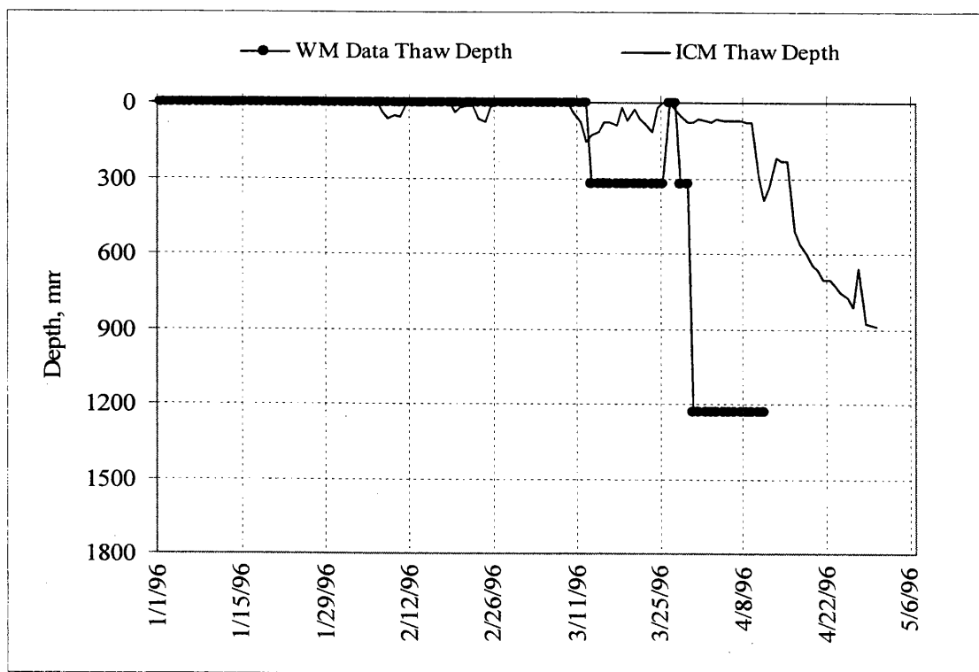
Figure 6.8. Predicted thawing front compared with WM data in test section 17, 1996.
