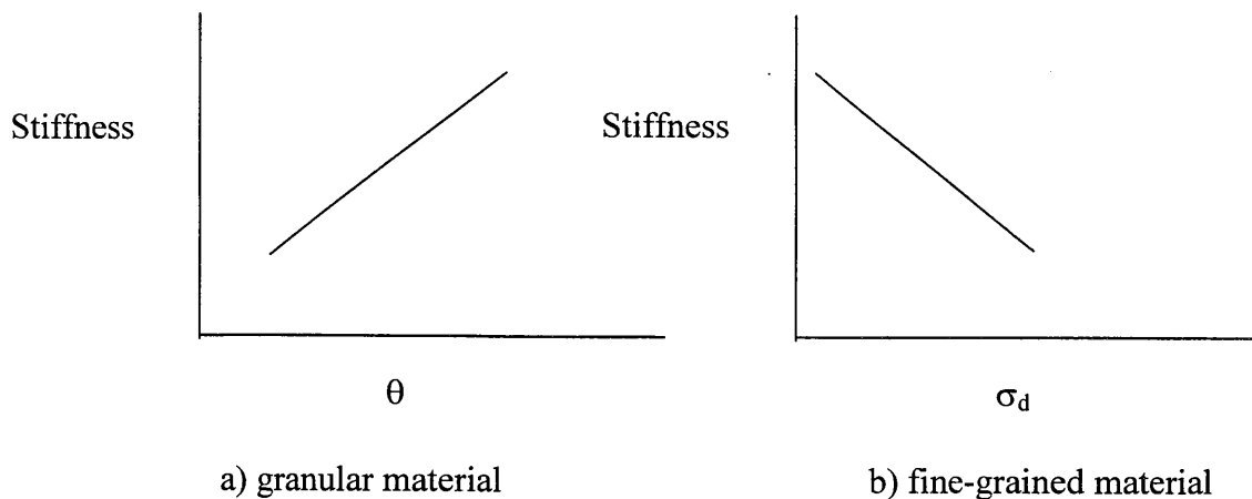
Figure 3.3. Simplified stress dependency relationships.
