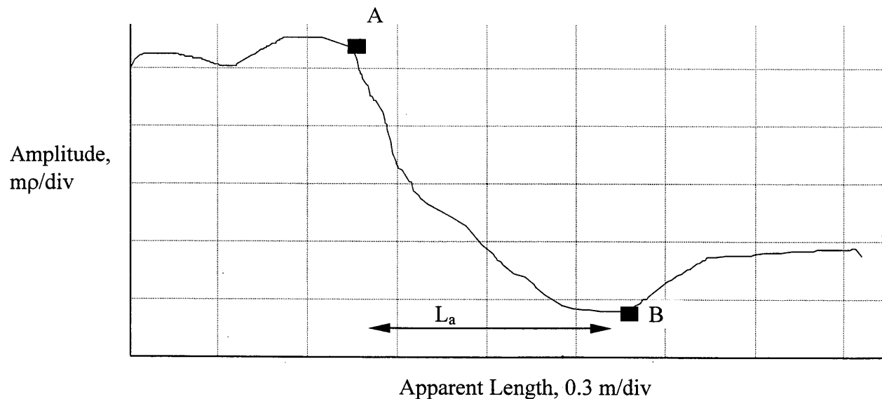
Figure 2.11. TDR trace where point A is the start and point B is the end of the TDR probe (mp/div is millirhos per division).
