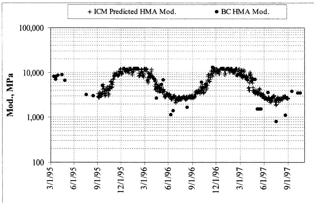
Figure 6.11. Comparison of predicted and backcalculated HMA moduli in test section 22.
