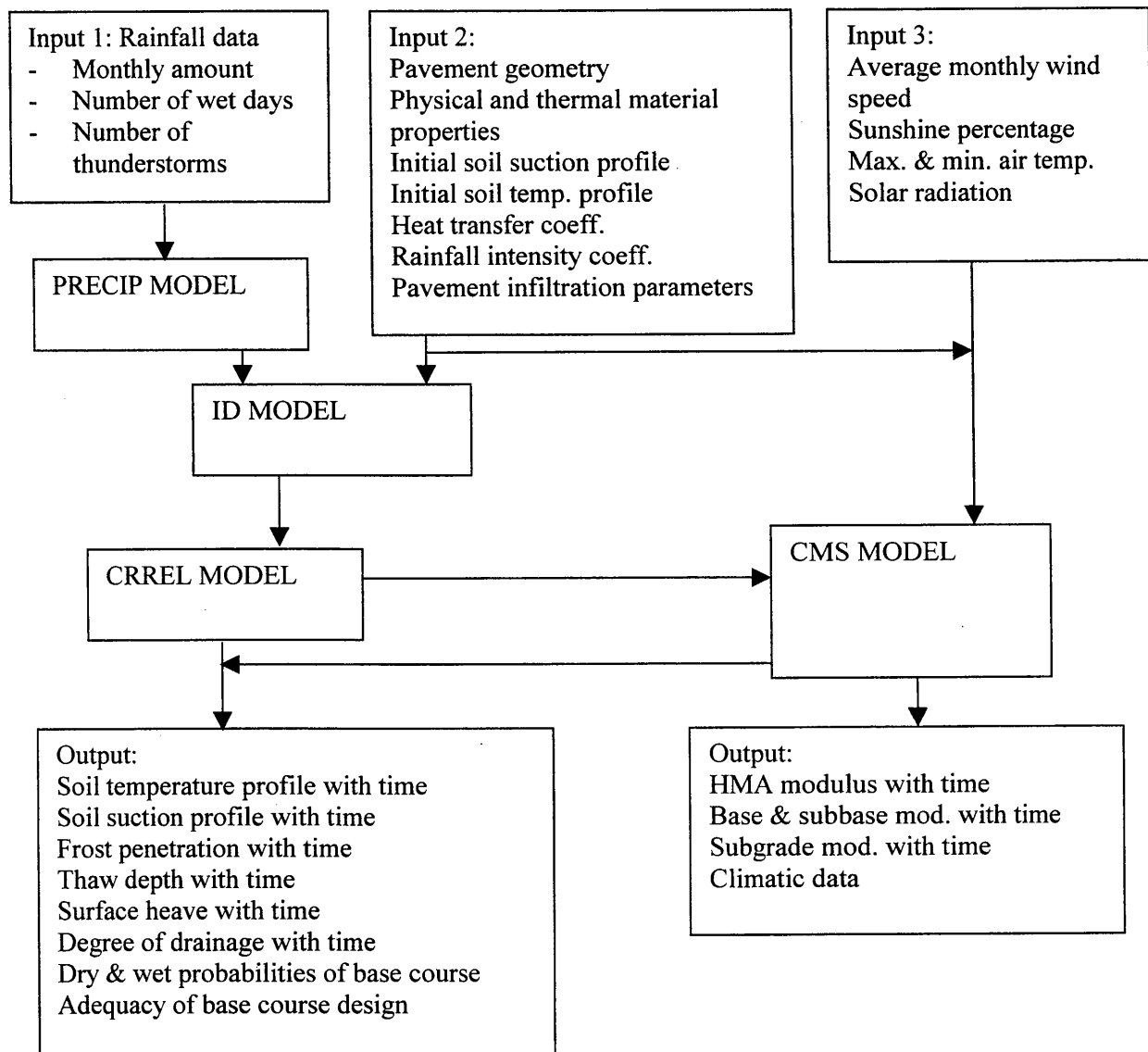
Figure 6.1. Integrated Climate Pavement Model [9].
