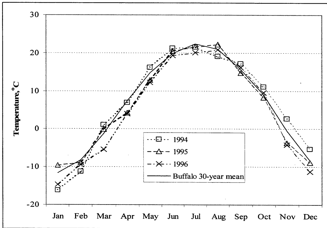
Figure 4.2. 30-year and Mn/ROAD mean monthly temperature.
