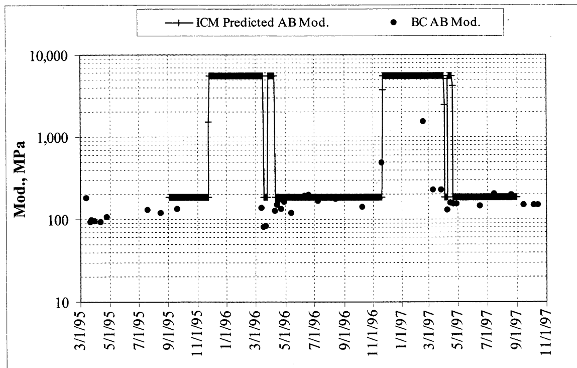
Figure 6.13. Comparison of predicted and backcalculated base layer moduli for test section 22.
