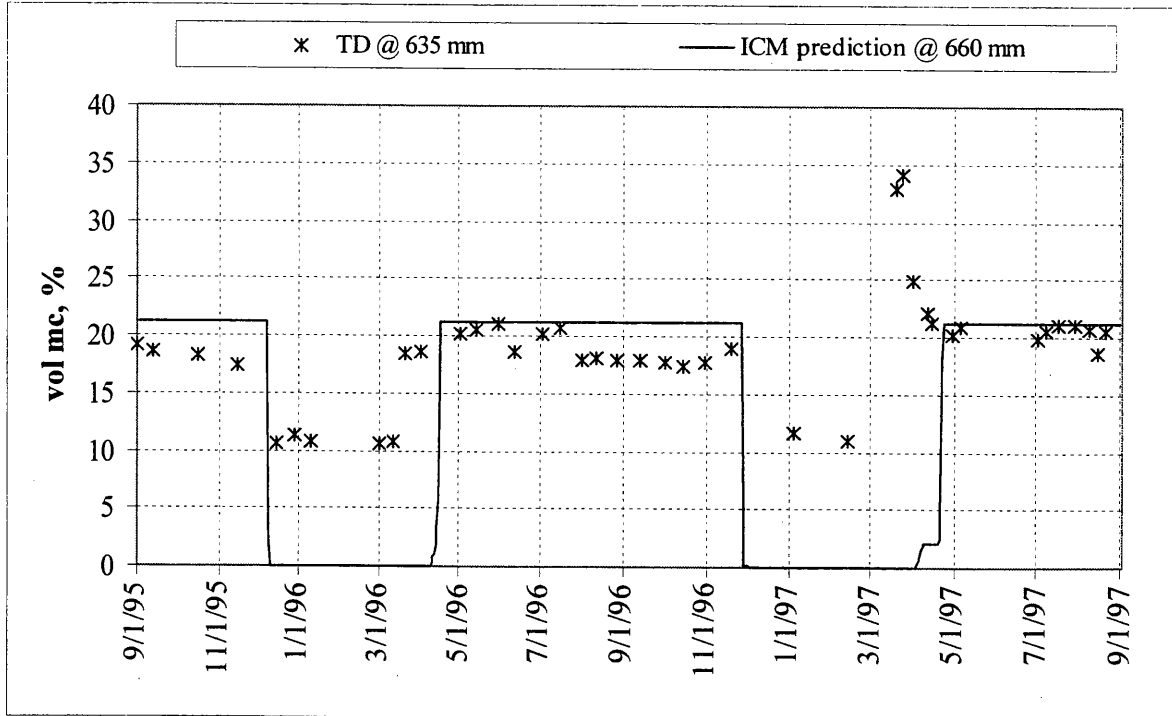
Figure 6.7. Comparison of measured and predicted volumetric moisture content in the base layer of test section 22.
