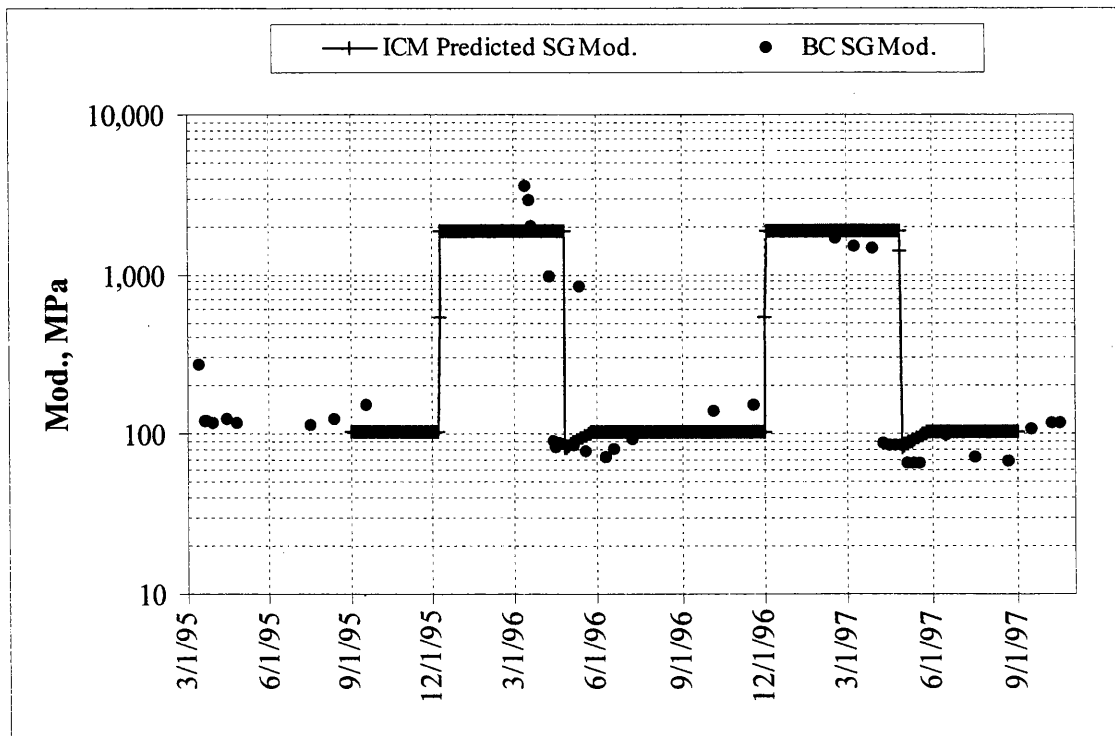
Figure 6.15. Comparison of predicted and backcalculated subgrade layer moduli for test section 22.
