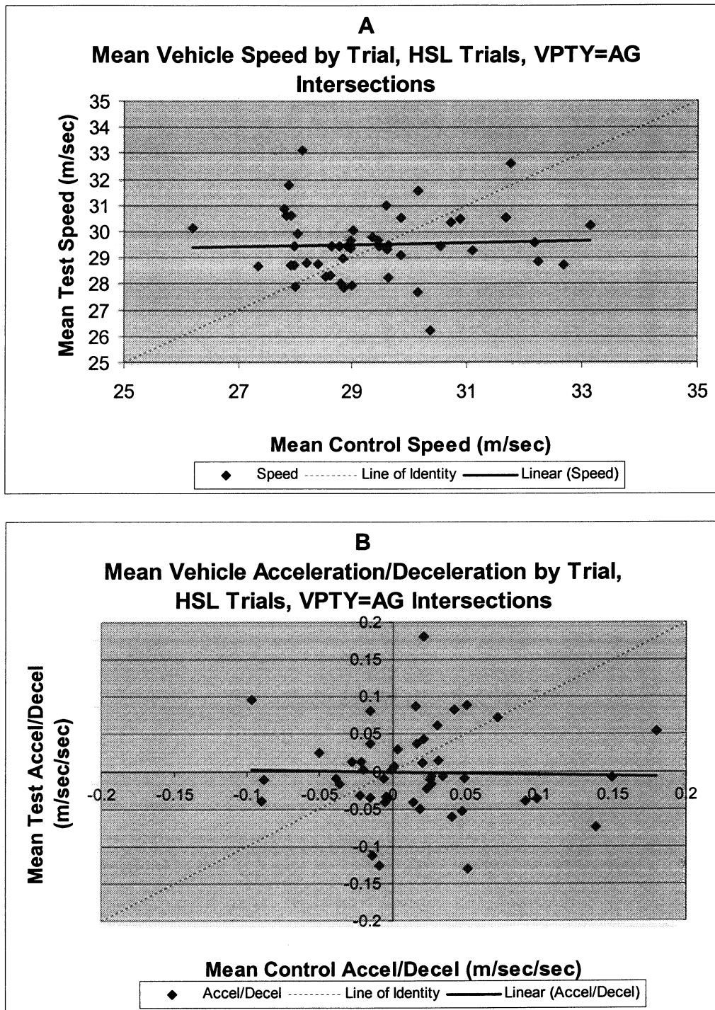
Figure N-1. Scatter plots of paired, within-subject control versus test mean results by trial for speed (A) and acceleration/deceleration (B) SDP measures, HSL trials, VPTY=AG intersections. Each point represents control-test paired means for 1 S. Solid line is LSR fit to data. Dashed line is line of identity.
