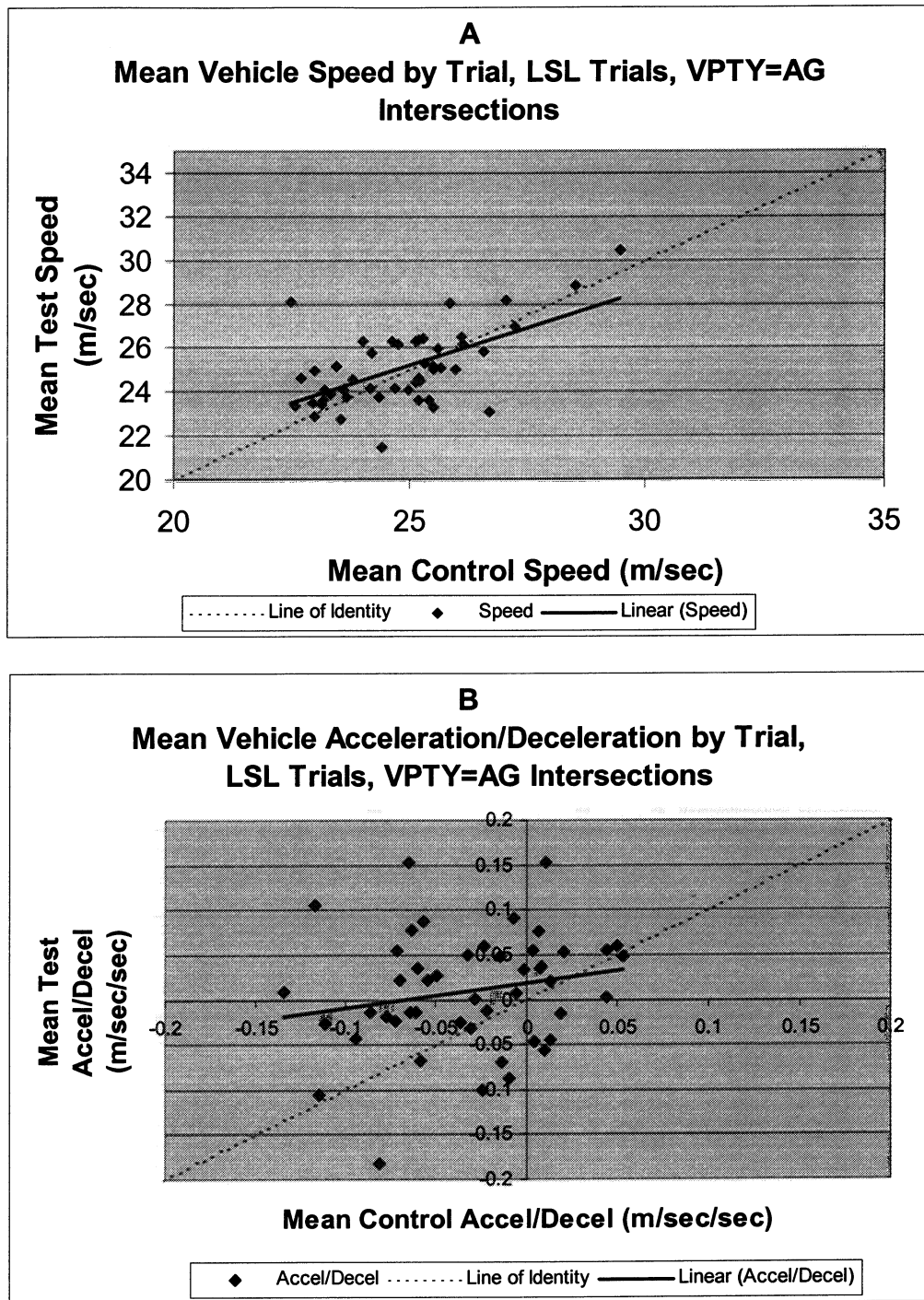
Figure M-1. Scatter plots of paired, within-subject control versus test mean results by trial for speed (A) and acceleration/deceleration (B) SDP measures, LSL trials, VPTY=AG intersections. Each point represents control-test paired means for 1 S. Solid line is LSR fit to data. Dashed line is line of identity.
