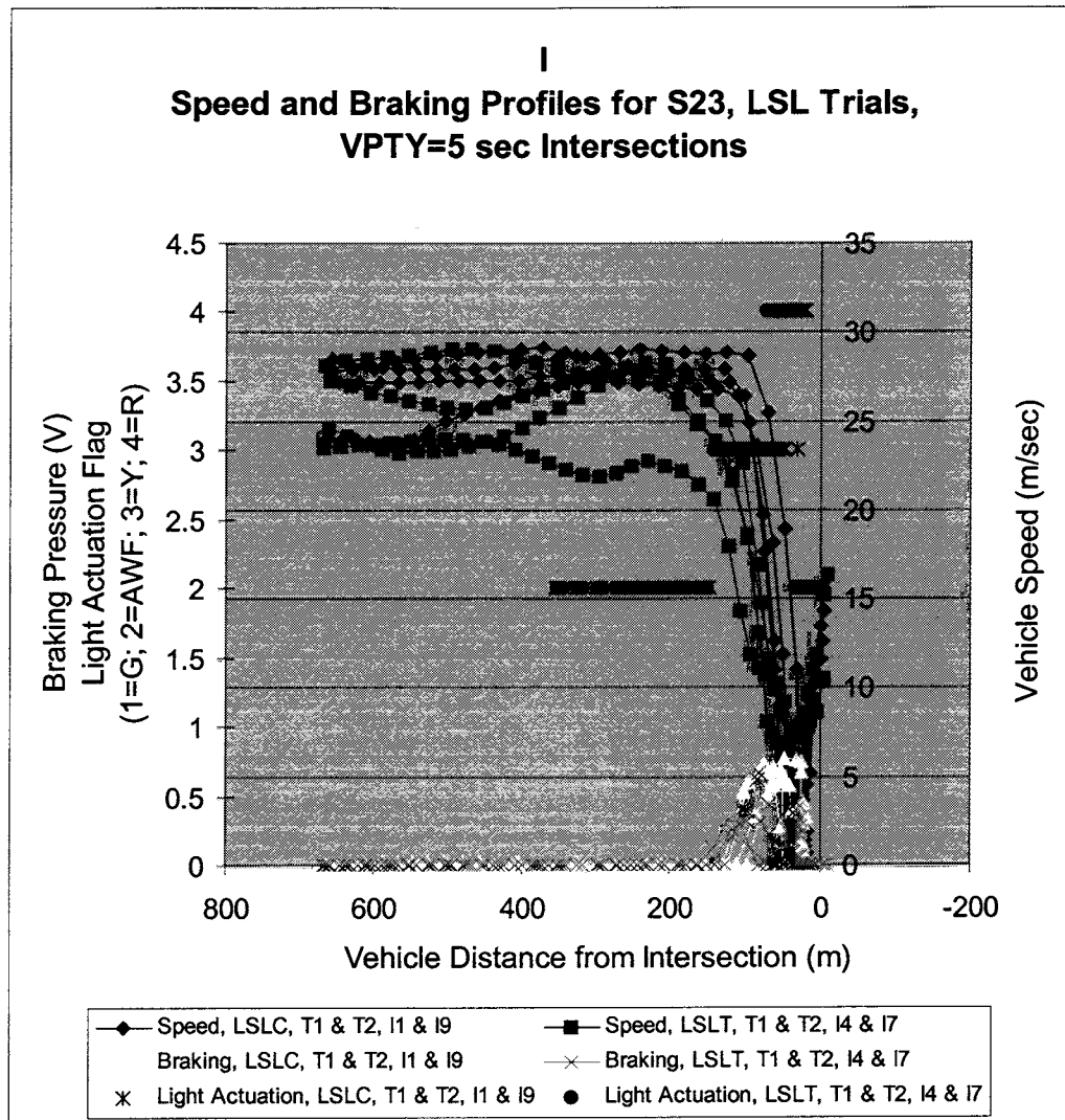
Figure L-1I. Speed and braking profiles for interactions of S23 with VPTY=5 sec intersections during LSL trials. Four profiles each for control and test trials (2 control and 2 test trials, and 2 VPTY=5 sec intersections per trial), along with light actuation flags for each trial, are plotted in relation to vehicle distance from the intersection.
