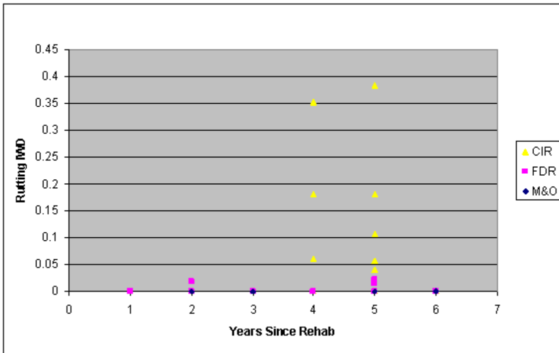
Figure 3.5: Rutting IWD recurrence.
