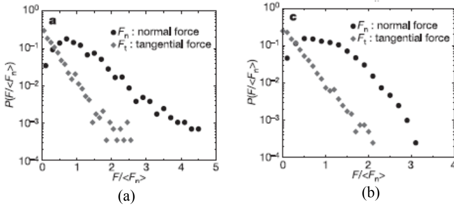
Figure 5.1: Force distribution [55]. (a) Probability distributions of the normal ( F_n ) and the tangential ( F_t ) forces for the sheared system on a semi-log scale. (b) Probability distributions of the normal and the tangential forces for the isotropically compressed system on a semi-log scale.
