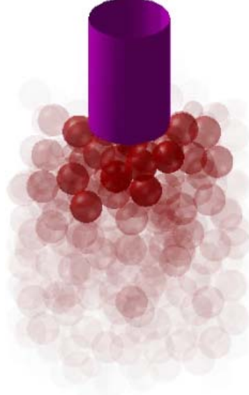
Figure 5.2: Inter-particle force distribution during a CBR test. The figure shows the summation of the normal forces on the each particle. The color intensity indicates the relative magnitude of the forces.
