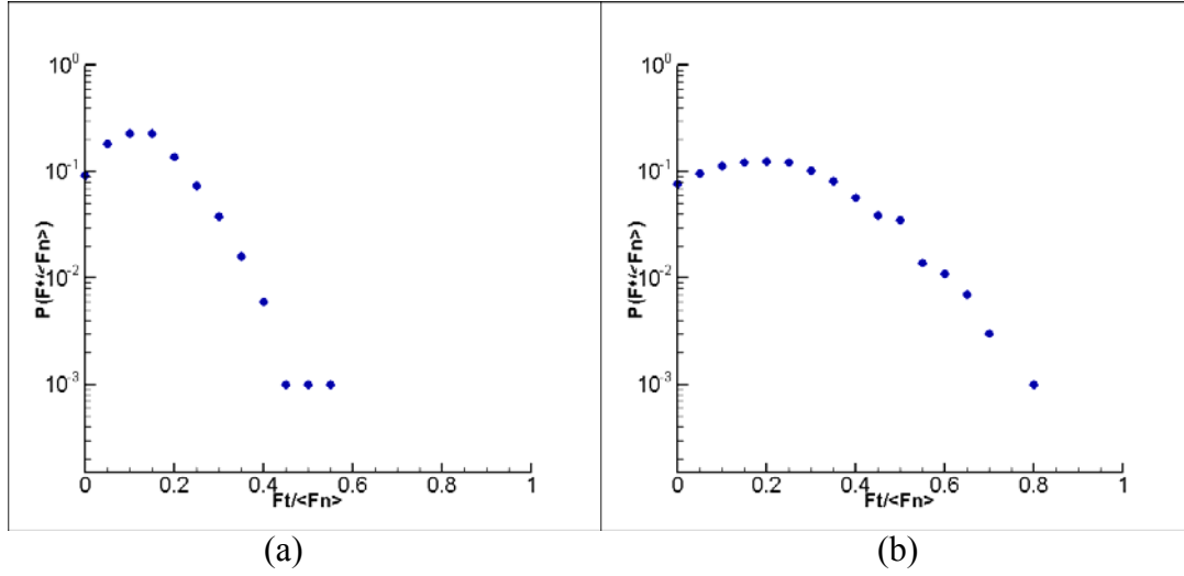
Figure 5.8: Tangential force distribution MR test. (a) Probability distributions (PDF) of the tangential force ( F_t ) during rest period. The forces are normalized by the average normal force \langle F_n \rangle . (b) PDF of the F_t during the maximum applied deviator stress.
