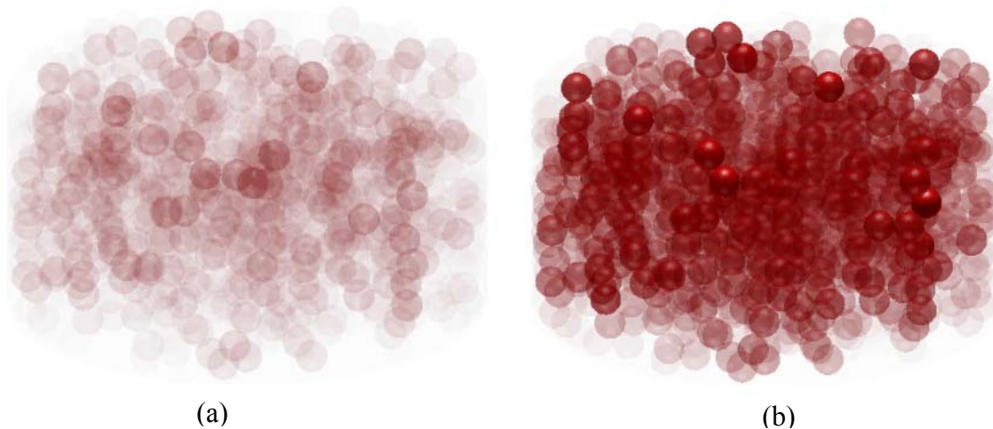
Figure 5.4: Inter-particle force distribution for MR test. The figure shows the summation of the normal forces on the each particle. The color intensity indicates the relative magnitude of the forces. (a) shows the magnitude of force during the rest period. (b) shows the magnitude of the force during the maximum deviator stress.
