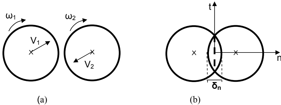
Figure 2.1: Illustration of the interaction of two particles in a soft sphere 2-D DEM model. (a) Two particles, particle 1 and particle 2, approach each other at a velocity of V_1 and V_2 . The particles can also have a rotational speed of \omega_1 and \omega_2 . (b) During collision the particles the deformation is represented by the normal overlap ( \delta_n ) between the two circular particles. The plane of contact is assumed to be flat and perpendicular to the line joining the centers of the two particles. n is the axis perpendicular (normal) to the contact plane and t is the axis parallel (tangential) to the contact plane.
