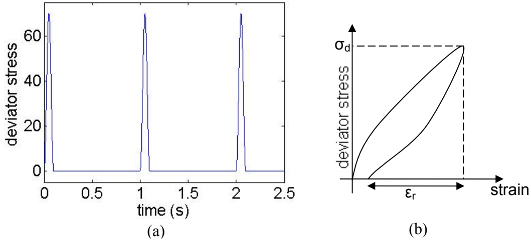
Figure 1.3: Application of cyclic deviator stress. (a) The cyclic deviator stress is applied at intervals of 1 s: 0.05 s loading, 0.05 s unloading and 0.9 s rest period. The loading and unloading impulse follows a haversine function. (b) The figure shows typical stress-strain curve. During loading the specimen deforms and during unloading some of the strain is recovered.
