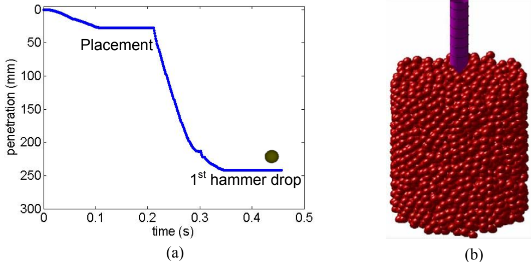
Figure 4.3: Typical result from DCP. (a) The graph shows the penetration incurred from a DCP test simulation during placement and first hammer drop. The penetration during the placement of the DCP is due to the weight of the apparatus. After the hammer is dropped the DCP penetrated larger depth. This test was performed for specimen comprising 5000 particles with physical properties of d = 10 mm, E = 29 GPa, \nu = 0.15 , \mu = 0.5 and \rho = 2650 kg/ m 3 . The surcharge load used is equivalent to 300 mm of granular materials of material density 2650 kg/ m 3 and solids fraction 0.60. b) Shows a snap shot from the DCP simulation: just before the DCP is placed on the surface of the sample.
