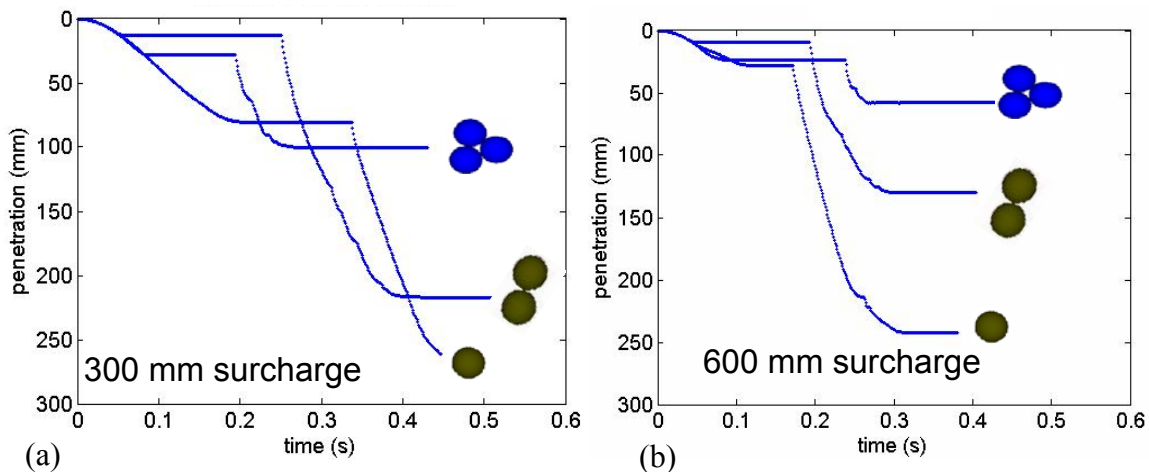
Figure 4.7: DCP test: surcharge load. (a) shows the penetration of DCP for three specimens where a 300 mm surcharge load is applied at the surface. The specimens were made of different shape of particles (Figure 4.6). (b) shows the penetration of DCP for three specimens where 600 mm surcharge load is applied. The shape of the particles is the same as in a. Increase in surcharge load decreased the penetration for the three specimens.
