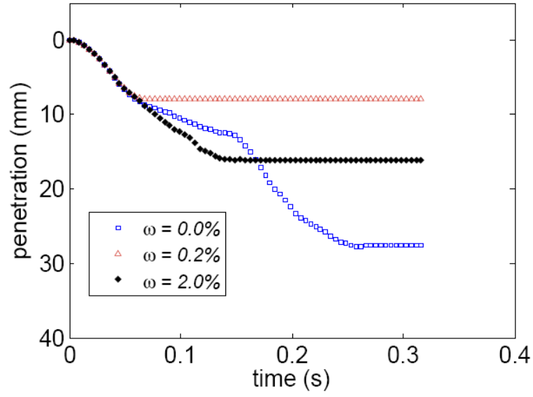
Figure B.3: DCP penetration for granular material with different moisture content as shown in the caption. The granular material was composed of 5000 ten millimeter particles ( E=29 GPa, \rho=2650 kg/m 3 , \mu = 0.5 and \nu = 0.15 ).
