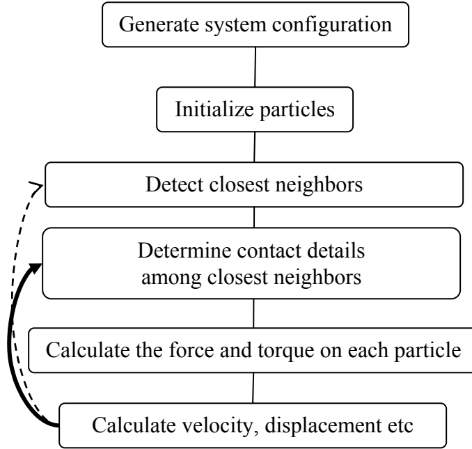
Figure 2.2: Flow chart for the DEM simulation. The simulation starts with generating system configuration and particle initialization. Possible contacts between particles are detected and the force between the particles is calculated based on effective overlap. Then displacement and velocity can be integrated from the acceleration of the particles. The solid arrow indicates that the explicit iteration for calculating the contact and forces. The broken line shows that nearest neighbor detection is not done for every iteration.
