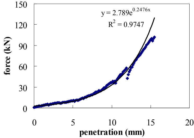
Figure 2.6: Resisting force vs. penetration for CBR test. The figure shows a plot of resisting force during plunger penetration in the CBR test. The force is measured at the intervals of 0.5 mm up to 15 mm. The resisting force increased continuously as the penetration depth increased. The test is performed on specimen comprising 3500 particles with physical properties of d = 10 mm E = 29 GPa, \nu = 0.15 , \mu = 0.5 and \rho = 2650 kg/m 3 . The discrete points represent results from the code and the solid line is an exponential fit to the data.
