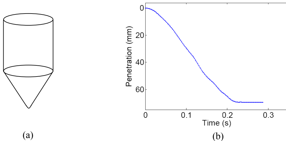
Figure 4.1: (a) Schematics of ‘light weight’ cone. (b) Results from the light weight cone drop test described in the text: graph of the penetration of the cone as a function of time. The graph shows penetration depths of a cone dropped a granular material. The specimen comprises 5000 10 mm spherical particles. The material properties are E = 29 GPa, \nu = 0.15 , \mu = 0.5 and \rho = 2650 kg/ m 3 .
