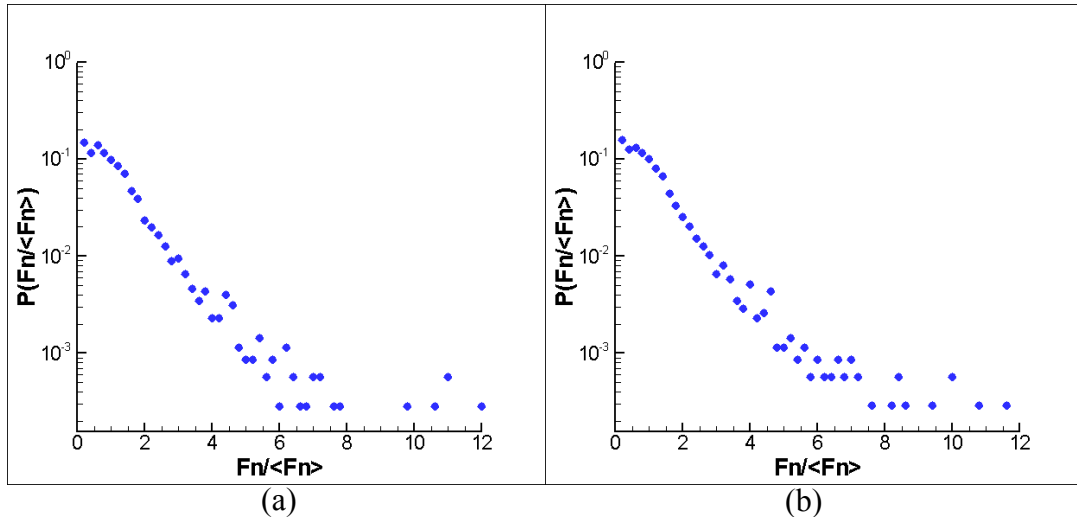
Figure 5.3: Normal force distribution CBR test. (a) Probability density function (PDF) of the normal forces ( F_n ) for the CBR test at 3 mm of plunger penetration. The forces are normalized by the average normal force \langle F_n \rangle . (b) PDF of F_n at 12.5 mm of plunger penetration.
