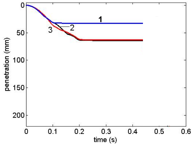
Figure 4.11: DCP test: height of specimen. The figure shows the penetration depths for specimen in three different specimens during placement of the DCP. The container size, the number of particles and the porosity of each test is shown in the table. The DCP penetrated more depth for the container with larger diameter.
