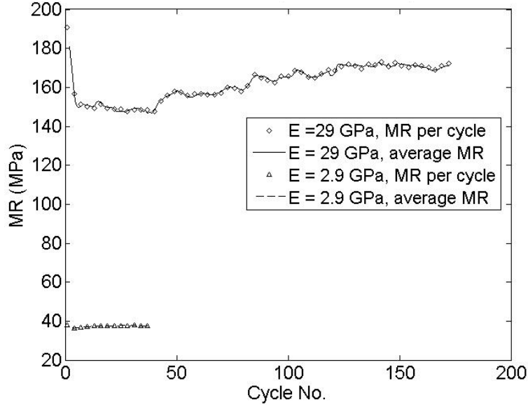
Figure 3.5: Calculated MR. The calculated MR from the simulation for two specimens with E = 2.9 GPa and E = 29 GPa. The symbols indicate the MR for every application of deviator load. The lines indicated the MR averaged over three consecutive MR values for every application of deviator stress.
