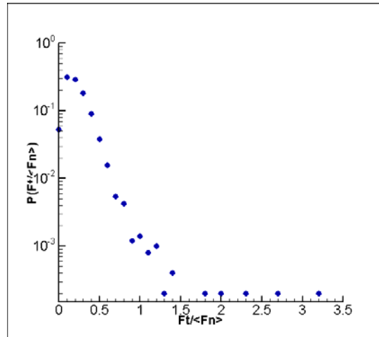
Figure 5.9: Tangential force distribution for the DCP test. The tangential force is normalized by the average normal force.
