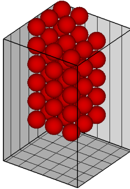
Figure 2.4: Suspended particles prior to drop. The figure shows 50 spherical particles suspended in a rectangular prism container. The base of the container is 150x150 mm. The size of the particles is 10 mm. The particles will be released at a very small random initial velocity.
