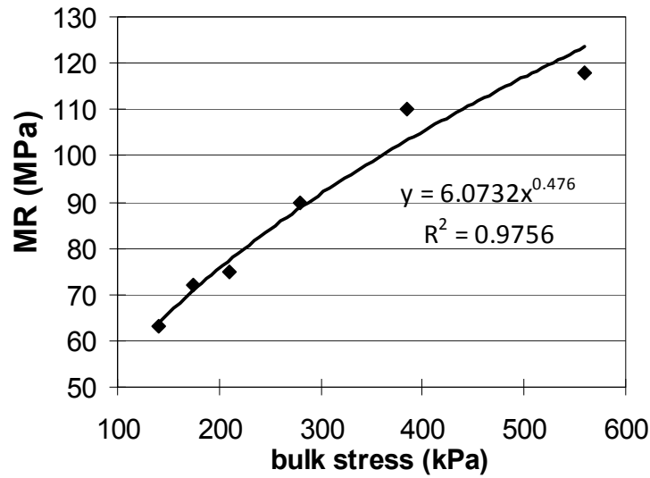
Figure 3.7: MR as a function of bulk stress. Calculated MR for specimen comprising particles of 10 mm diameter and 9 GPa of particle modulus of elasticity. MR increases as a power law function of the bulk stress. The constants k_1 and k_2 in Equation 3.5 are 6.07 and 0.476 respectively.
