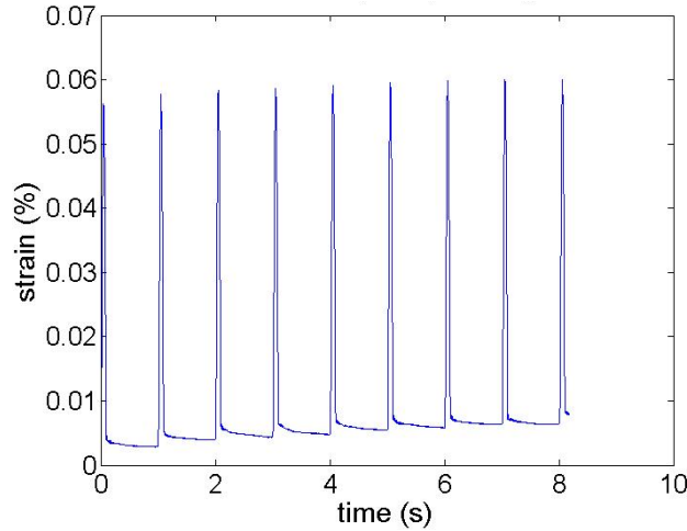
Figure 3.2: Strain (%) vs. time curve. The graph shows strain (%) incurred during application of the first nine cycles of deviator load. The confining and maximum deviator stresses were 35 kPa and 70 kPa. These results are from a specimen comprising 1500 particles with physical properties of d = 10 mm E = 20 GPa, \nu = 0.15 , \mu = 0.5 and \rho = 2650 kg/ m 3 .
