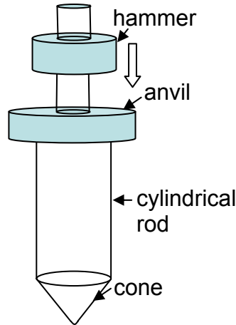
Figure 4.2: Schematics of DCP apparatus (not to scale). The cone is connected to the cylindrical rod. The hammer is dropped onto the anvil, which is attached to the cylindrical rod.
