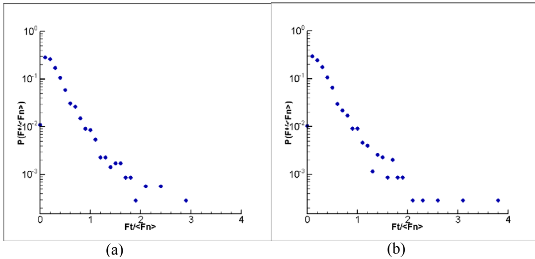
Figure 5.7: Tangential force distribution for CBR test. (a) Probability distributions of the tangential forces ( F_t ) at 3 mm of plunger penetration. The forces are normalized by the average normal force \langle F_n \rangle . (b) PDF of F_t at 12 mm of plunger penetration.
