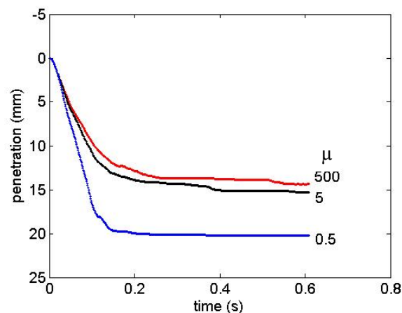
Figure 4.4: ‘Cone Drop’ test: coefficient of contact friction. The graph shows penetration depths of a cone dropped on specimens that have different coefficient of contact friction (0.5, 5 and 500). The tests were performed on a specimen that has gradation of 10%: 60%: 30% 19 mm: 9.5 mm: 4.75 mm. The difference between the penetrations for coefficients of friction of 0.5 and 5 is of the same order of the smallest particle size.
