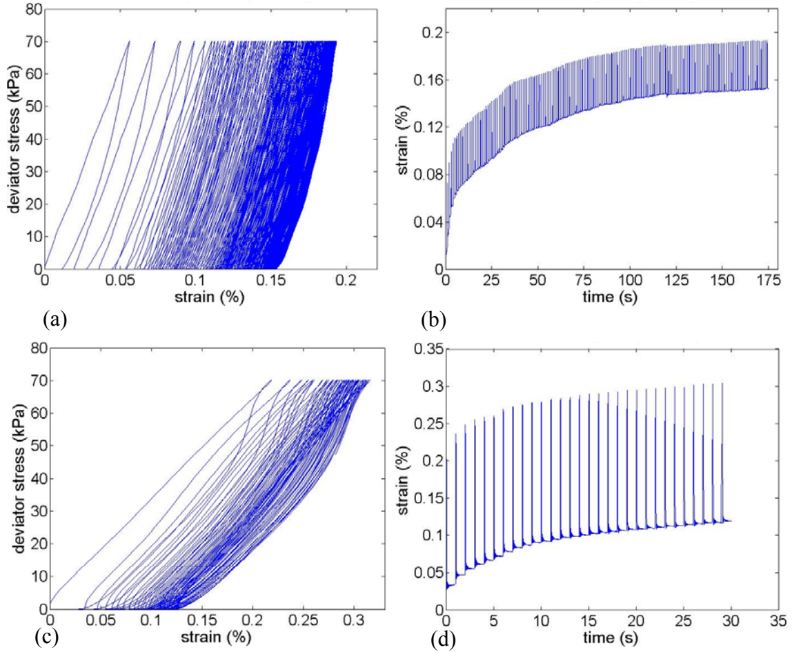
Figure 3.3: Typical results from MR simulation. (a) shows the stress-strain curve for specimen comprising 1500 spherical particles with physical properties d = 10 mm E = 29 GPa, \nu = 0.15 , \mu = 0.5 and \rho = 2650 kg/ m 3 . (b) shows the strain incurred for the simulation as shown in a. The permanent deformation approaches a constant value after application of 170 cycles of deviator stress. (c) shows stress-strain curve for another specimen which is similar as described in (a) but with E = 2.9 GPa. (d) shows the strain incurred for the simulation shown in c. The permanent deformation approaches a constant value after application of 30 cycles of deviator stress.
