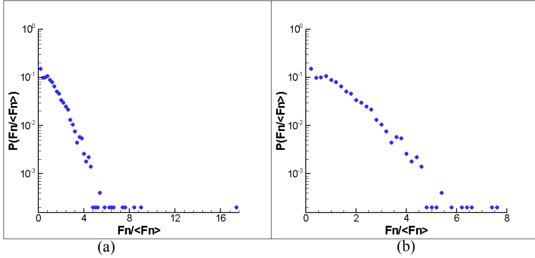
Figure 5.6: Normal force distribution DCP test. (a) Probability distributions of the normal ( F_n ) forces on a semi-log scale. The forces are normalized by the average normal force \langle F_n \rangle . (b) Zoom in of (a).
