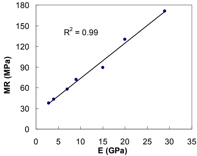
Figure 3.6: MR vs. E. The graph shows the calculated MR from simulations as a function of particle modulus of elasticity. The simulations are done for particle modulus of elasticity of 2.9, 4, 7, 9, 15, 20 and 29 GPa. The graph shows that the MR is a linear function of the particle modulus of elasticity.
