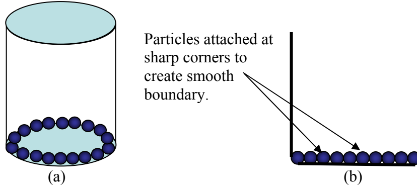
Figure 2.5: Schematic representation of the CBR plunger (not to scale). Spherical particles are glued at the joint of the circular wall and the cylindrical wall. a) 3-D view of the plunger b) cross sectional view of the plunger.
