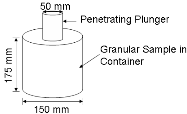
Figure 1.1: Schematics of CBR. The container has a diameter of 150 mm and height of 175 mm. The plunger which has a diameter of 50 mm penetrates at a constant rate of 1mm/min.
