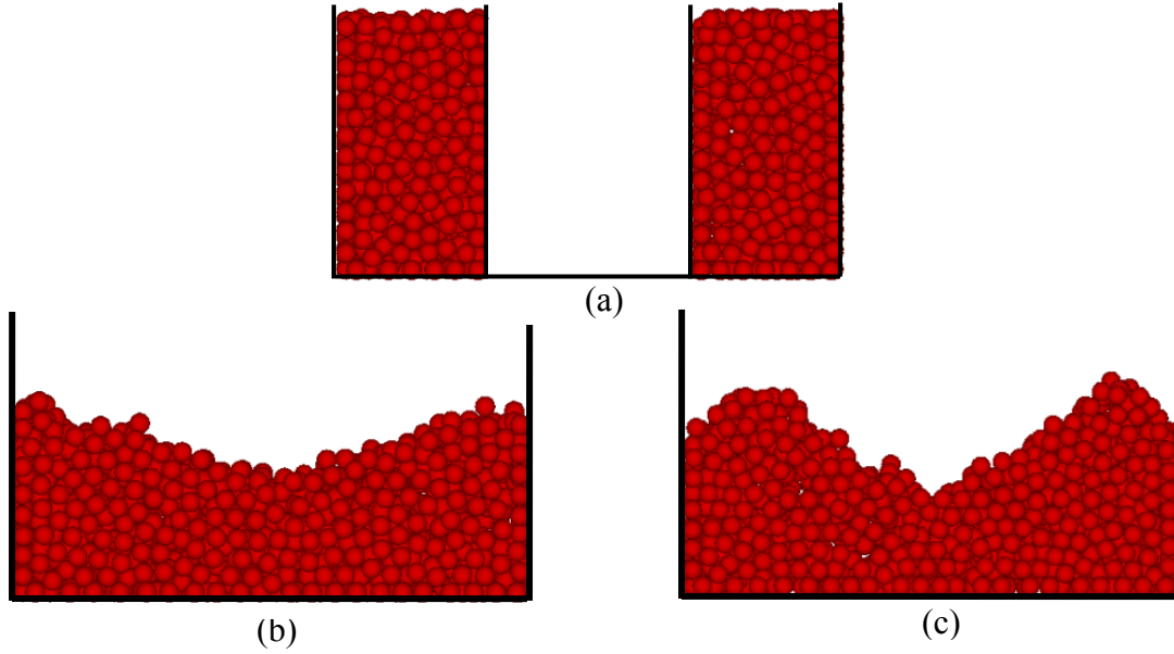
Figure B.2: Collapse of granular material. (a) Granular material in a rectangular container supported by vertical walls. (b) Collapse of dry granular material when the vertical supporting walls are removed. (c) Collapse of granular material with 0.2% moisture content. The slope is steeper for the wet granular material than the dry one.
