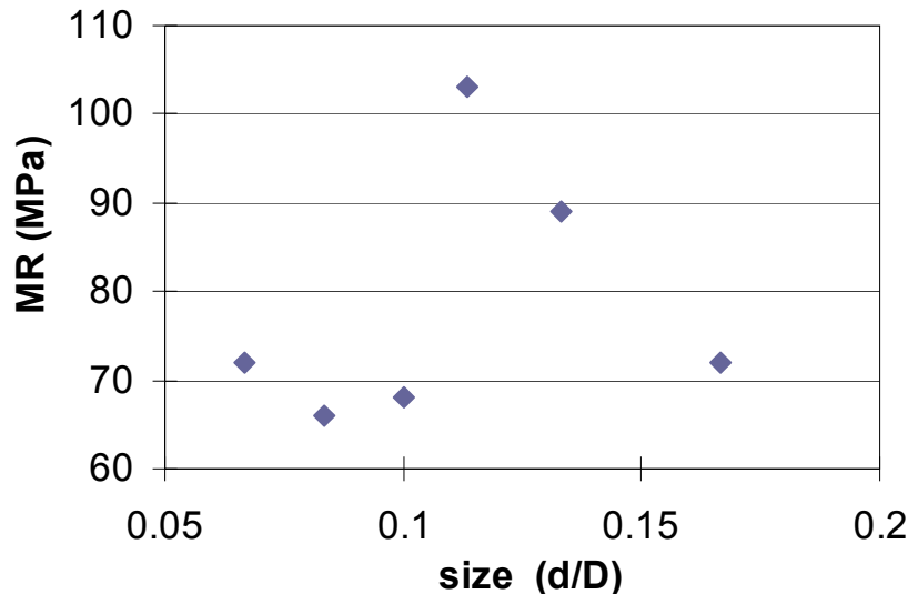
Figure 3.8: MR for different particle size. The graph shows calculated MR for different particle size. The x-axis is the size of particles normalized by the diameter of the cylindrical container (150 mm). The y-axis shows the MR in MPa. For d/D < 0.1 , the MR value is relatively stationary, but for larger values of d/D the value for MR is significantly more variable.
