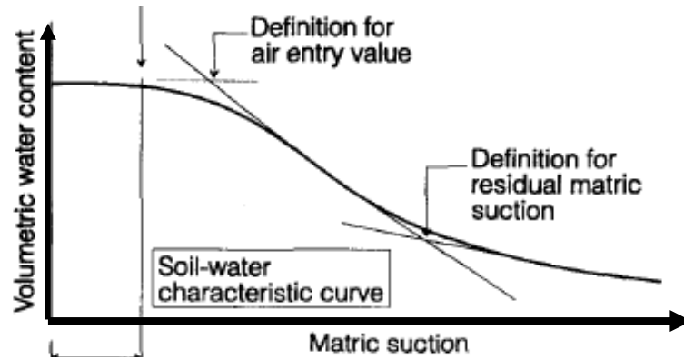
Figure B.1: Soil Water Characteristic Curve. The matric suction decreases with increasing water content (Gan and Fredlund [61]).
