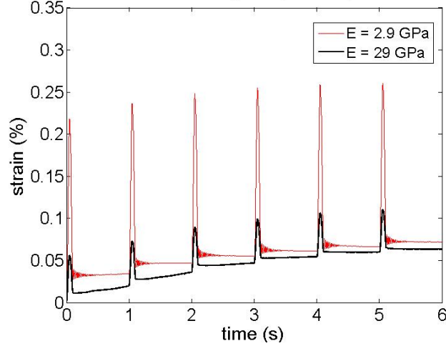
Figure 3.4: Strain(%) for different modulus elasticity. The figure shows comparison of strain for specimen comprising particles with modulus of elasticity of 2.9 GPa and 29 GPa. More strain is observed for the softer material.
