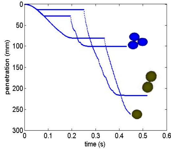
Figure 4.6: DCP test: particle shape. The figure shows penetration during placement of the DCP and during the first hammer drop. The test was performed on specimens that contain different particle shape. The first specimen comprises 5000 spherical particles of 10 mm diameter. The second sample comprises 2500 couples, each couple is made by gluing two 10 mm diameter spherical particles together. The third specimen comprises 1667 triplets, which are made by gluing three 10 mm spherical particles. The centers of the three glued particles form an equilateral triangle. The particles in the three cases have physical properties of E = 29 \text{ GPa} , \nu = 0.15 , \mu = 0.5 and \rho = 2650 \text{ kg/m}^3 . The penetration is larger for the specimen with spherical particles. The penetration during the hammer drop decreases as more particles are glued together.
