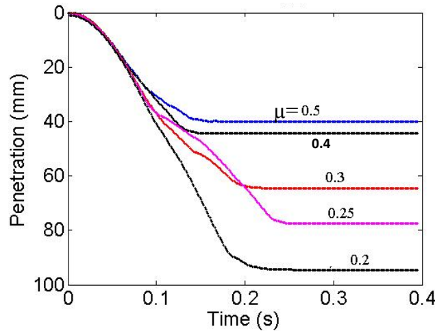
Figure 4.5: DCP test: coefficient of contact friction. The figure shows penetration depths incurred during placement of the DCP on specimens with different values of coefficient of contact friction (0.2, 0.25, 0.3, 0.4 and 0.5). The penetration decreases as the coefficient of contact friction increases. The difference in the penetration depths is larger for lower coefficients of friction. However, the penetration depths do not vary much after the coefficient of friction of 0.4. The particle material properties are as mentioned in Figure 4.3 and the surcharge load is 300 mm thick.
