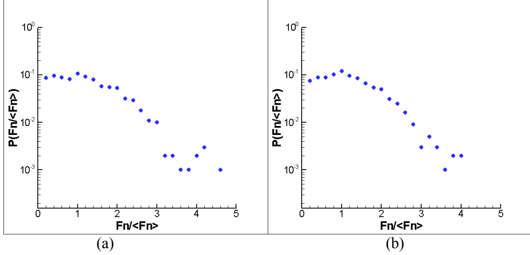
Figure 5.5: Normal force distribution for MR test. (a) Probability distributions (PDF) of the normal forces ( F_n ) during rest period. The forces are normalized by the average normal force \langle F_n \rangle . (b) PDF of the F_n during the maximum applied deviator stress.
