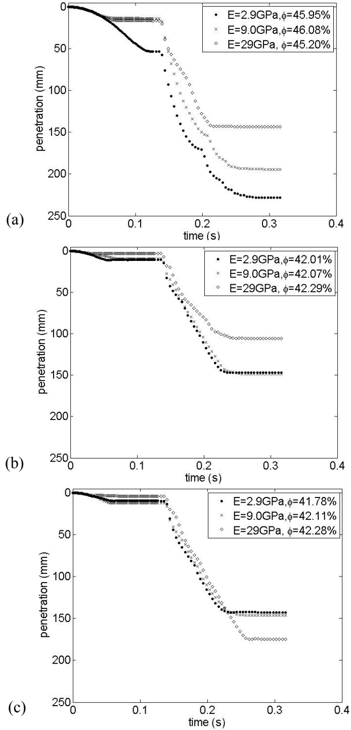
Figure 4.8: DCP test: modulus of elasticity. The three graphs show penetration of the DCP during placement and first hammer drop. The graphs show comparison of penetration depth for specimen with different modulus of elasticity (2.9, 9 and 29 GPa). The specimens comprise 2500 ‘couple’ particles made by gluing 10 mm spheres. The porosity of each specimen is indicated in the legend.
