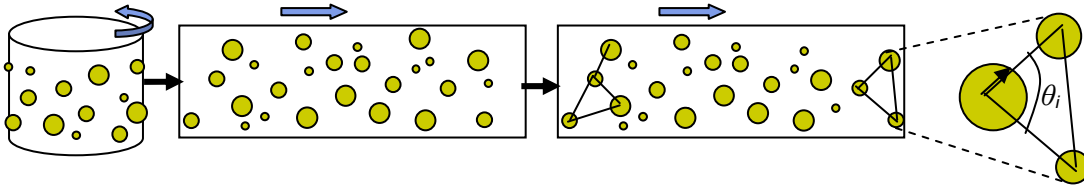
Figure 3.1: Illustration of force calculation due to the hydrostatic boundary. The figure shows how centers of particles touching the lateral boundary are mapped into a rectangular plane and the formation of the Delaunay Triangulation. The confining pressure is then applied on each triangle depending on the area of the triangle.
