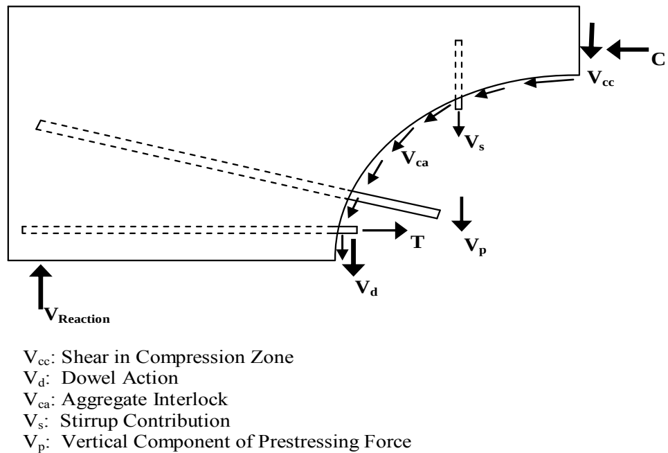
Figure 2.1 Shear Transfer/Actions Contributing to Shear Resistance (Hawkins et al. 2005)
