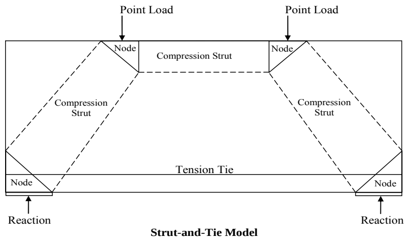
Figure 2.5 Strut-and-Tie Model for a Simple Deep Beam Figure
