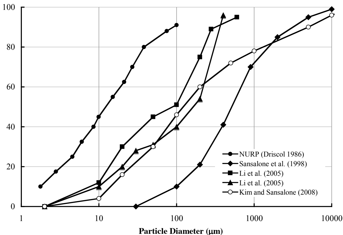
Figure 1. Comparison of cumulative size distributions (percent by mass greater than) for the NURP studies and receipt highway runoff studies. The NURP distribution was determined by conversion of measured settling velocity distribution to particle size assuming silica particles.
