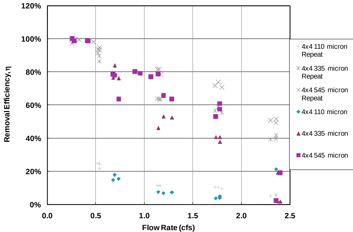
Figure 3.2. Comparison of the Original and the Repeat Tests of Removal Efficiency for the 4×4 ft Sump
