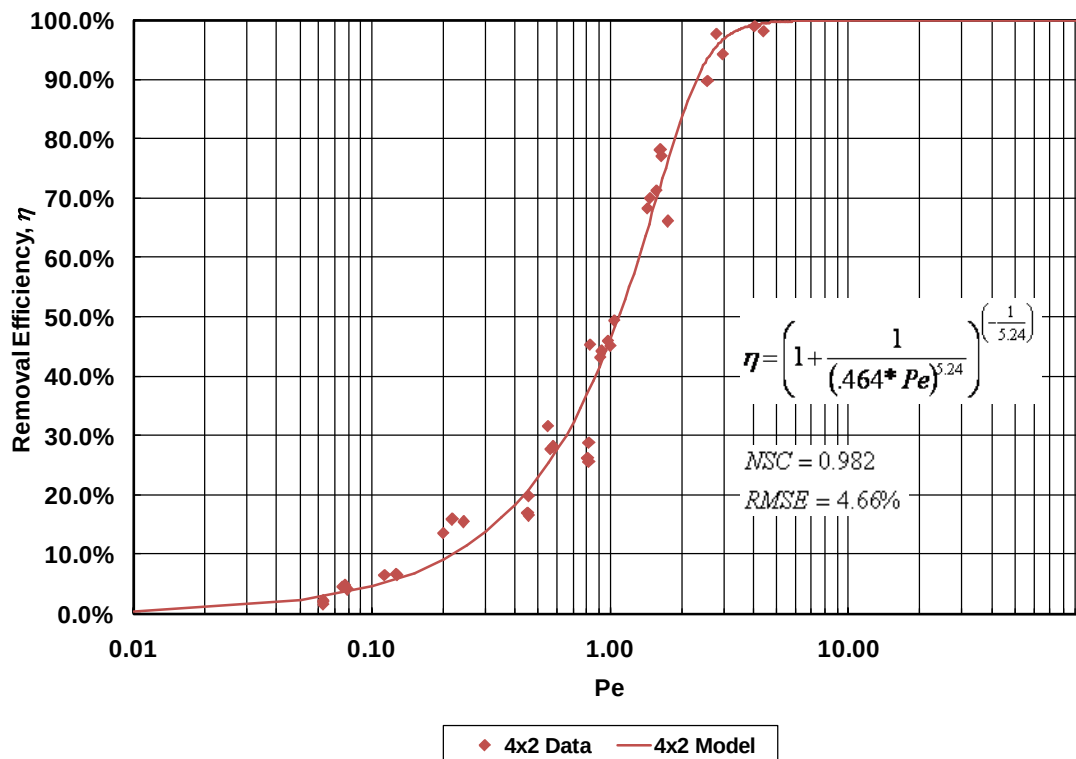
Figure G.2. 4×2 ft Standard Sumps Removal Efficiency Results
