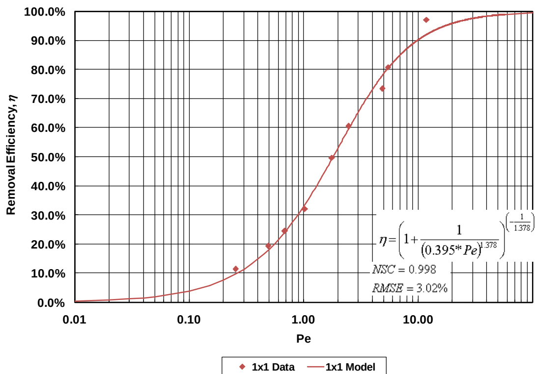
Figure G.5. 1×1 ft Standard Sumps Removal Efficiency Results
