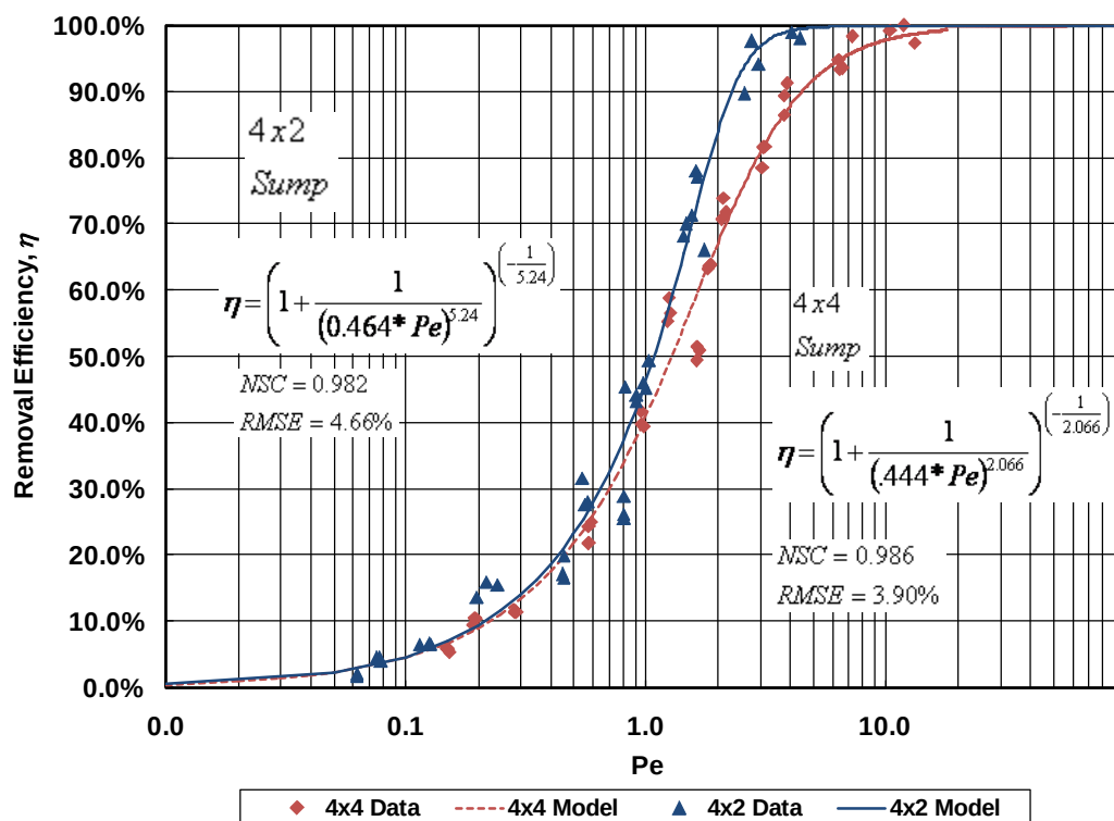
Figure G.7. Comparison of the Removal Efficiency Results for 4×4ft and 4×2ft Sumps
