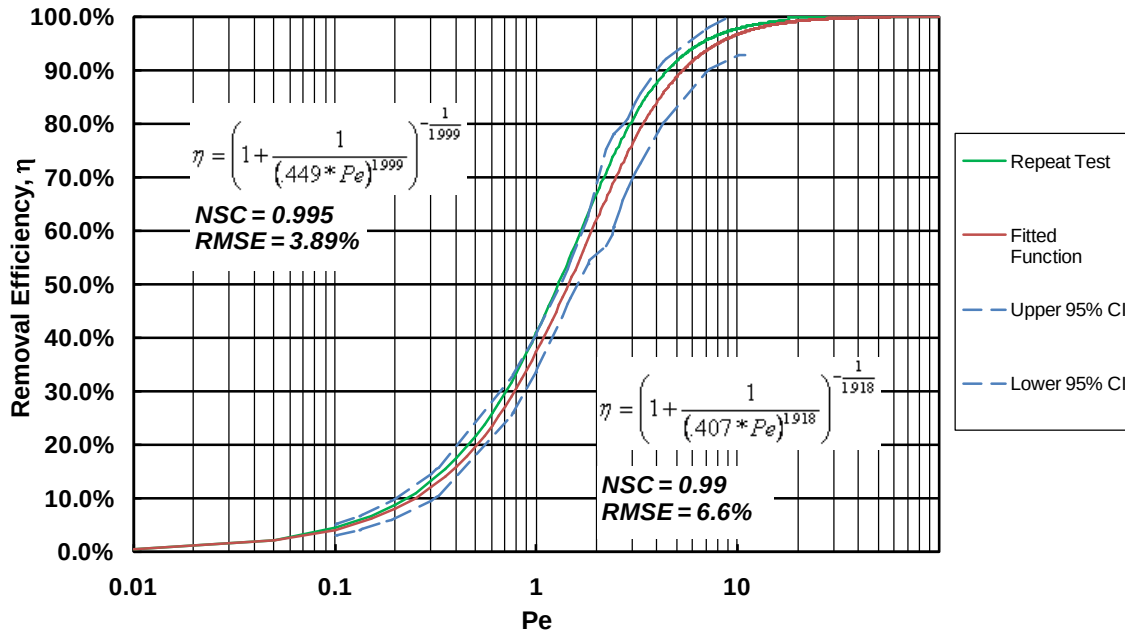
Figure G.6. Repeatability of Removal Efficiency Results for 4×4 ft Sump
