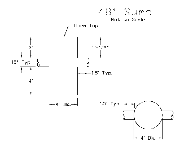
Figure A.1. 4×4 ft Sump Design Drawing
