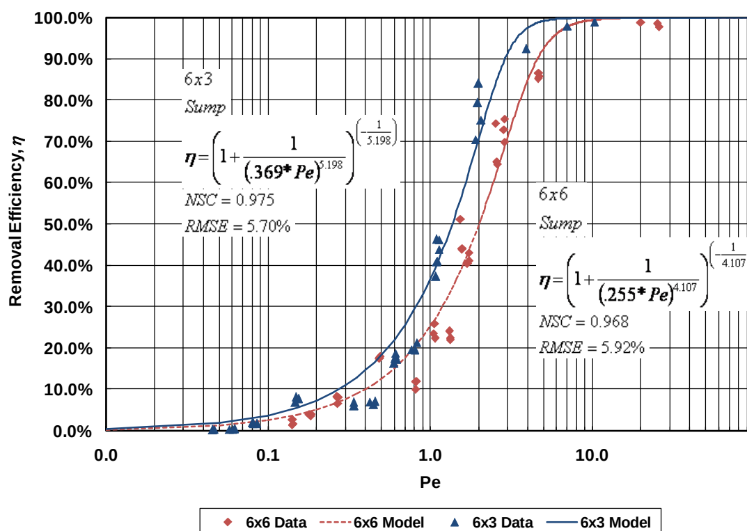
Figure G.8. Comparison of the Removal Efficiency Results for 6×6ft and 6×3ft Sumps
