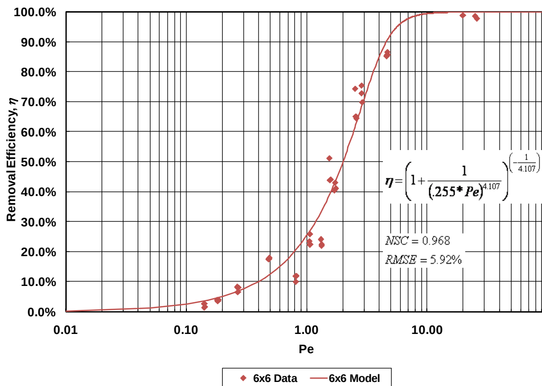
Figure G.3. 6×6 ft Standard Sumps Removal Efficiency Results
