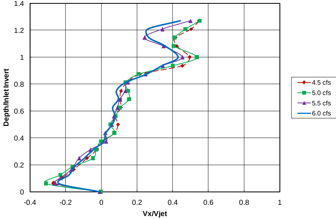
Figure 4.4. Velocity Measurements at Center Location in the 4-ft Standard Sump
