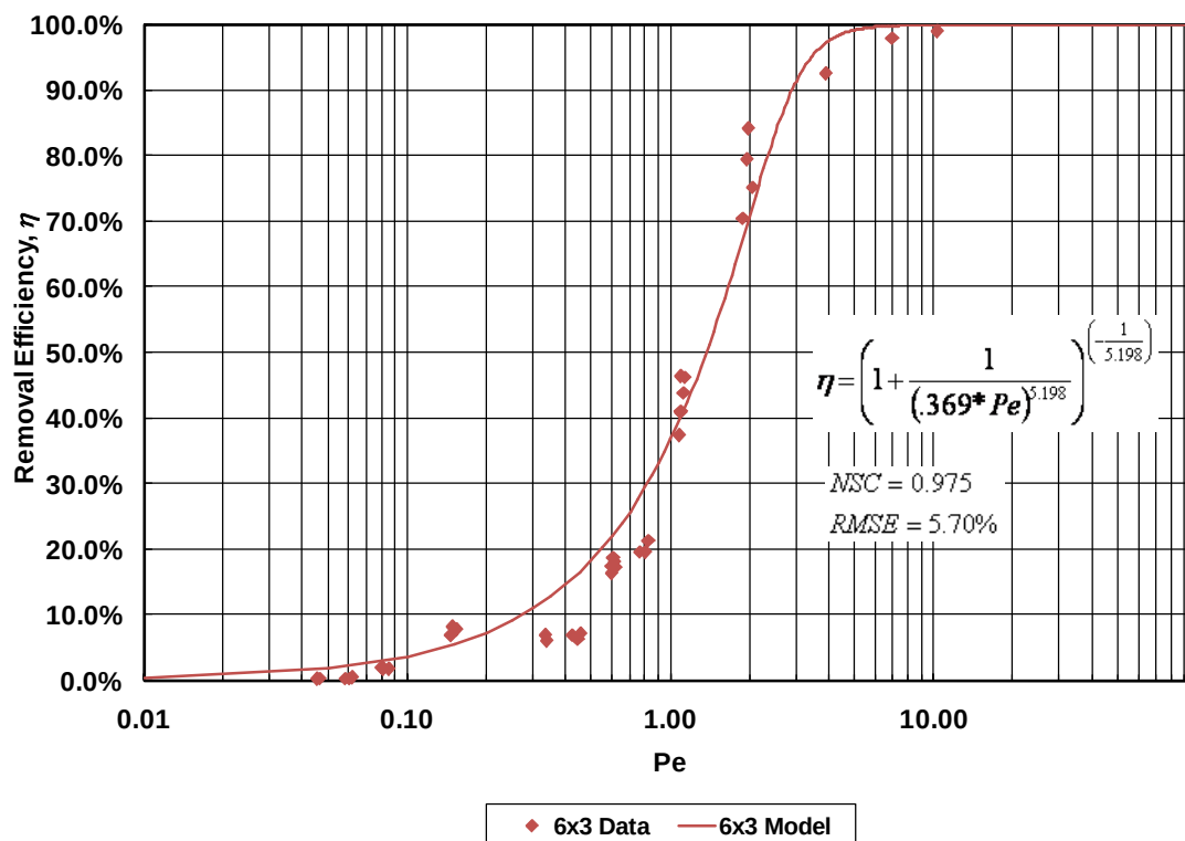
Figure G.4. 6×3 ft Standard Sumps Removal Efficiency Results
