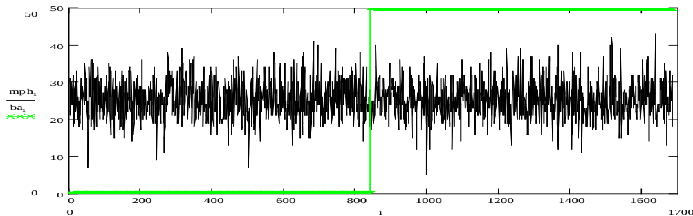
Figure 4.1. Sequential Plot of Speed Measurements from Colorado Site (‘After’ Period Begins at Position = 839)
