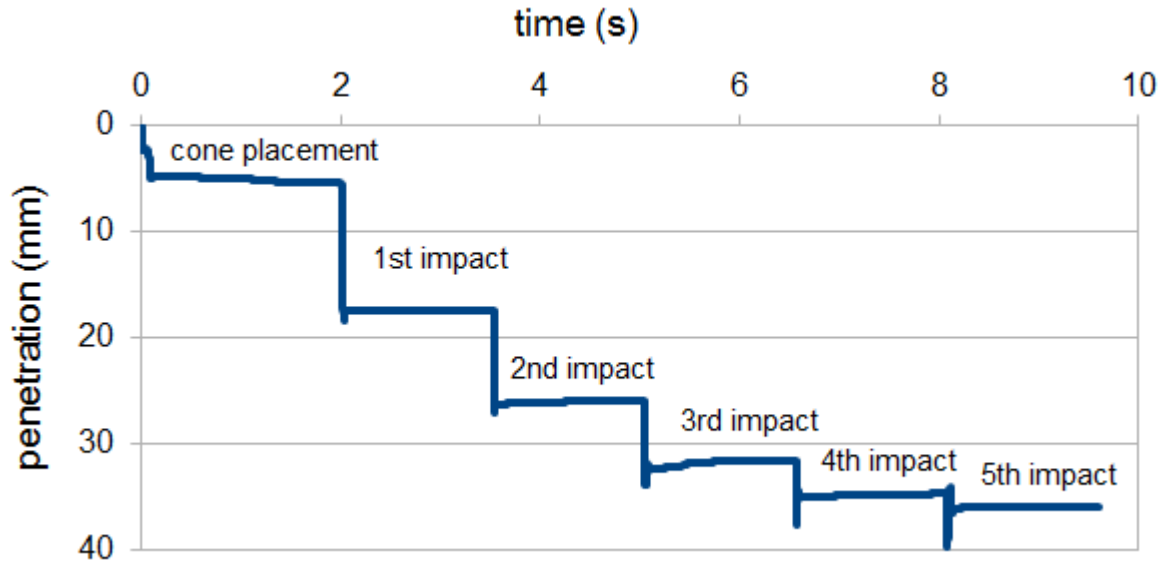
Figure 61: Data from a DCP model test using Moisture Model III and the DEM mixture representing the Class 5 mixture described in Section 3.1. DCP penetration during including initial placement and consecutive hammer blows for a system with equivalent model suction of 114 kPa, and an interparticle friction coefficient of 0.2.
