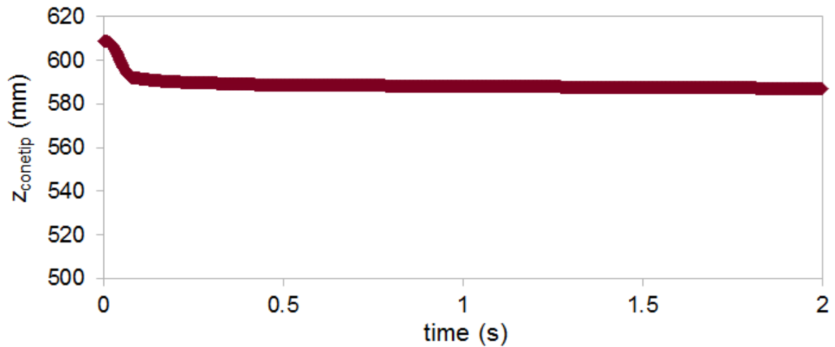
Figure 28: Data from initial placement of the DCP rod/cone assembly using Moisture Model I and the DEM mixture representing the Class 5 mixture described in Chapter 3. Position of cone-tip (base of cone-rod assembly) is plotted as a function of time during initial placement for a system with 6% gravimetric moisture content and surface tension \gamma^* .
