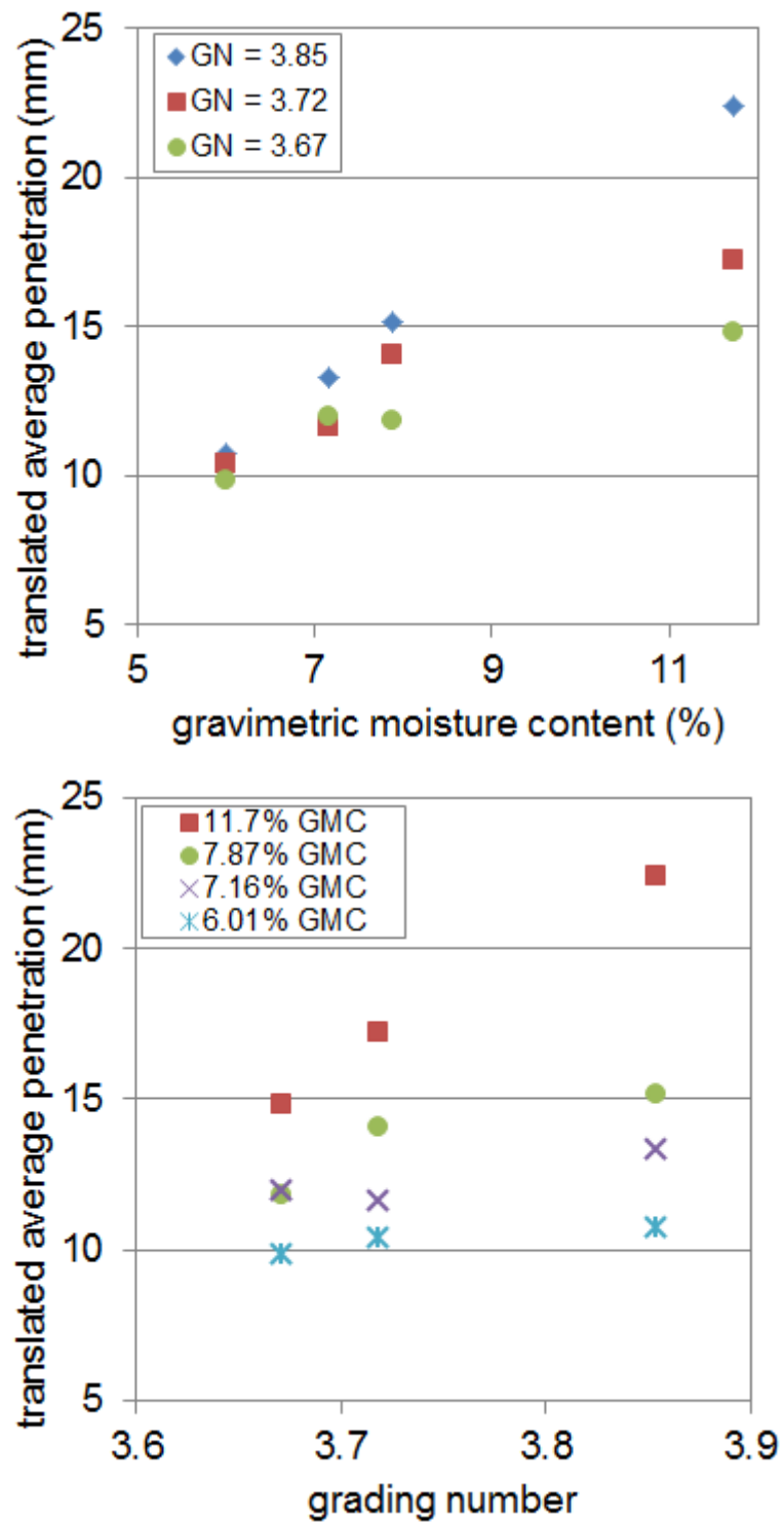
Figure 69: DCP model test results in terms of all translated parameters according to Equations 32, 33, and 35.
