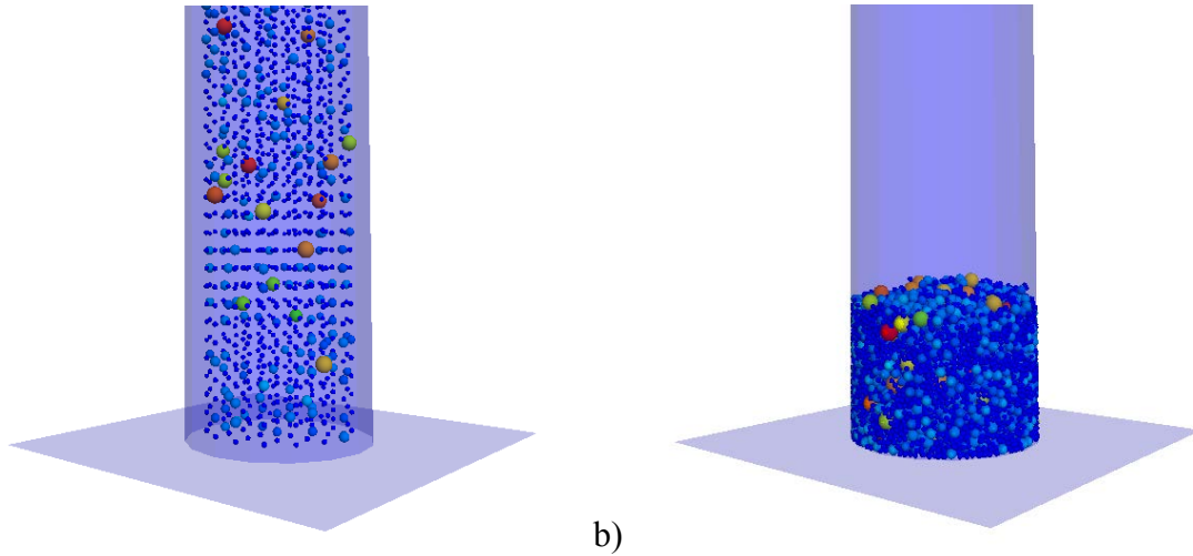
Figure 70: Screenshots of the initialization stage of the LWD test in PFC3D: (a) A suspended arrangement of spheres is dropped into a cylinder. (b) This method of initialization method results in a non-segregated mixture.
