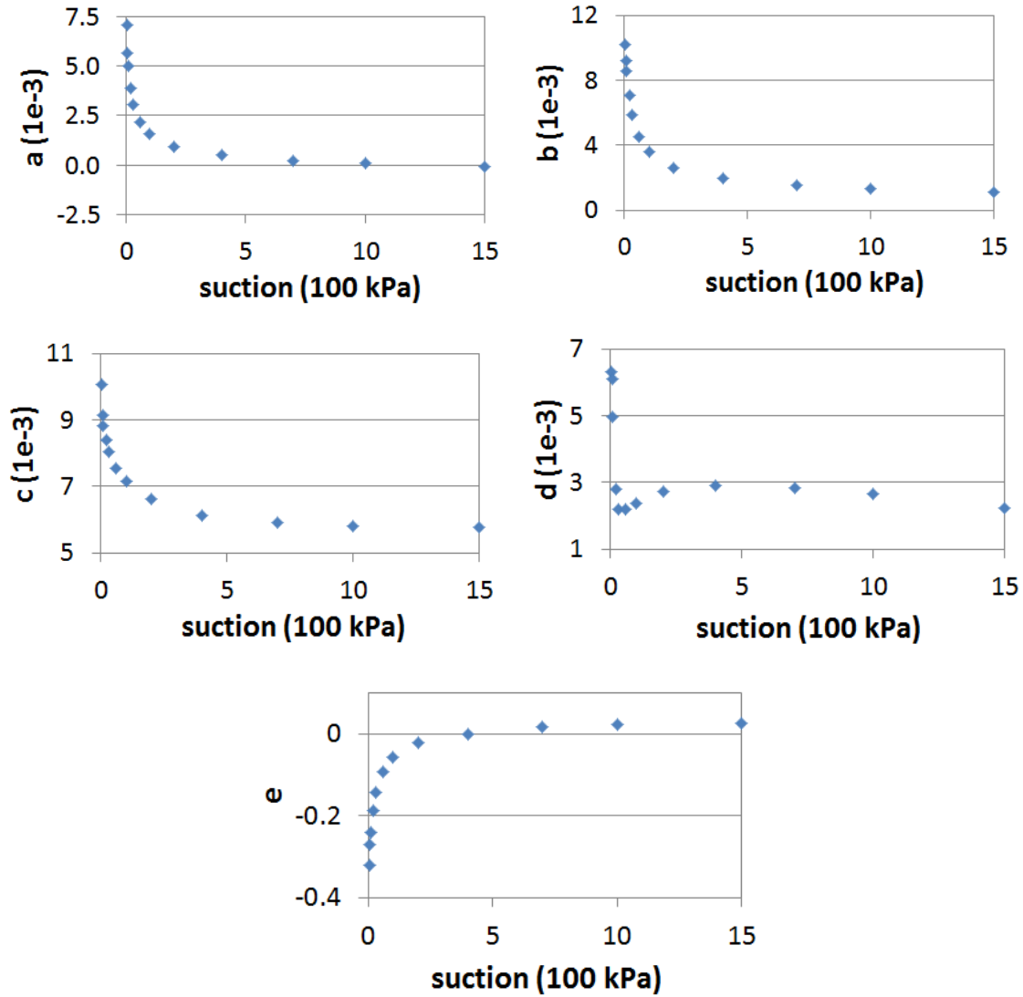
Figure 40: Empirical fit coefficients a , b , c , d and e for Equation 15 described in detail by Gupta and Larson [33].
