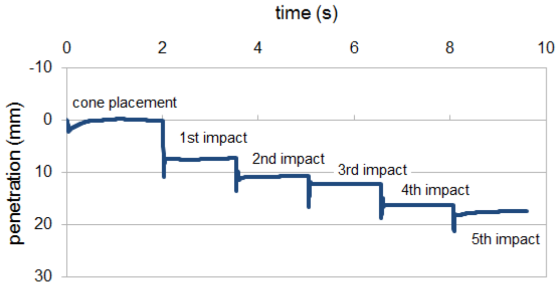
Figure 52: Data from a DCP model test using Moisture Model II and the DEM mixture representing the Class 5 mixture described in Section 3.1. Temporal dependence of the cone penetration during including initial placement and consecutive hammer blows for a system with equivalent model suction of 114 kPa.
