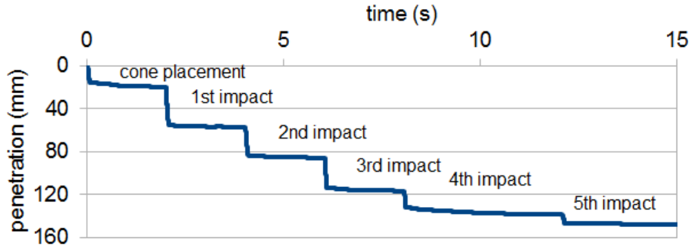
Figure 29: Data from model DCP test using Moisture Model I and the DEM mixture representing the Class 5 mixture described in Chapter 3. DCP penetration is plotted as a function of time during including initial placement and consecutive hammer blows for a system with 6% gravimetric moisture content and surface tension \gamma^* .
