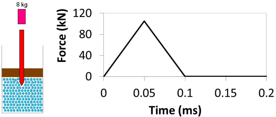
Figure 16: (Left) Sketch of the DEM simulation procedure of the hammer drop phase of the DCP test; (Right) Loading history of the model DCP test, representing the falling hammer.
