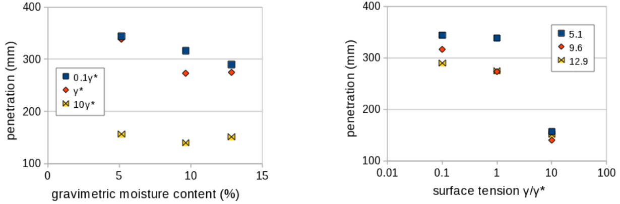
Figure 33: Data from Figs. 31 and 32. Penetration during 1st hammer impact plotted as a function of (left) gravimetric moisture content for surface tensions 0.1 \gamma^* , \gamma^* and 10 \gamma^* ; and (right) as a function of surface tension, for gravimetric moisture contents 5.1%, 9.6% and 12.9%.
