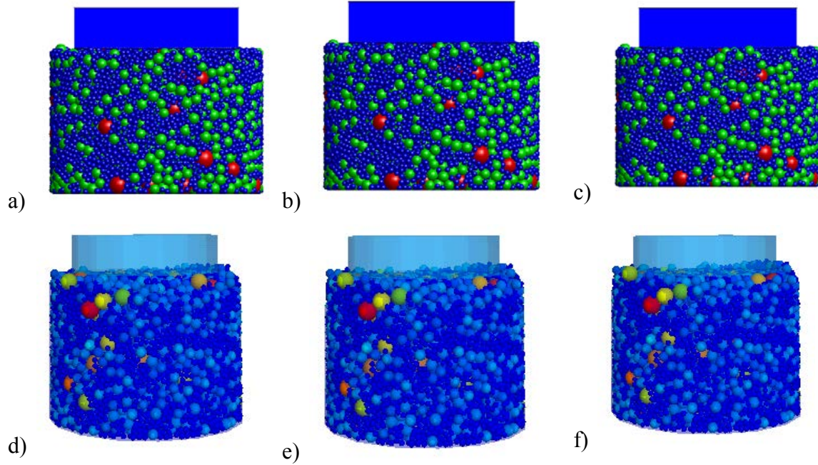
Figure 87: Screenshots of a granular mixture with 8% gravimetric moisture content during the LWD test using the DEMP-3D (a-c) and PFC3D (d-f) codes: after the 1st impact (a,d), after the 3rd impact (b,e), and after the 5th impact (c,f).
