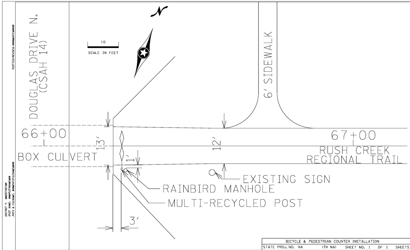
Figure 3-3 Site Plans for Rush Creek Trail Bicycle and Pedestrian Traffic Monitoring Station (inductive loop and passive infrared counter)
