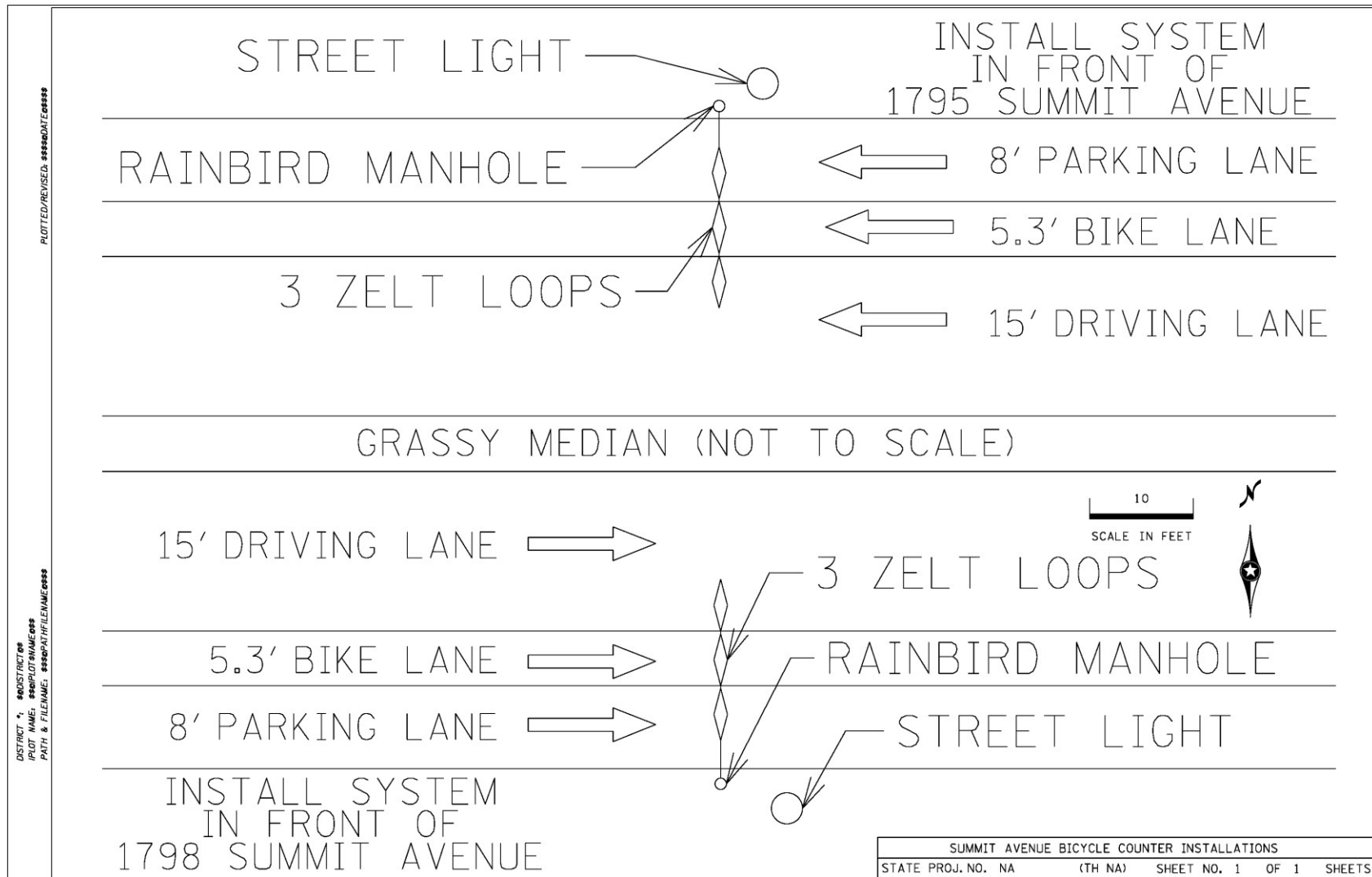
Figure 3-2 Site Plans for Summit Avenue Bicycle Traffic Monitoring Station (inductive loop counter)
