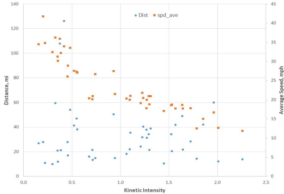
Figure 3.3 Winter drive cycle distance and average speed versus KI for ¾-ton pickup trucks
