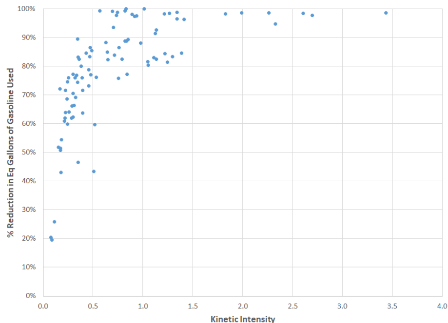
Figure 3.6 ¾ ton pickup trucks fall reduction in equivalent gallons of gasoline used
