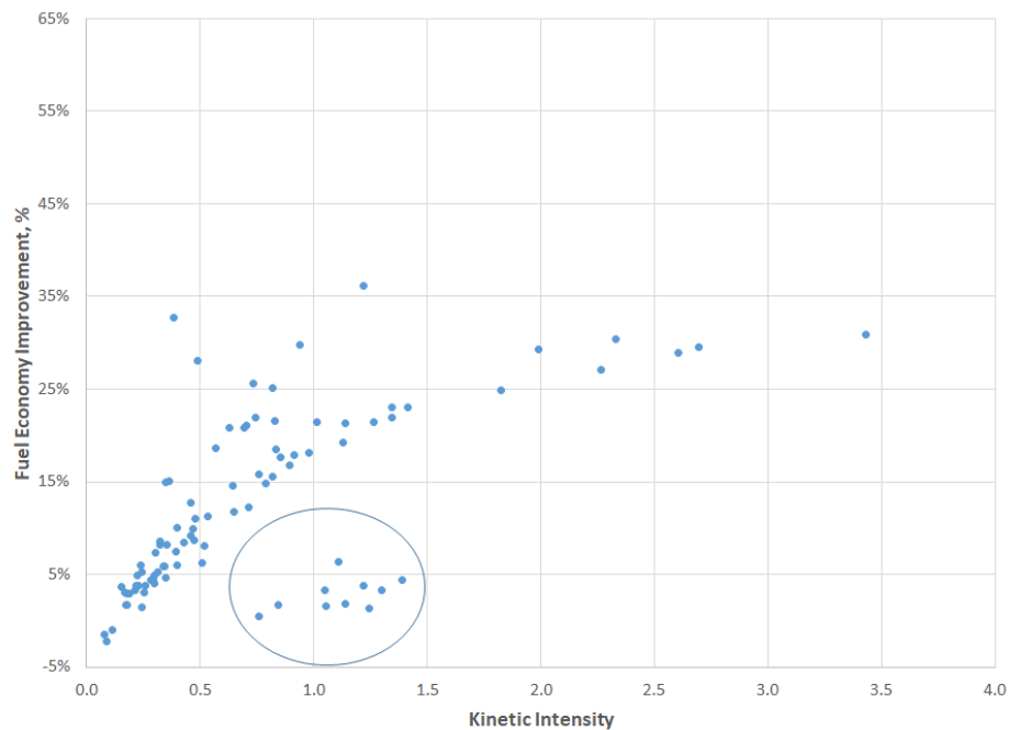
Figure 3.4 ¾ ton pickup truck fall fuel economy improvement versus kinetic intensity. Circled region are data points from a single vehicle with anomalous behavior
