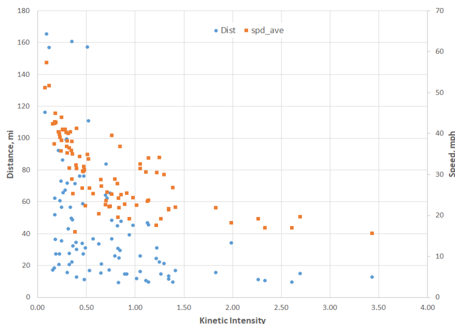
Figure 3.2 Fall drive cycle distance (circles) and average speed (squares) versus KI for \frac{3}{4} -ton pickup trucks
