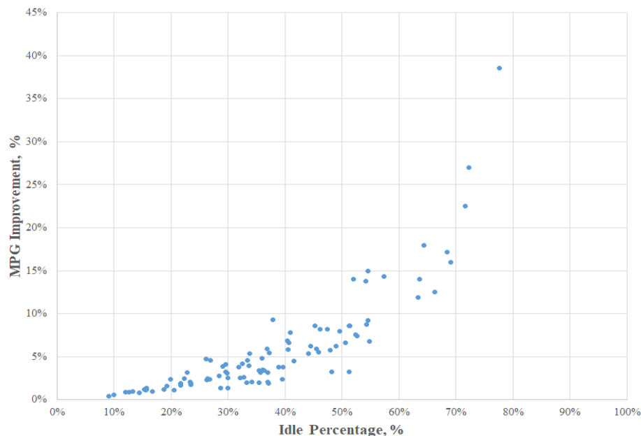
Figure 3.1 Modeled improvement in fuel economy with idling periods removed for the ¾ ton pickup trucks
