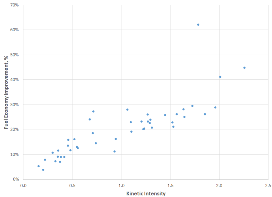
Figure 3.5 ¾-ton pickup truck winter fuel economy improvement versus kinetic intensity
