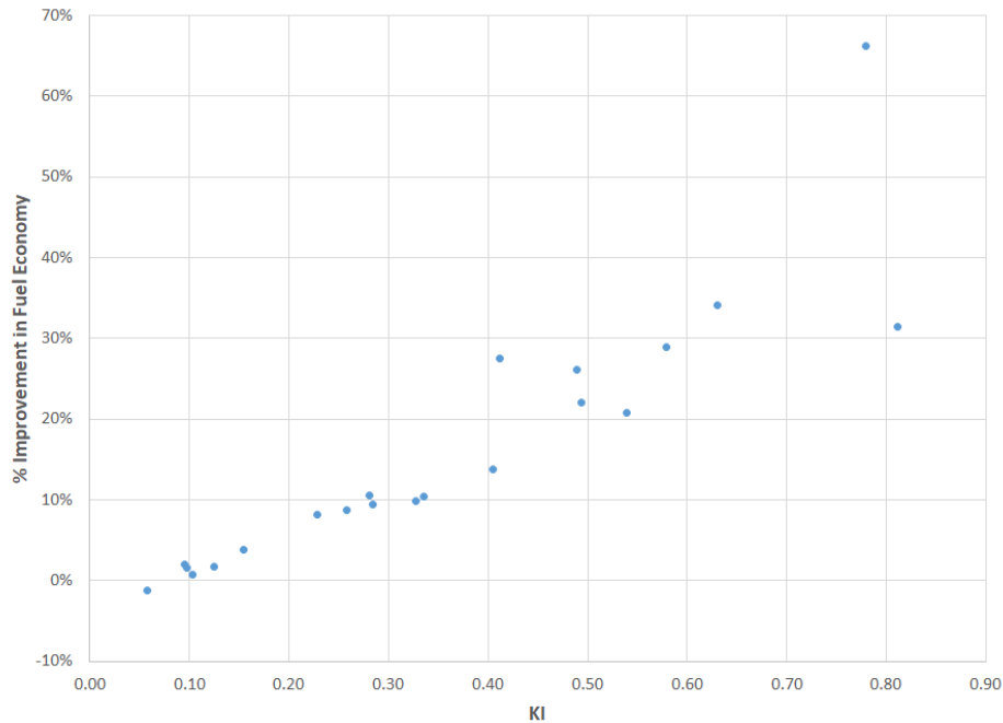
Figure 3.7 ½ ton PHEV pickup truck fuel economy improvement over conventional baseline powertrain versus KI
