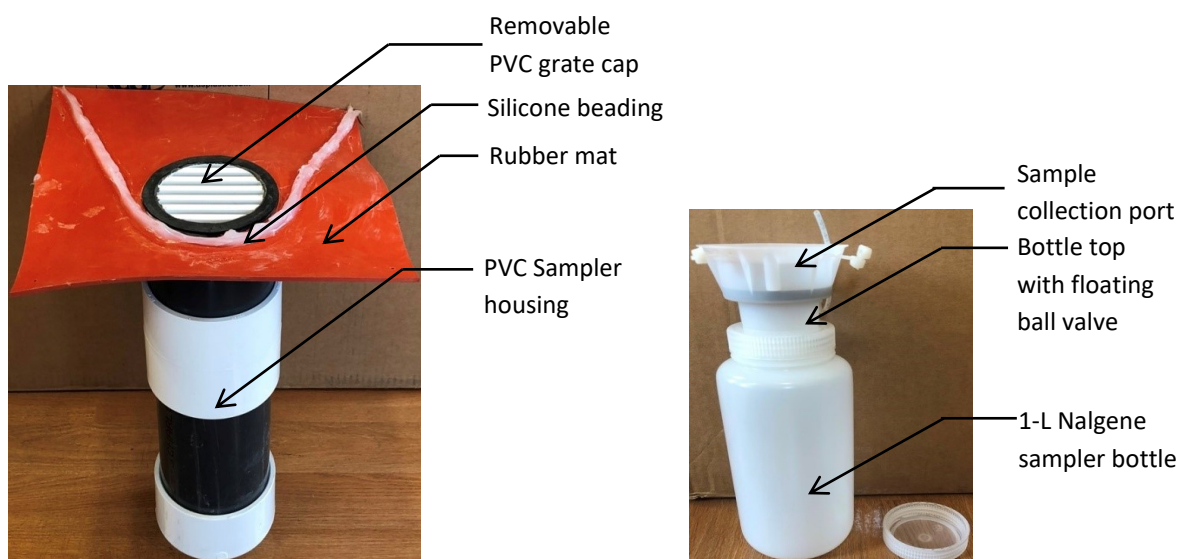
Figure 3.1. Photographs of the runoff sampler (left) and the Nalgene sampler bottle (right) used to collect runoff samples at the low-volume road sampling sites.
