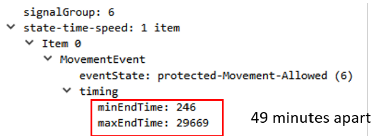
Figure 2.10: An excerpt of SPaT collected at Meadow
