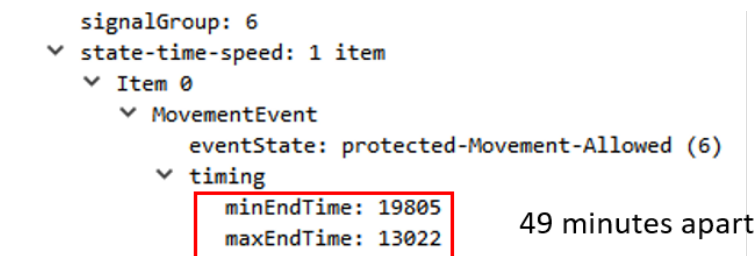
Figure 2.11: An excerpt of SPaT collected at Meadow
