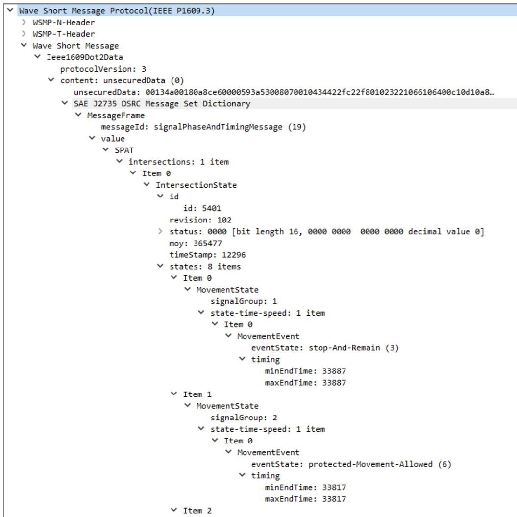
Figure 2.3: An example of a decoded SPaT message
