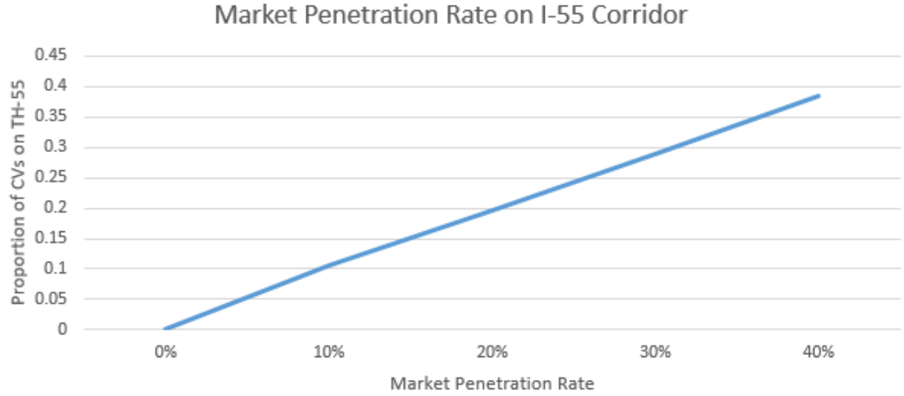
Figure 6.5: Observed TH-55 Market Penetration Rate
