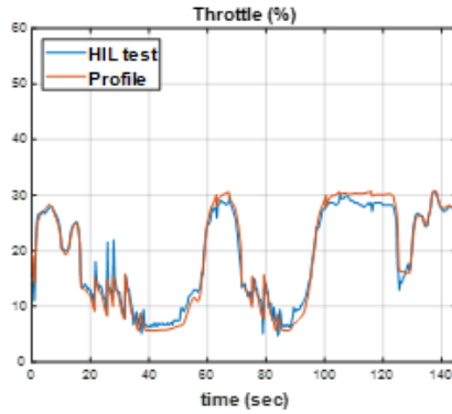
(c) Throttle (%)
