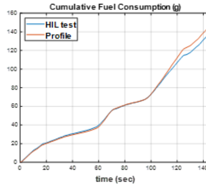
(f) Cumulative Fuel Consumption (g)
