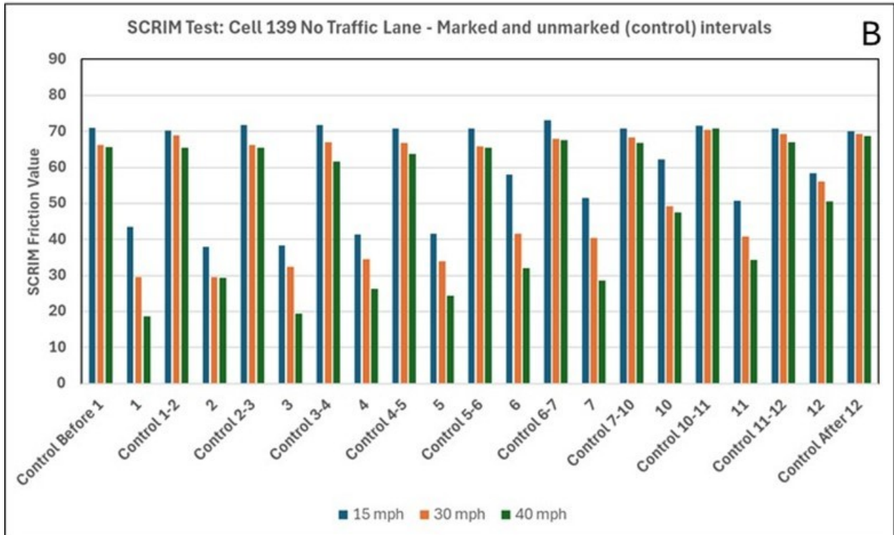
Figure 6.17 SCRIM friction numbers for Cell 139 relative to the unmarked intervals immediately before, between, and after the pavement markings: Traffic Lane (A) and No Traffic Lane (B)
