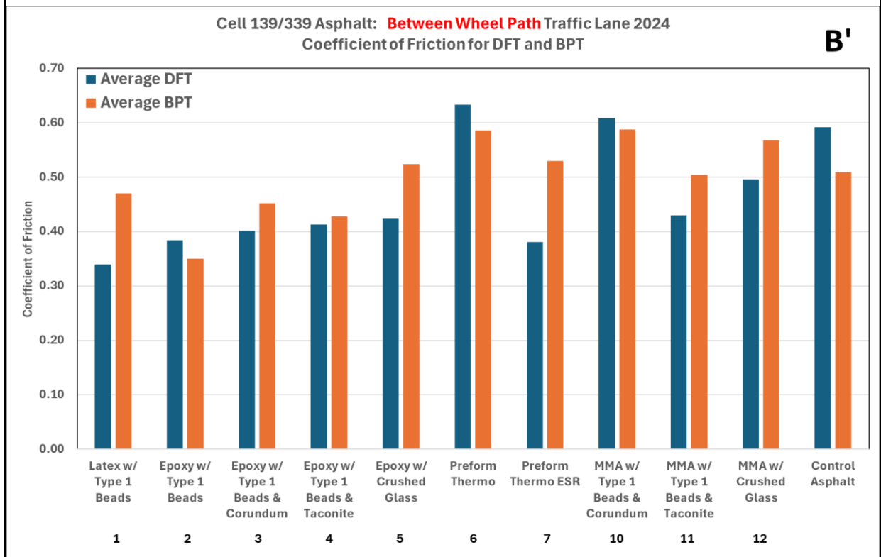
Figure 6.12 DFT and BPT measurements BWP of Cell 139/339 markings and control (B and B')
