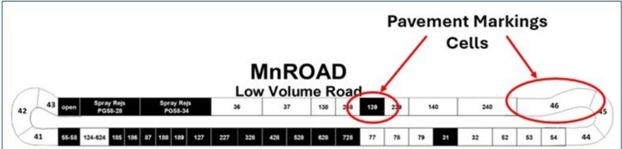
Figure 5.1 MnROAD Low Volume Road cells for pavement markings testing (Cell 46 concrete; Cell 139/339 asphalt)
