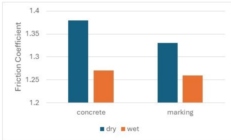
Figure 4.11 T2Go test results
