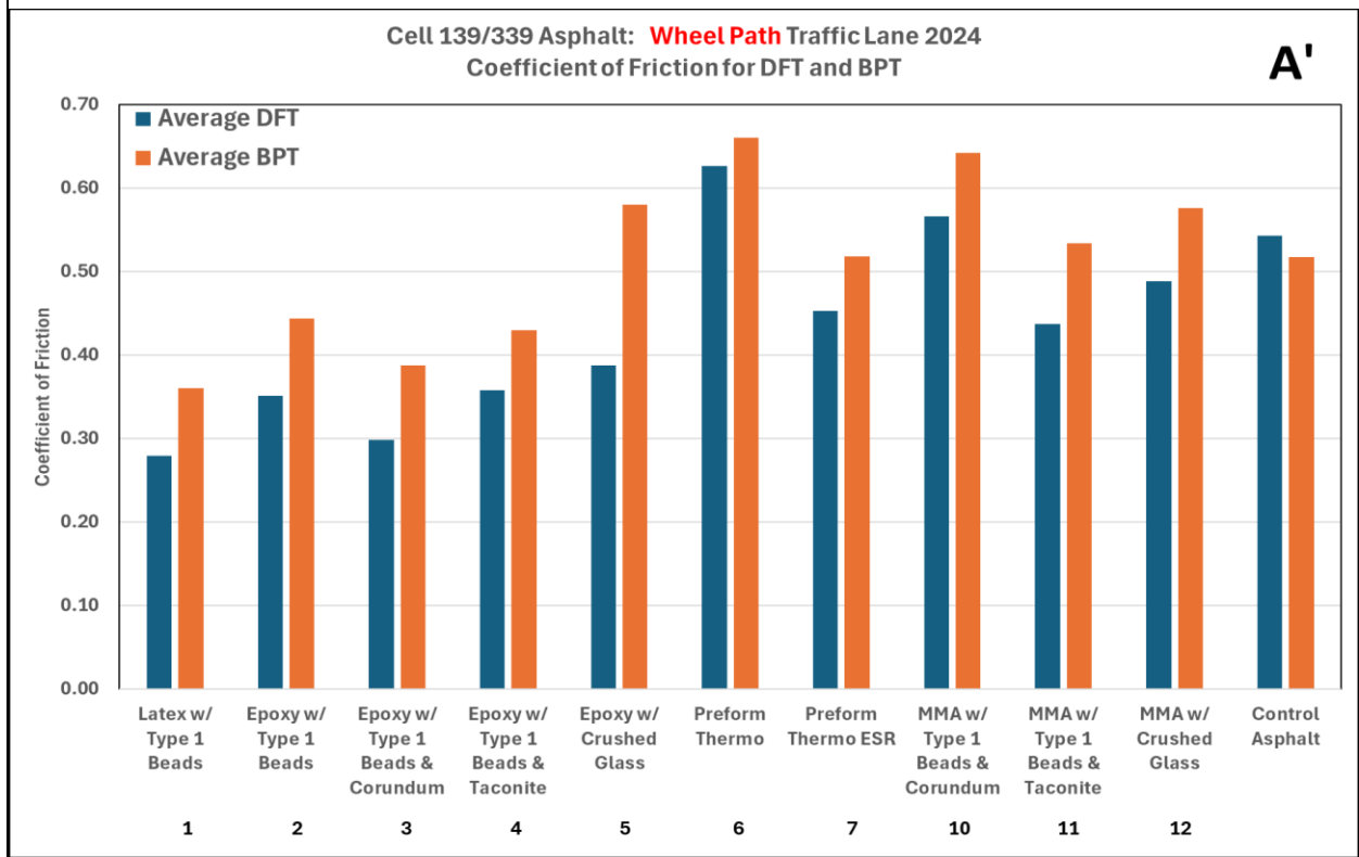
Figure 6.11 DFT and BPT measurements in WP of Cell 139/339 markings and control (A and A')
