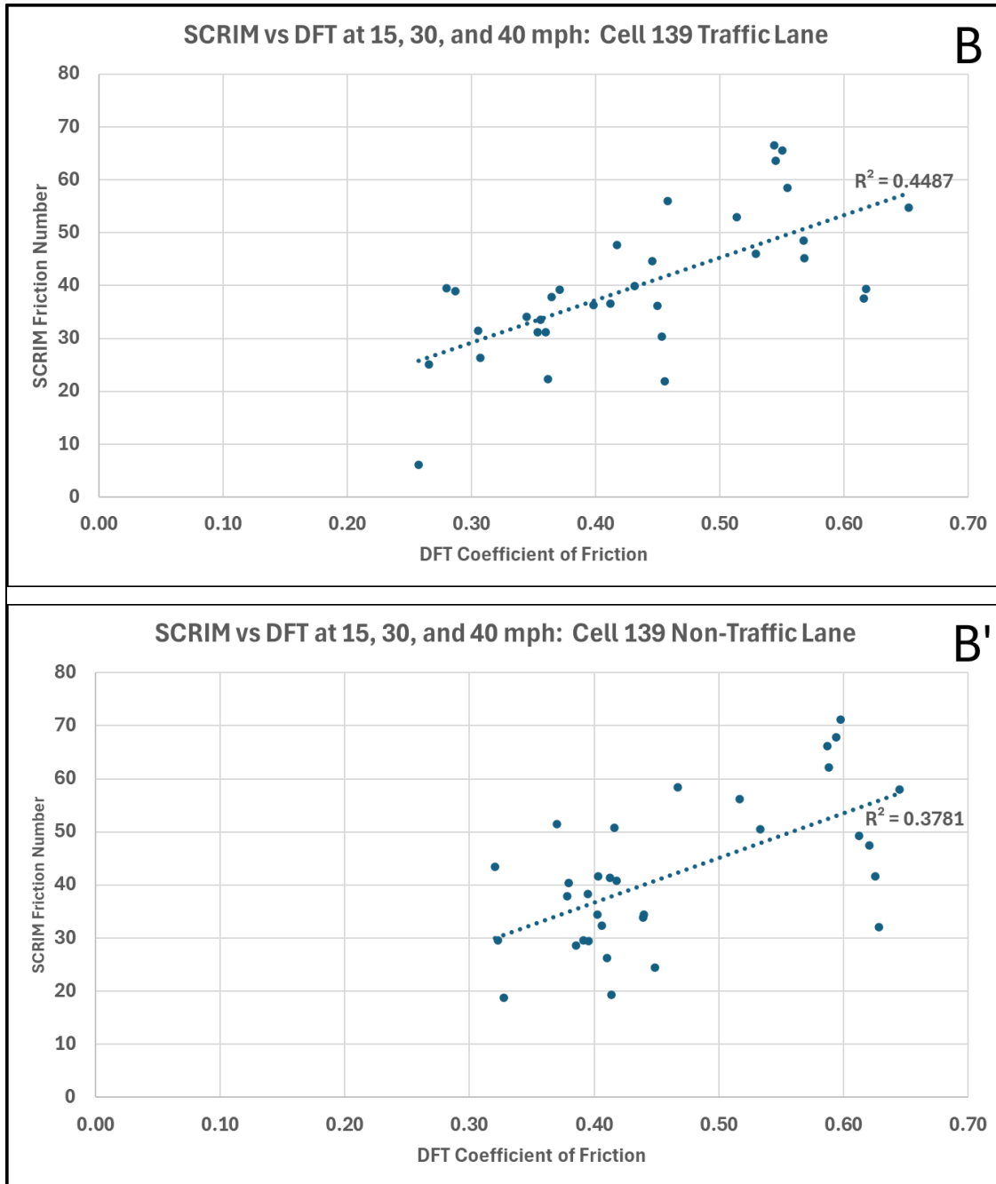
Figure 6.19 Scatter plots of SCRIM vs DFT friction values and linear regressions for Cell 139 Traffic Lane (B) and Non-Traffic Lane (B').
