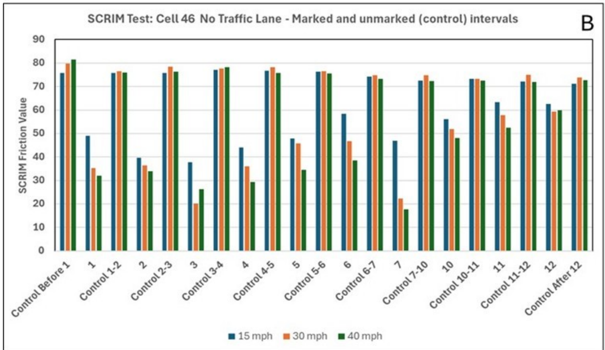
Figure 6.16 SCRIM friction numbers for Cell 46 relative to the unmarked intervals immediately before, between, and after the pavement markings: Traffic Lane (A) and No Traffic Lane (B)
