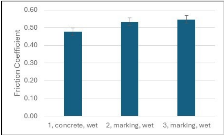
Figure 4.9 British pendulum test results
