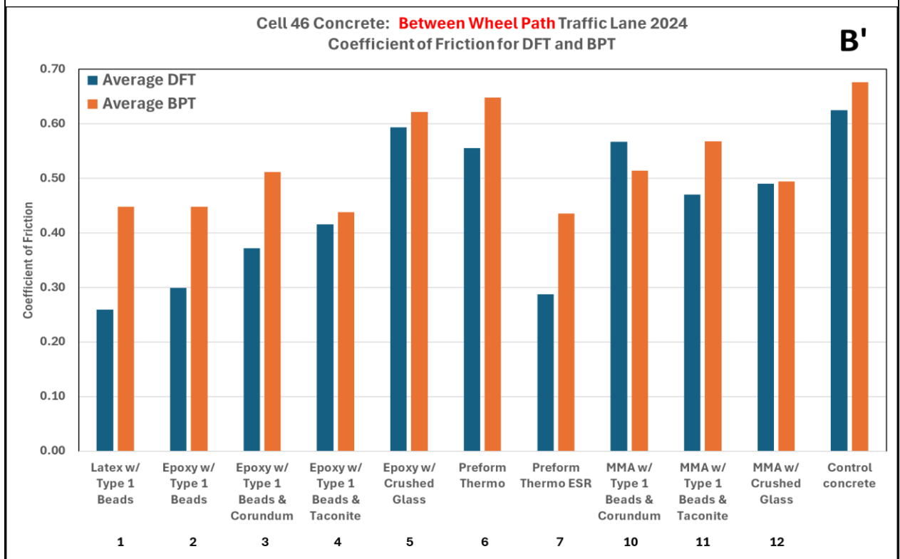
Figure 6.10 DFT and BPT measurements BWP of Cell 46 markings and control (B and B')
