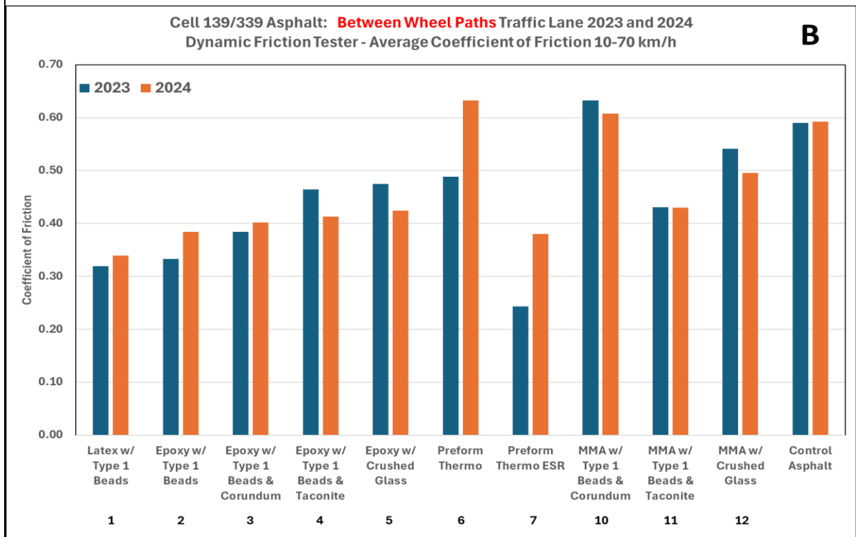
Figure 6.6 Average coefficient of friction measured by the DFT for Cell 139 markings: WP (A) and BWP (B)
