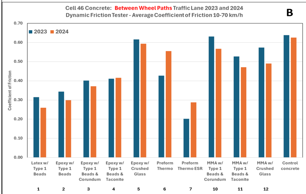
Figure 6.5 Average coefficient of friction measured by the DFT for Cell 46 markings: WP (A) and BWP (B)
