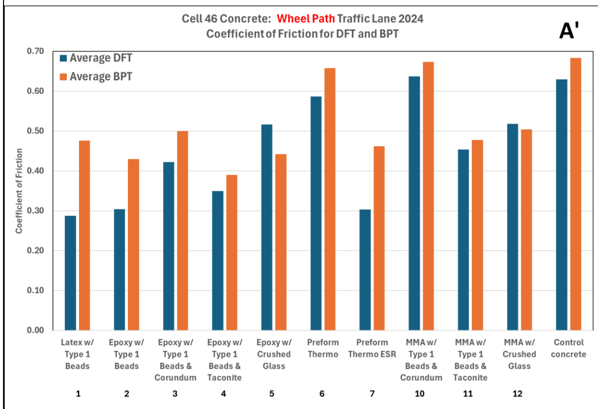
Figure 6.9 DFT and BPT measurements of WP of Cell 46 markings and control (A and A')
