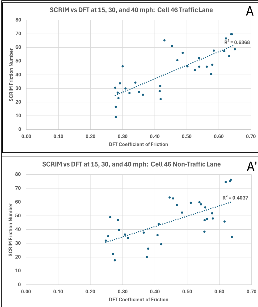
Figure 6.18 Scatter plots of SCRIM vs DFT friction values and linear regressions for Cell 46 Traffic Lane (A) and Non-Traffic Lane (A')
