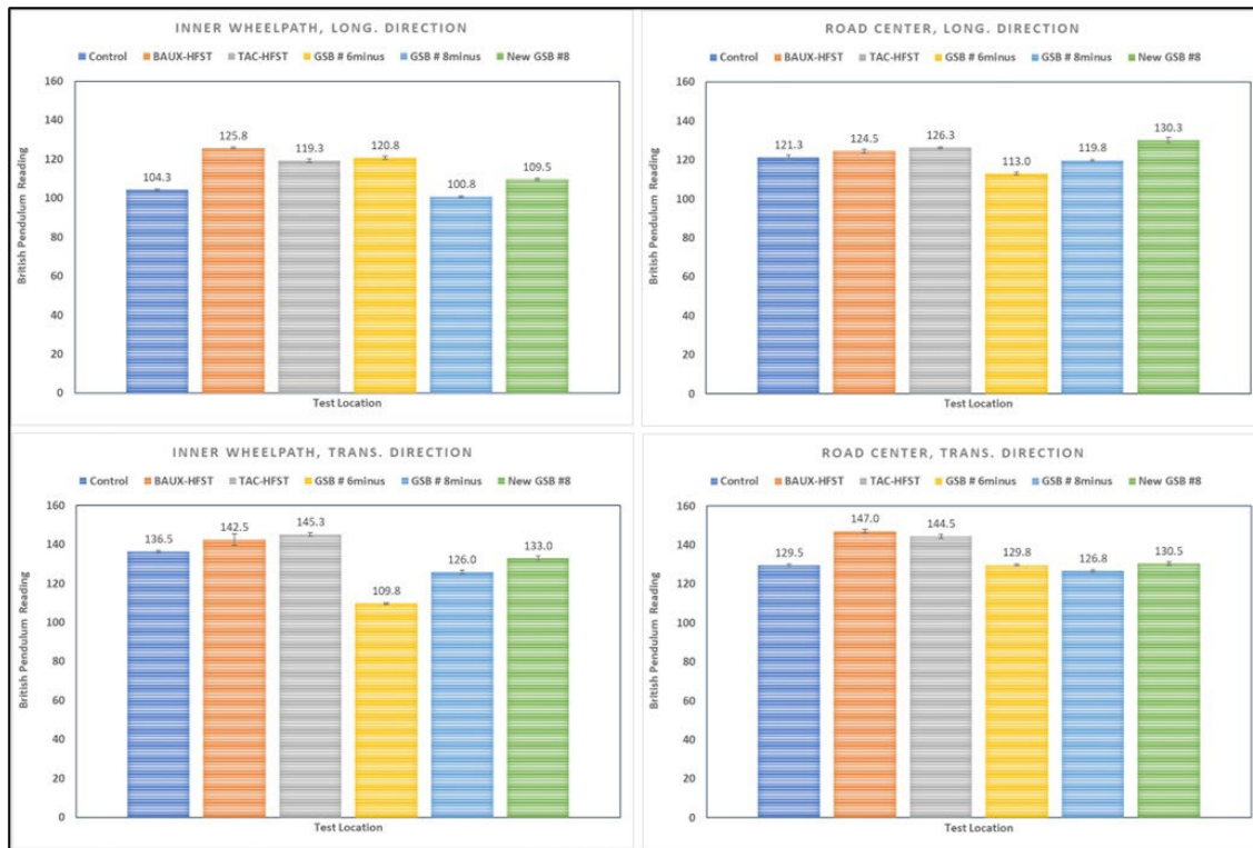
Figure 7.39. British Pendulum test results: April 30, 2024 (charts and data table)
