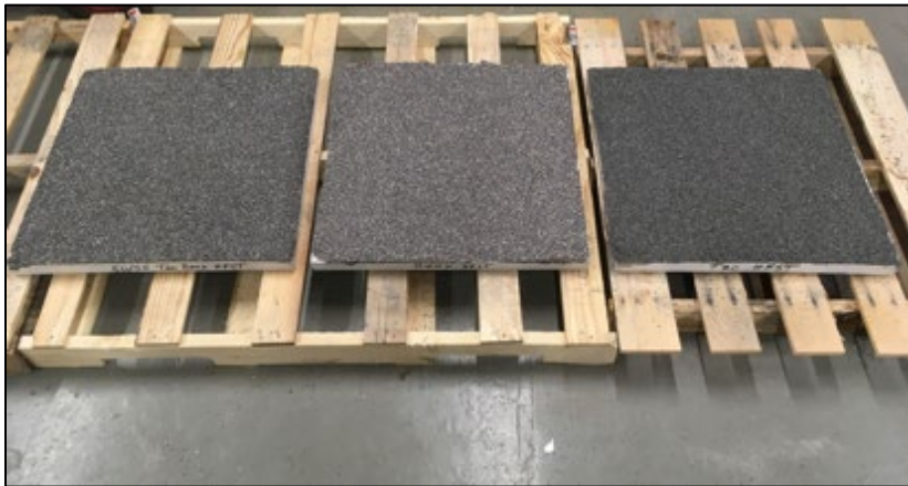
Figure 4.6. HFST specimen slabs for Circular Track Polishing Machine (CTPM) testing at the North Central Superpave Center - 50:50 blend of taconite and calcined bauxite (left); 100% calcined bauxite (center); and 100% taconite (right)
