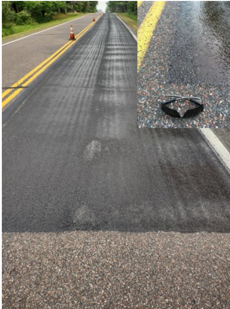
Figure 5.6. Completed Friction Seal test section and close-up image (inset)
